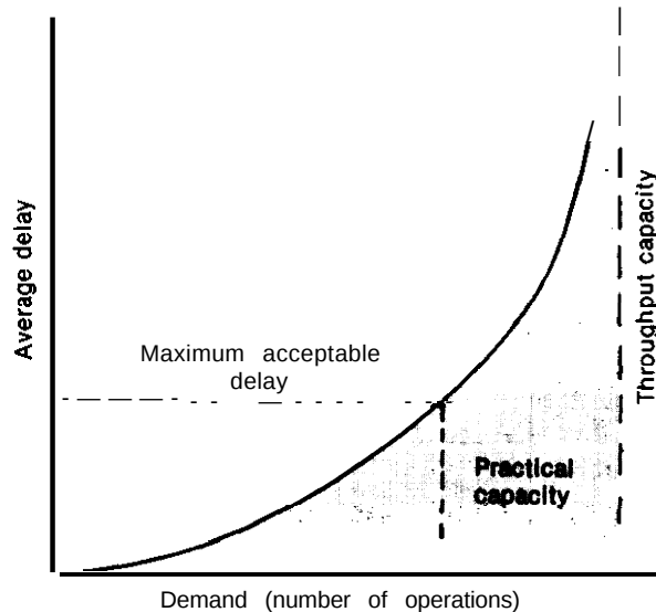
Figure 5.—Relationship Between Throughput and Practical Capacity
