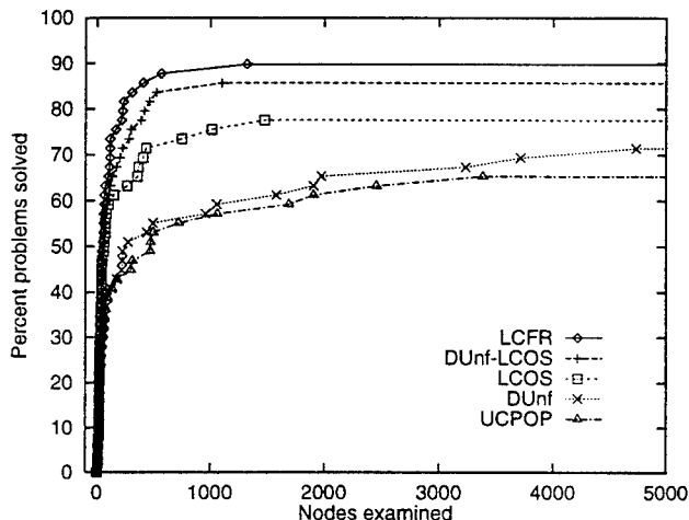
Figure 2: Comparison of planner search spaces
