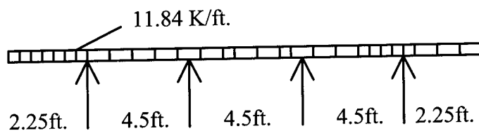
Longitudinal View of the 3 span pile cap
