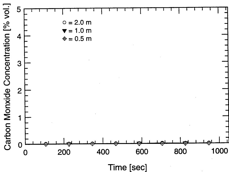
Gas Tree #2
