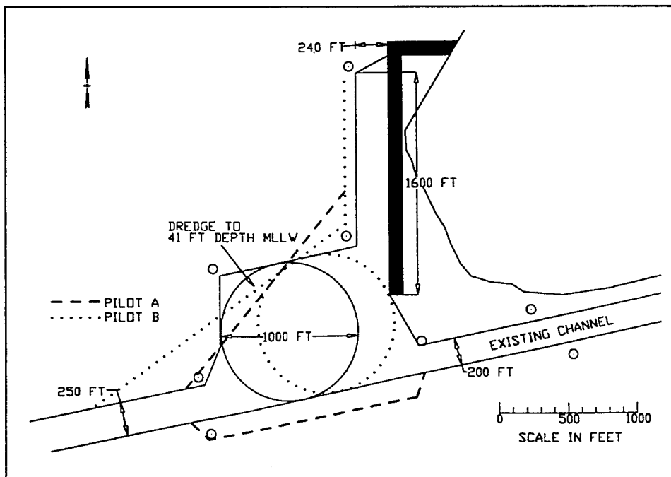
Figure 18. Pilot suggestions for Plan 2 turning basin configuration
