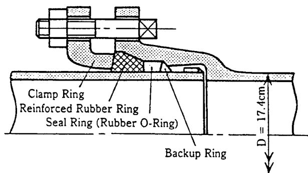
a. Cross Section of TM Joint
