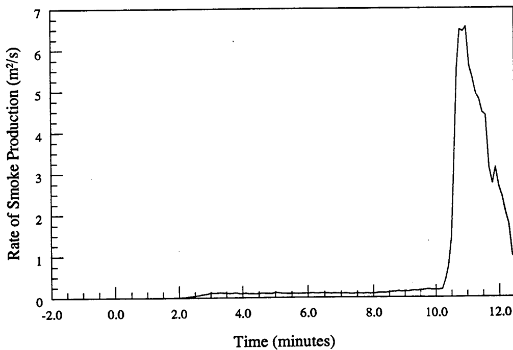
Figure 9.b - Material # 9 - Smoke production vs. time
