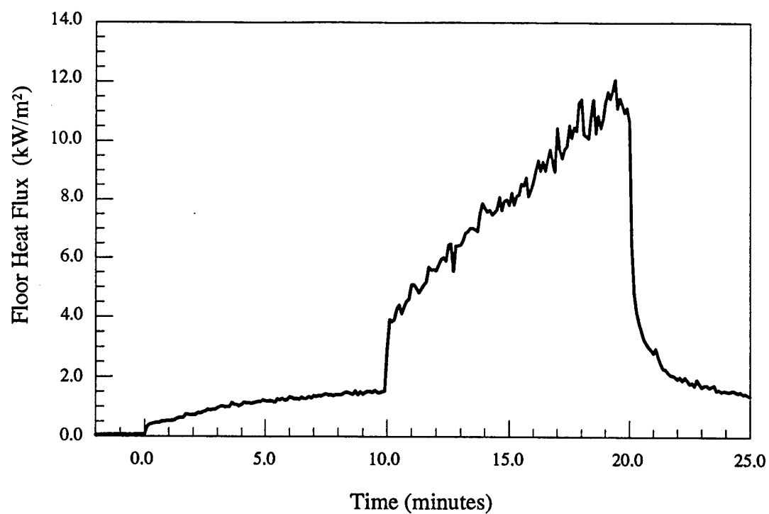
Figure 6.c - Material # 6 - Floor heat flux vs. time
