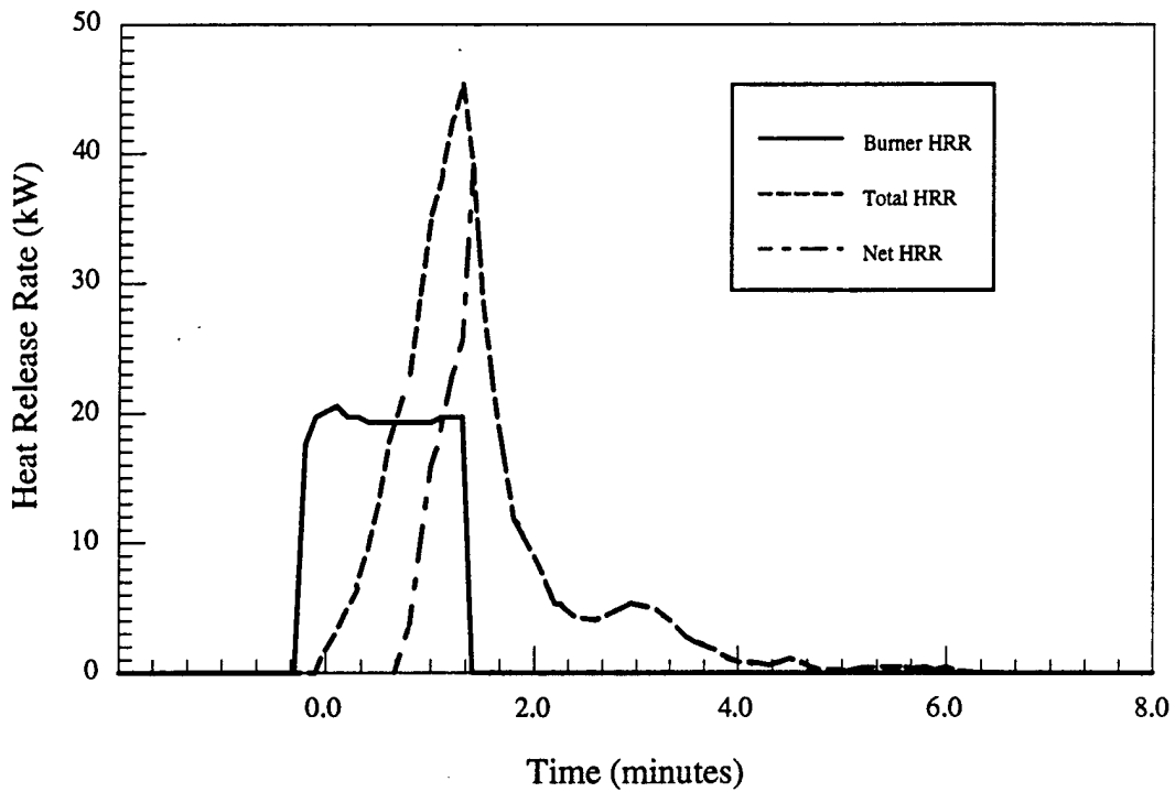
Figure 8.a - Material # 5 - Double chair - Heat release rate vs. time
