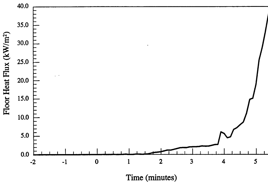
Figure 4.c - Material # 4 - Floor heat flux vs. time
