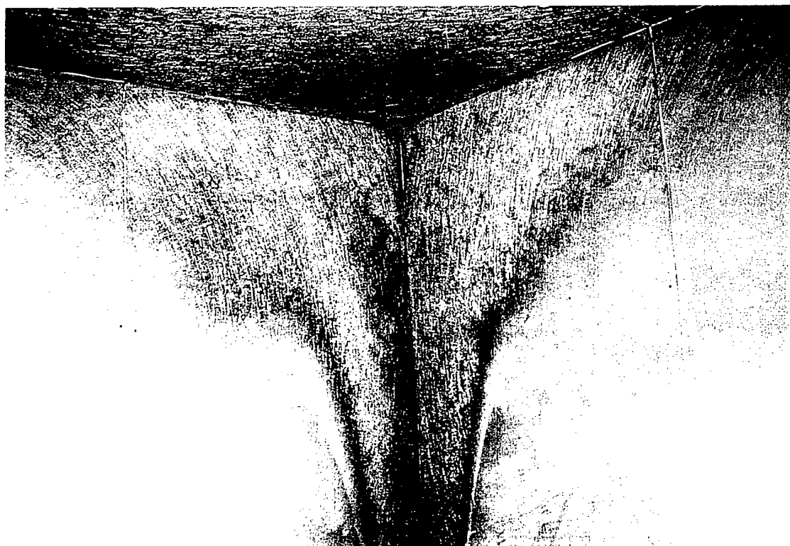
Figure 32. Material No. 8 After Termination of the Room/Corner Test.
