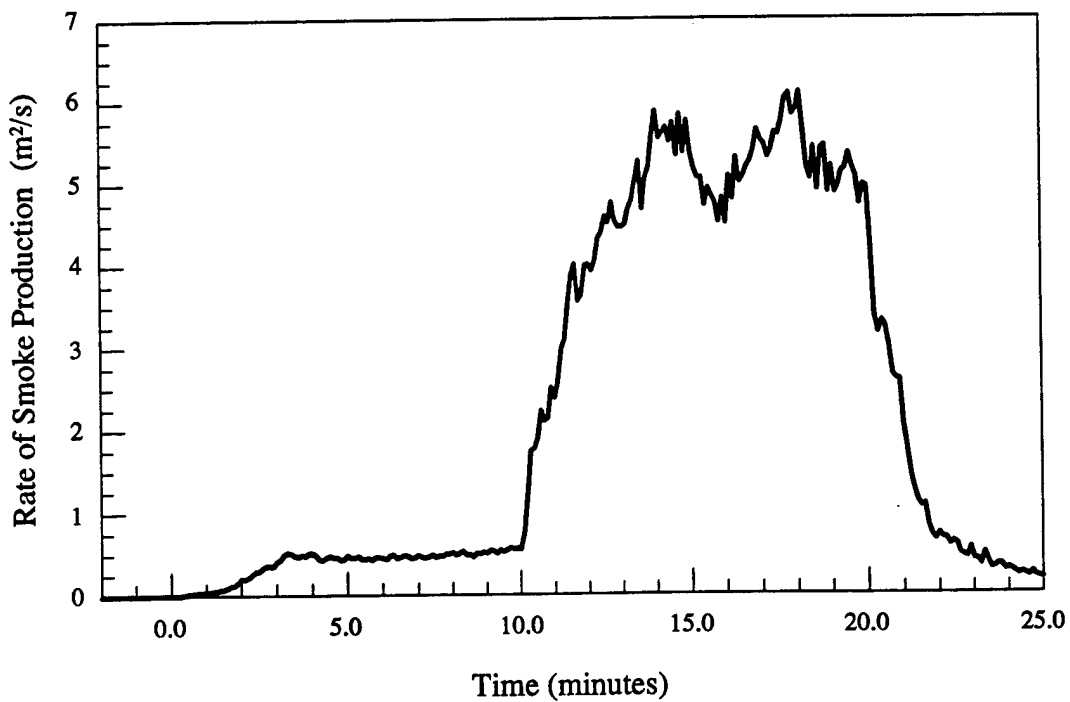
Figure 6.b - Material # 6 - Smoke production rate vs. time
