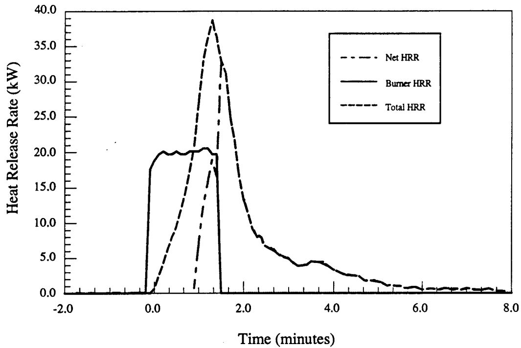
Figure 1.a - Steel - Heat release rate vs. time
