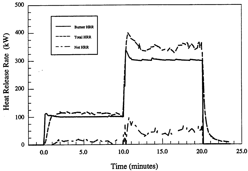
Figure 2.a - Material # 2 - Heat release rate vs. time
