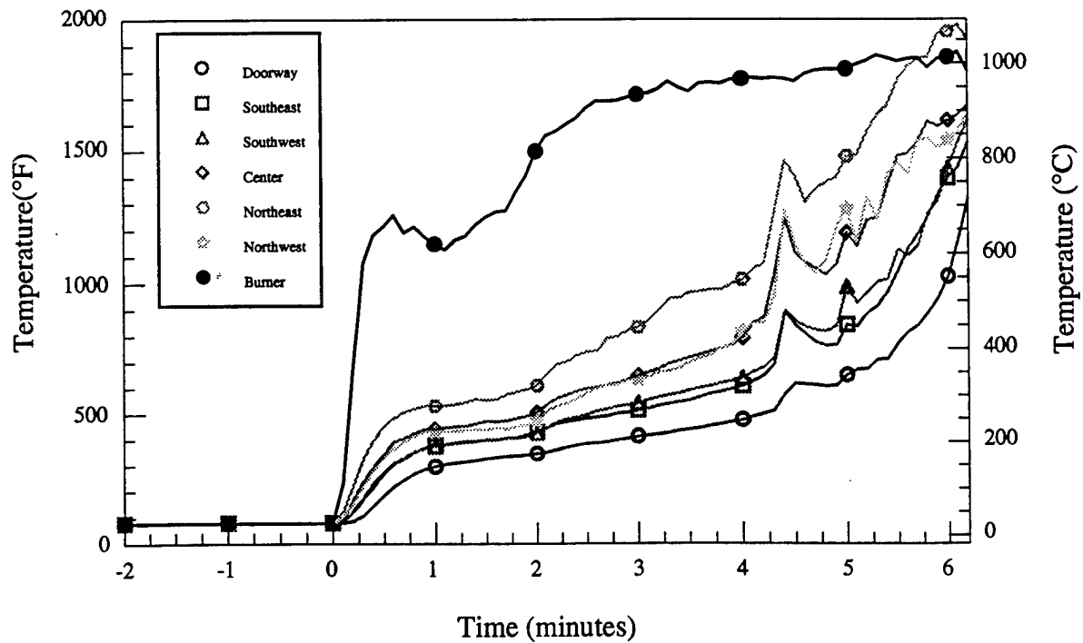
Figure A.3.d - Material # 3 - Room temperatures vs. time
