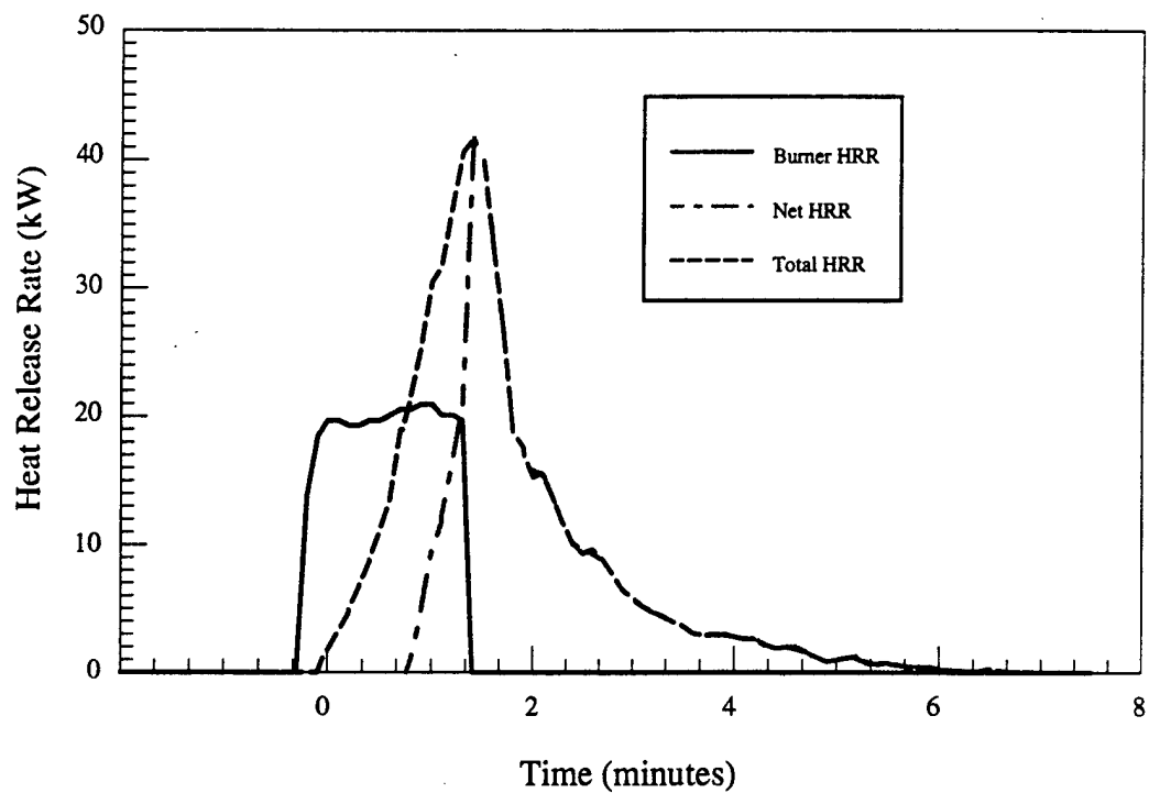
Figure 2.a - Steel - Double chair - Heat release rate vs. time
