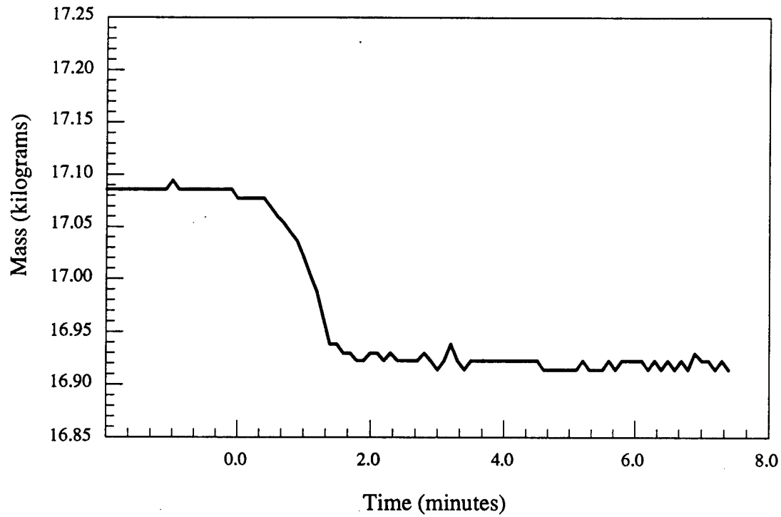
Figure 6.c - Material # 4 - Single chair - Mass vs. time
