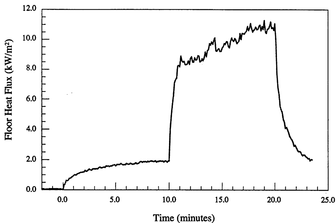
Figure 2.c - Material # 2 - Floor heat flux vs. time
