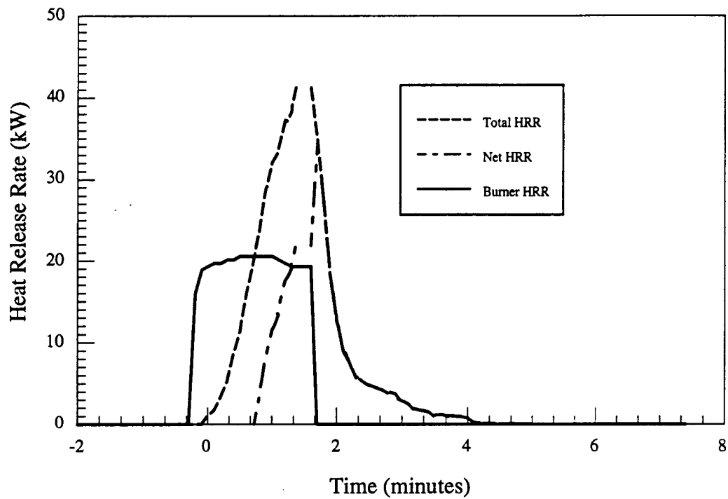
Figure 7.a - Material # 5 - Single chair - Heat release rate vs. time
