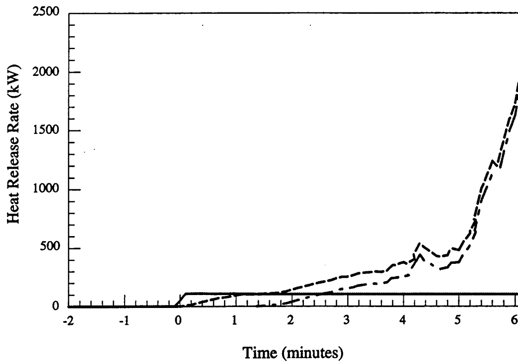
Figure 3.a - Material # 3 - Heat release rate vs. time
