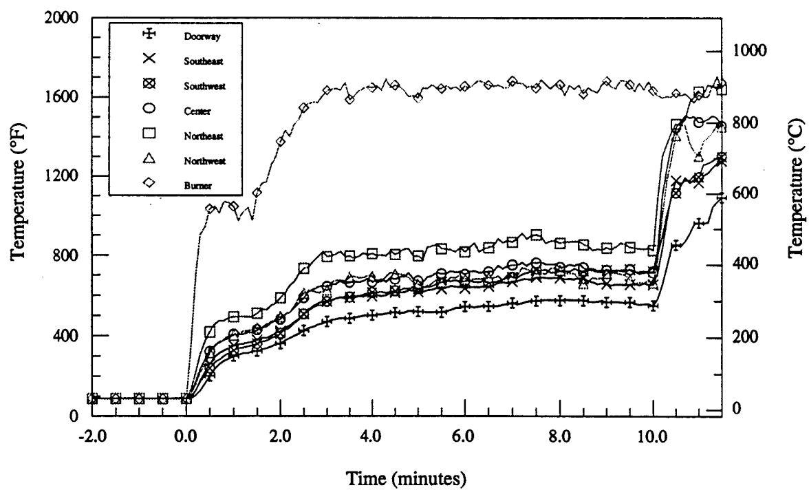
Figure 9.d - Material # 9 - Room temperatures vs. time
