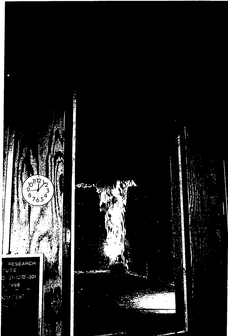
Figure 11. Material No. 3 Just Prior to Flashover.
