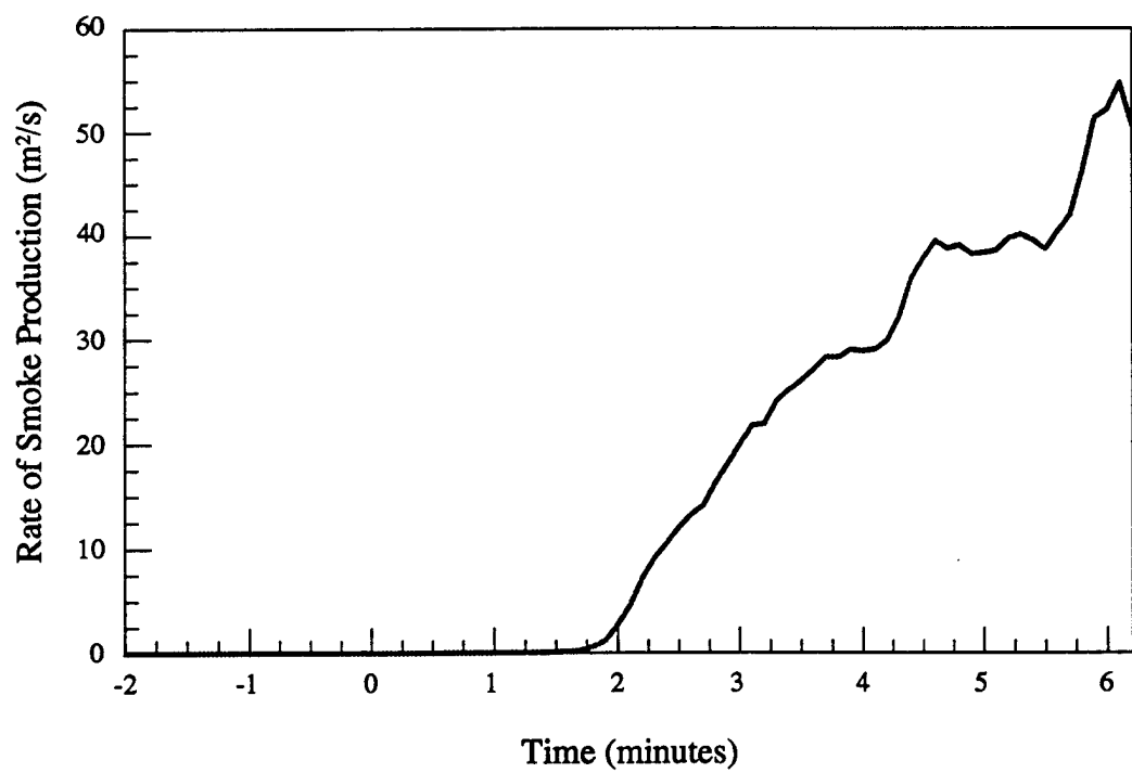
Figure 3.b - Material # 3 - Smoke production rate vs. time
