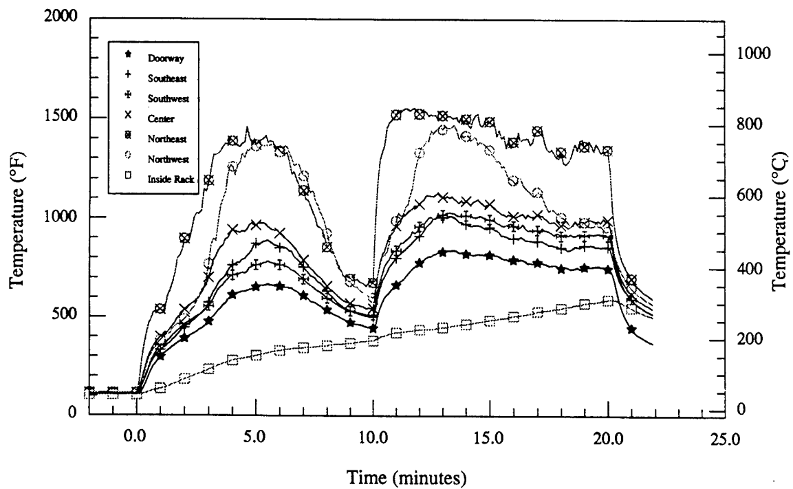
Figure 11.d - Material # 3 - Luggage rack - Room temperatures vs. time
