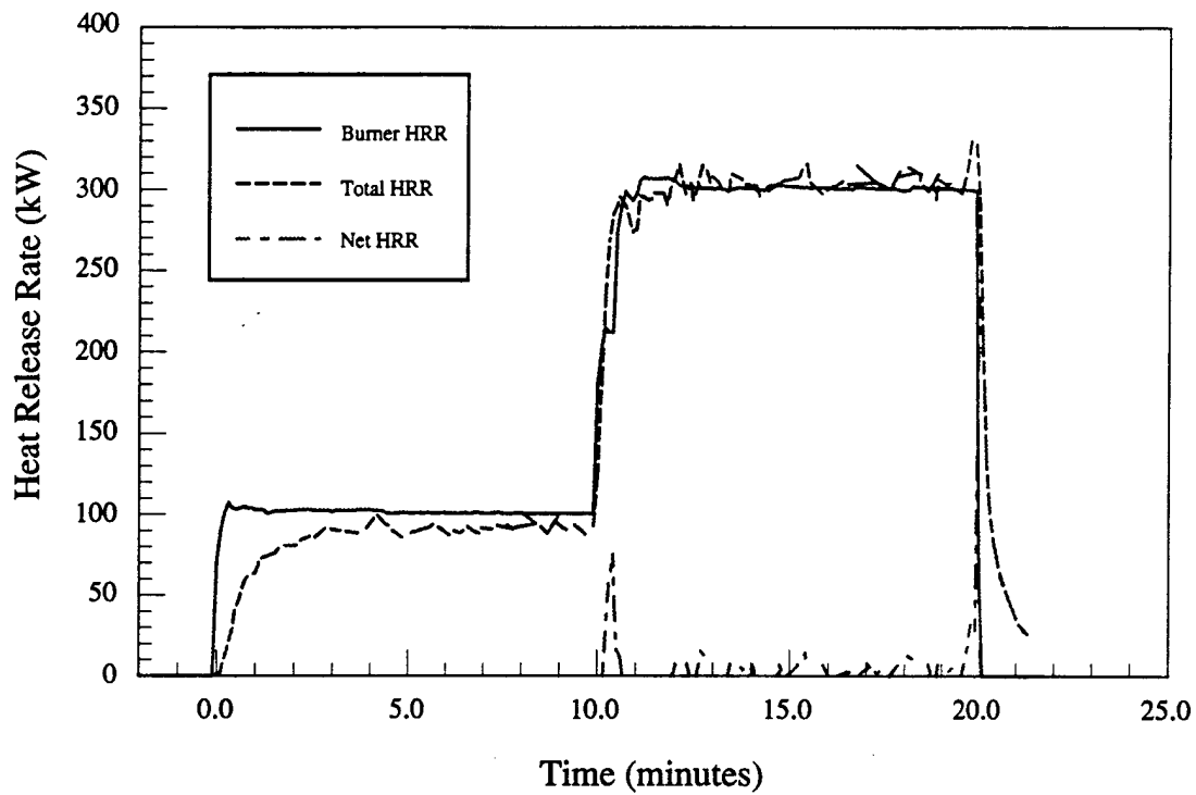
Figure 9.a - Steel - Luggage rack - Heat release rate vs. time
