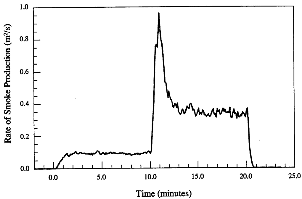
Figure 2.b - Material # 2 - Smoke production rate vs. time
