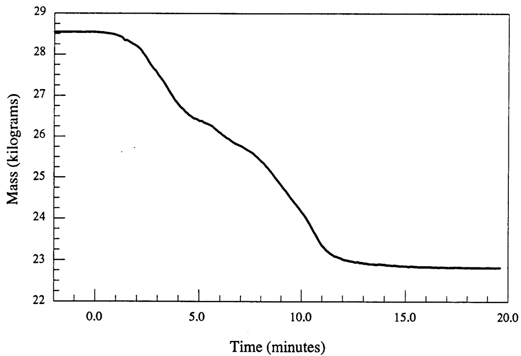
Figure 5.c - Material # 3 - Double chair - Mass vs. time
