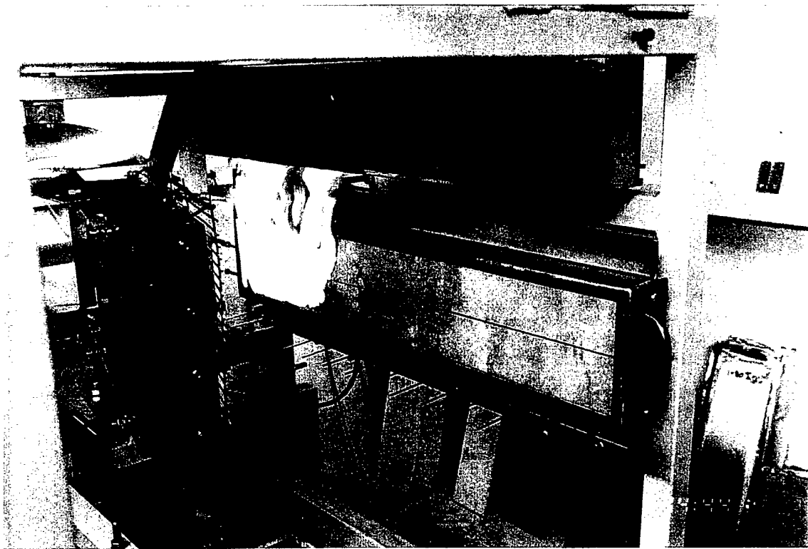
Figure 7. ASTM E1321 Flame Spread Test in Progress.
