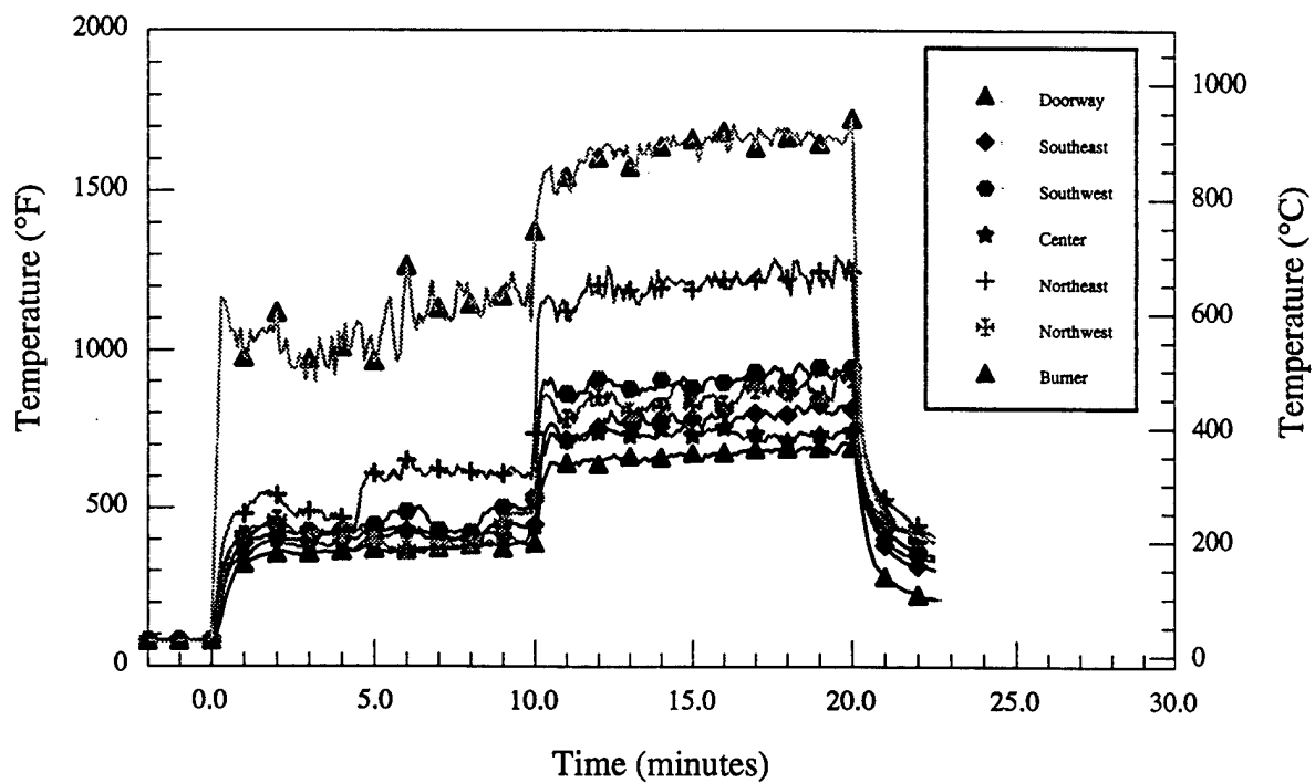
Figure 7.d - Material # 7 - Room temperatures vs. time
