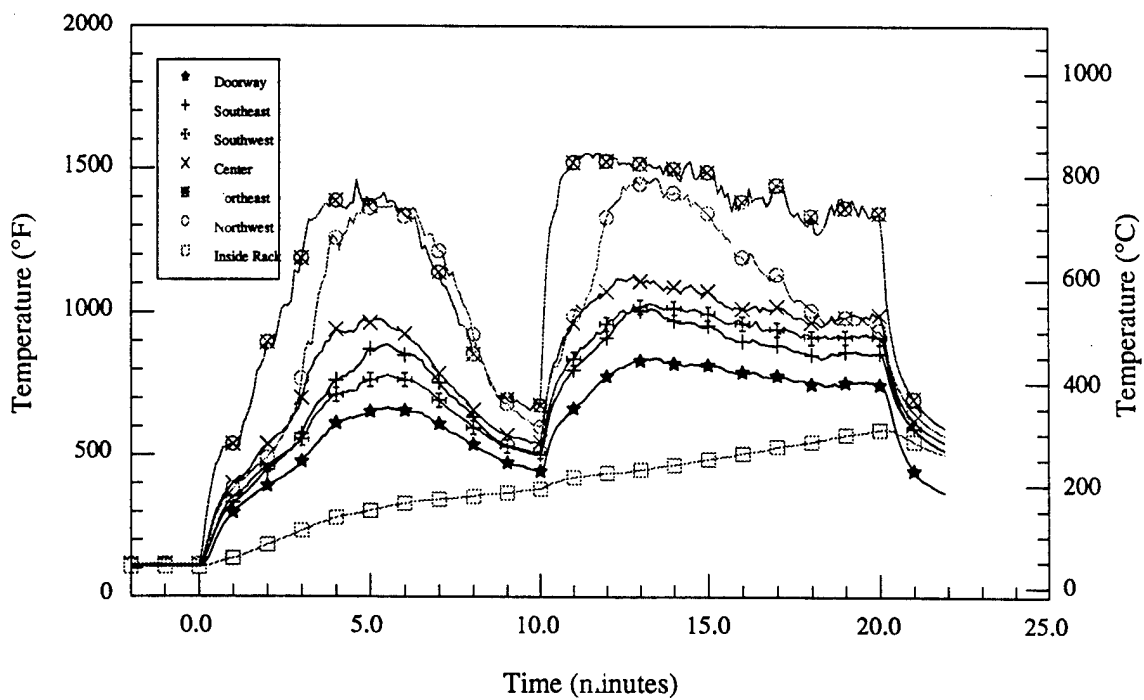
Figure 13.d - Material # 5 - Luggage rack - Room temperatures vs. time
