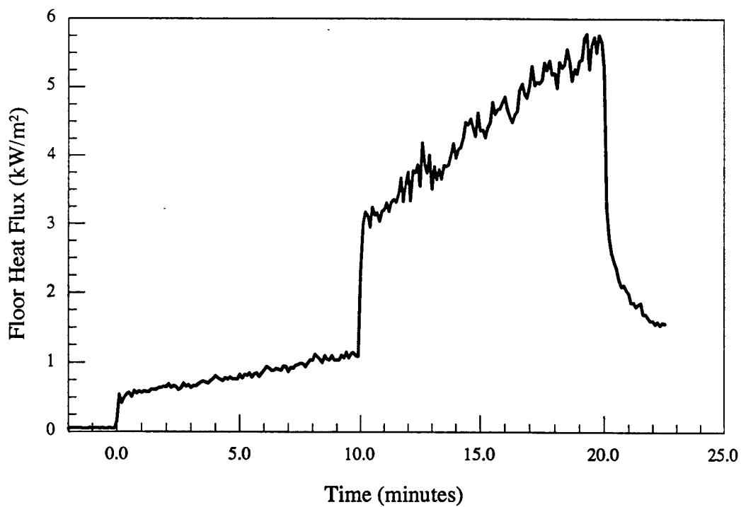
Figure 7.c - Material # 7 - Floor heat flux vs. time
