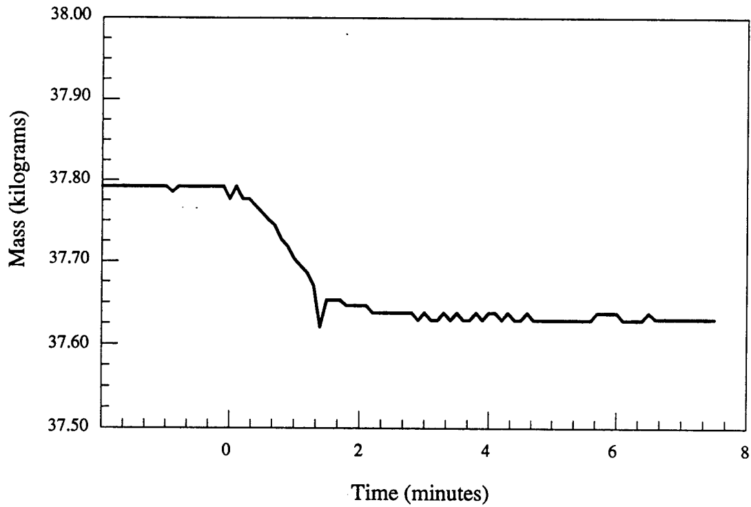
Figure 2.c - Steel - Double chair - Mass vs. time
