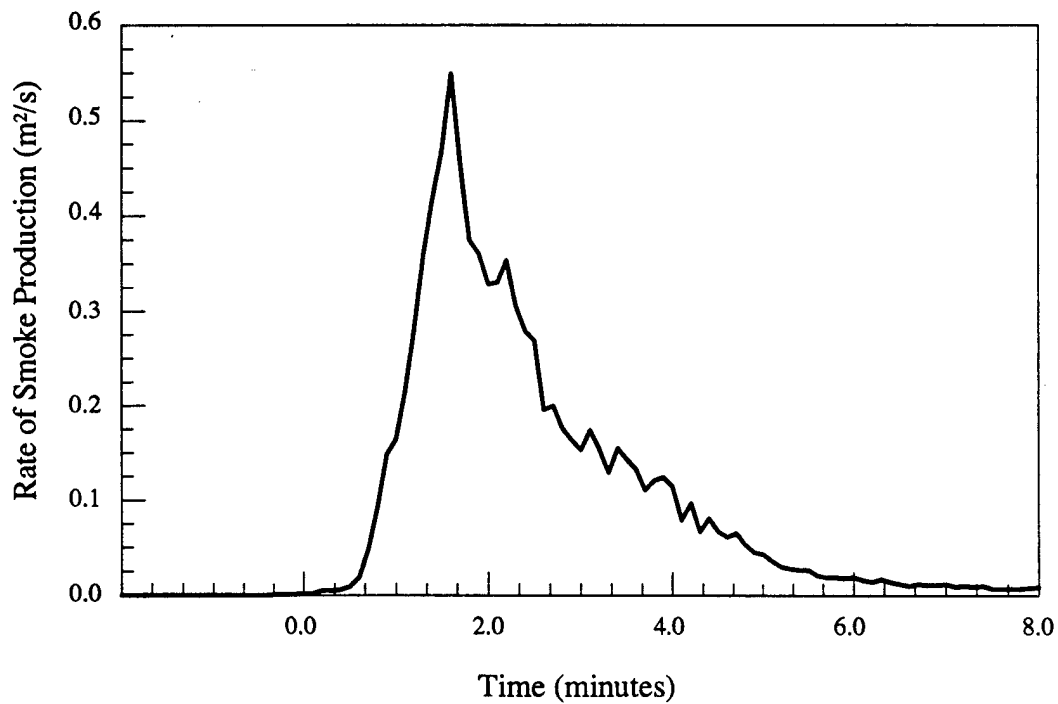
Figure 1.b - Steel - Smoke production rate vs. time
