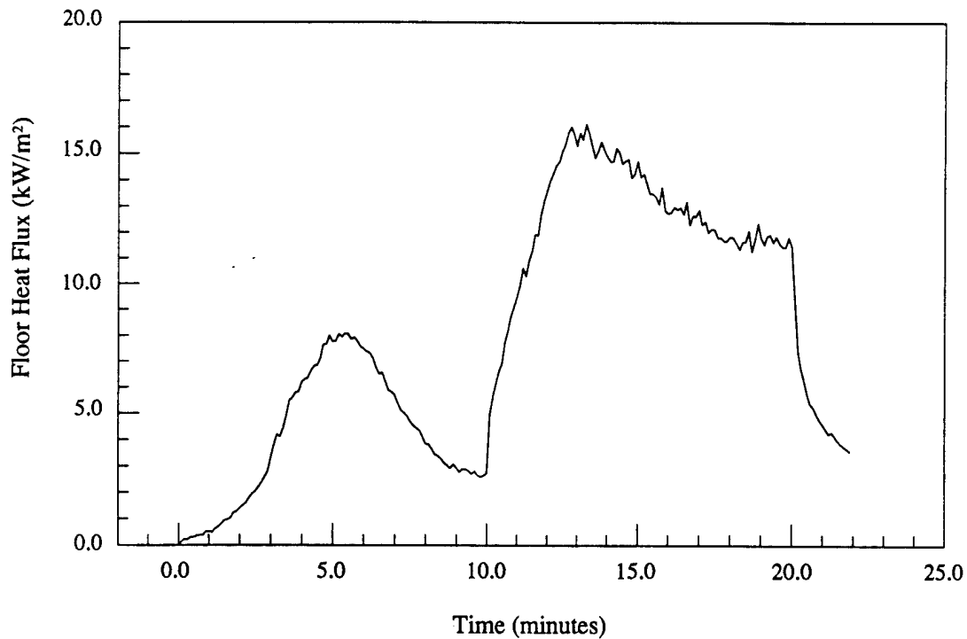
Figure 13.c - Material # 5 - Luggage rack - Floor heat flux vs. time
