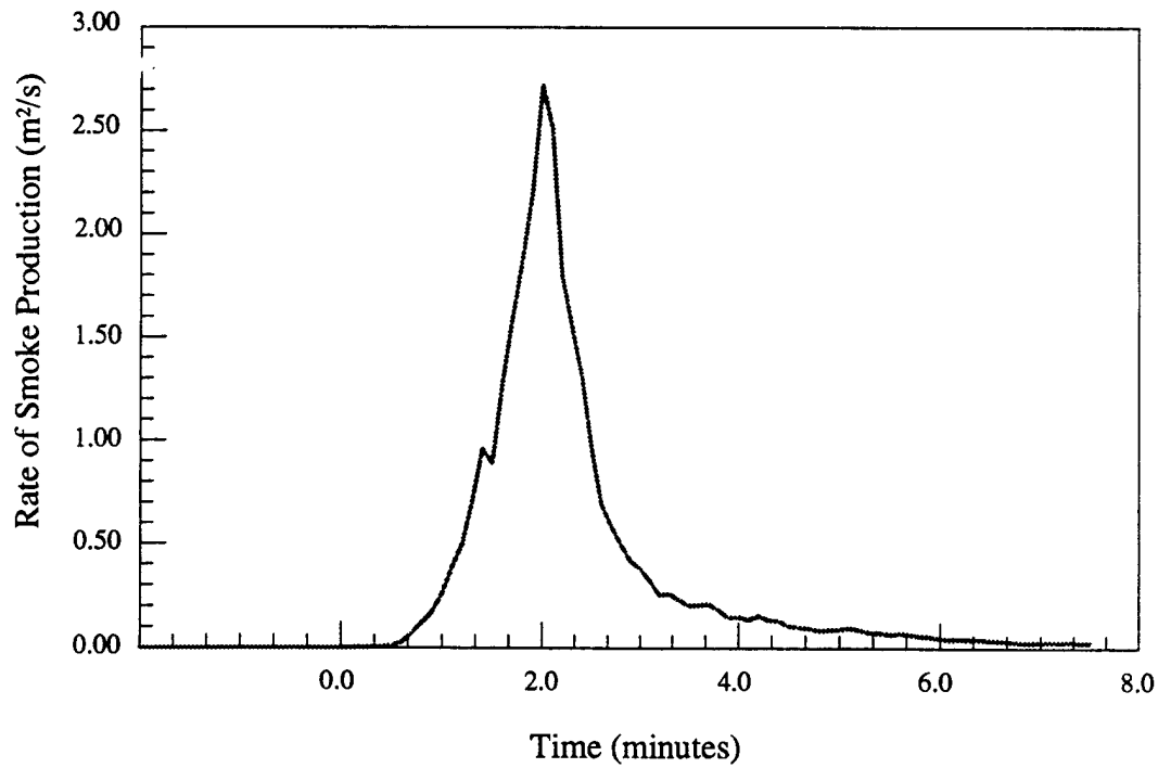
Figure 4.b - Material # 1 - Double chair - Smoke production rate vs. time
