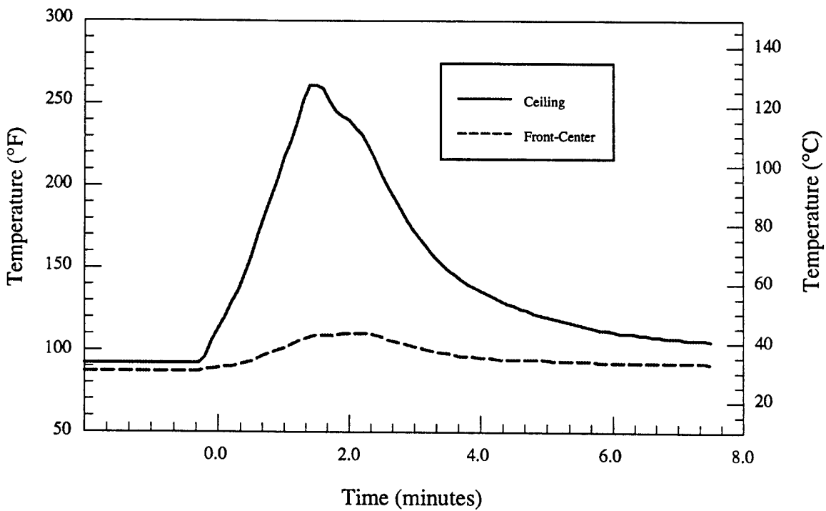
Figure 3.d - Material # 1 - Single chair - Room temperatures vs. time
