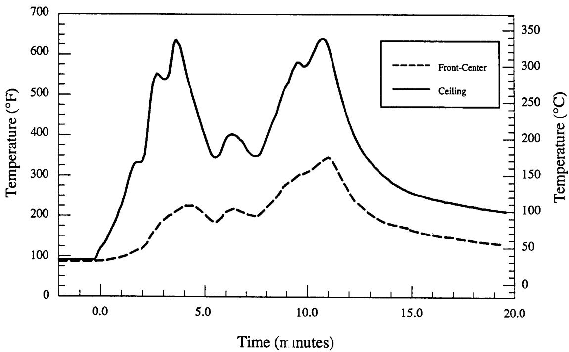
Figure 5.d - Material # 3 - Double chair - Room temperatures vs. time
