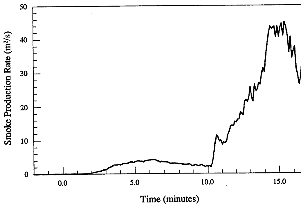
Figure 5.b - Material # 5 - Smoke production rate vs. time
