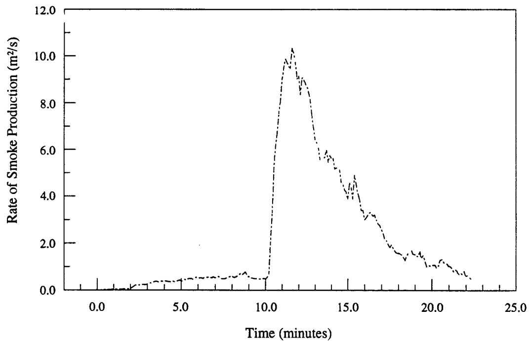
Figure 12.b - Material # 4 - Luggage rack - Smoke production rate vs. time
