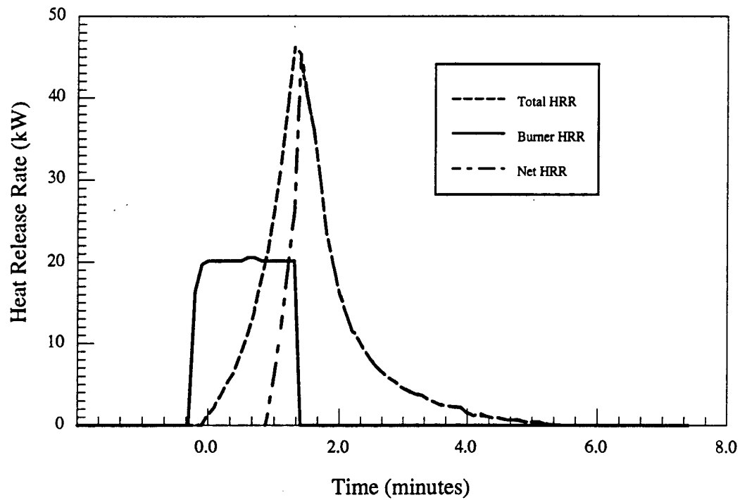
Figure 6.a - Material # 4 - Single chair - Heat release rate vs. time
