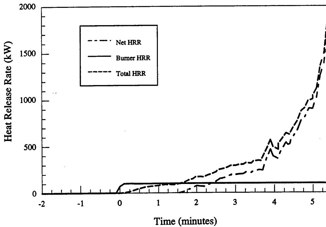
Figure 4.a - Material # 4 - Heat release rate vs. time
