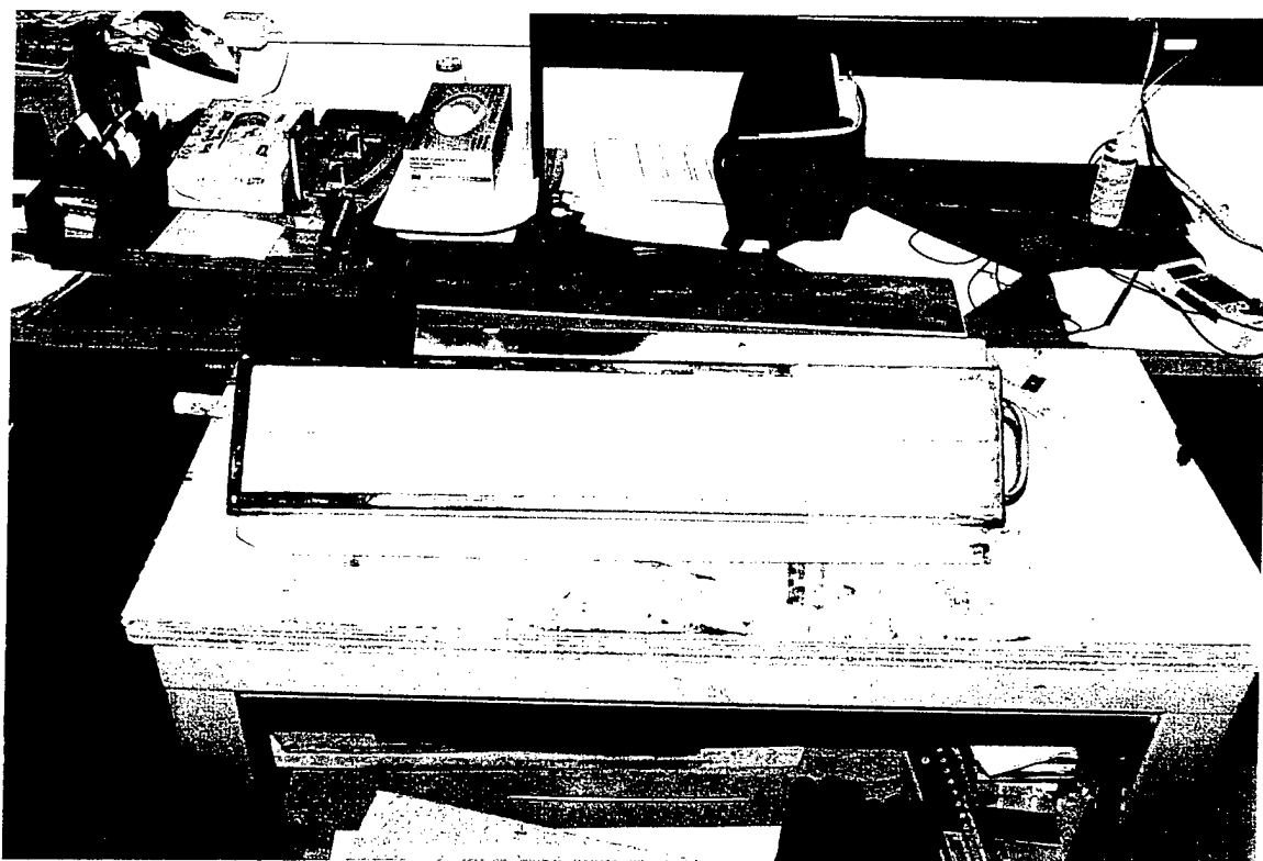
Figure 6. Finished Flame Spread Sample Mounted in Specimen Holder.
