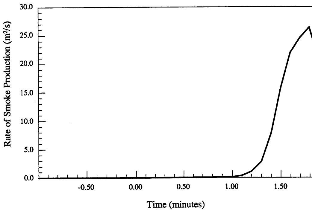
Figure 8.b - Material # 8 - Smoke production rate vs. time
