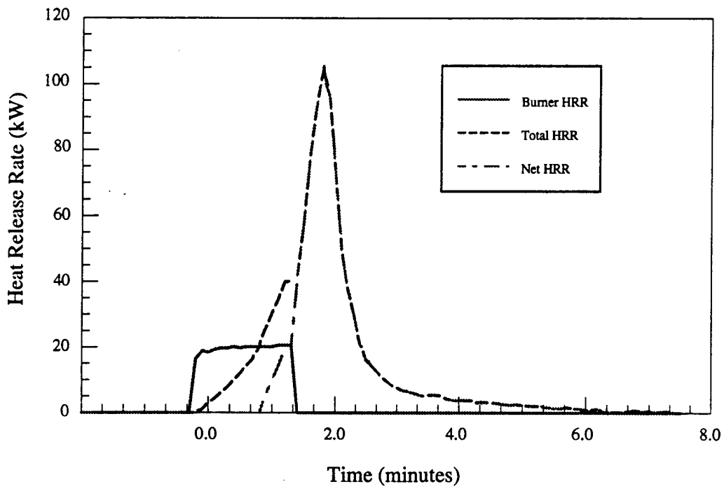
Figure 4.a - Material # 1 - Double chair - Heat release rate vs. time
