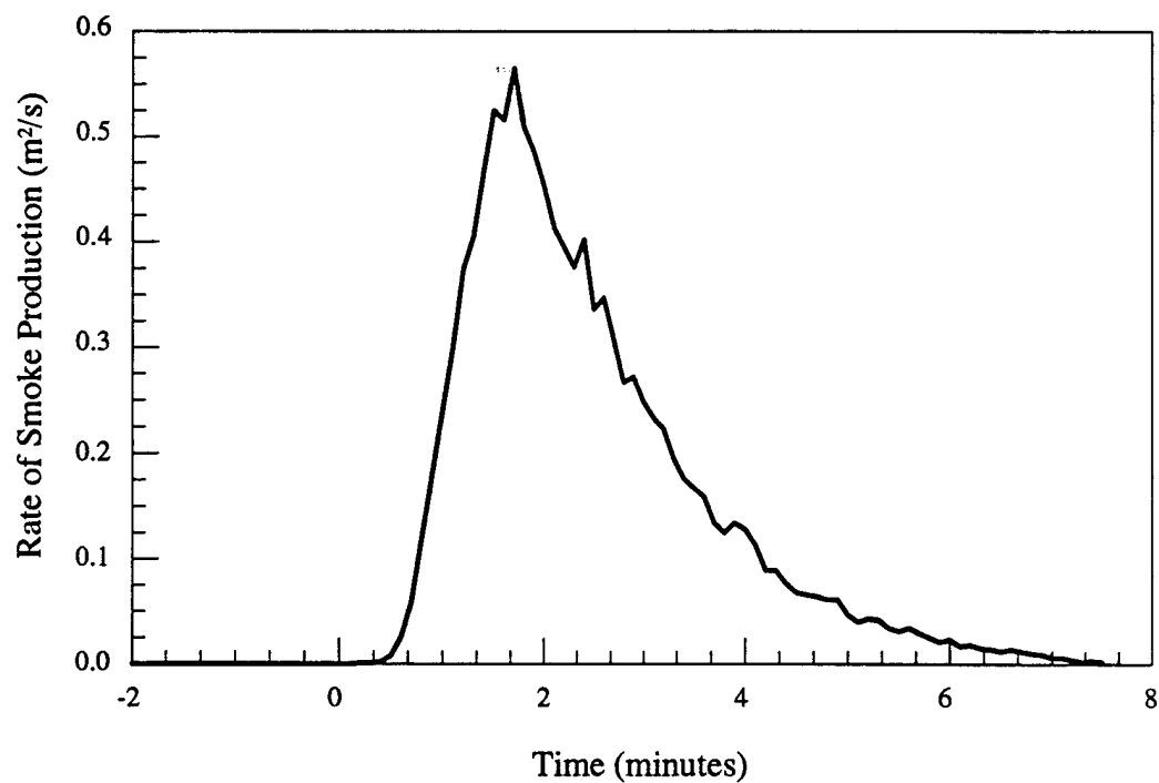
Figure 2.b - Steel - Double chair - Smoke production rate vs. time
