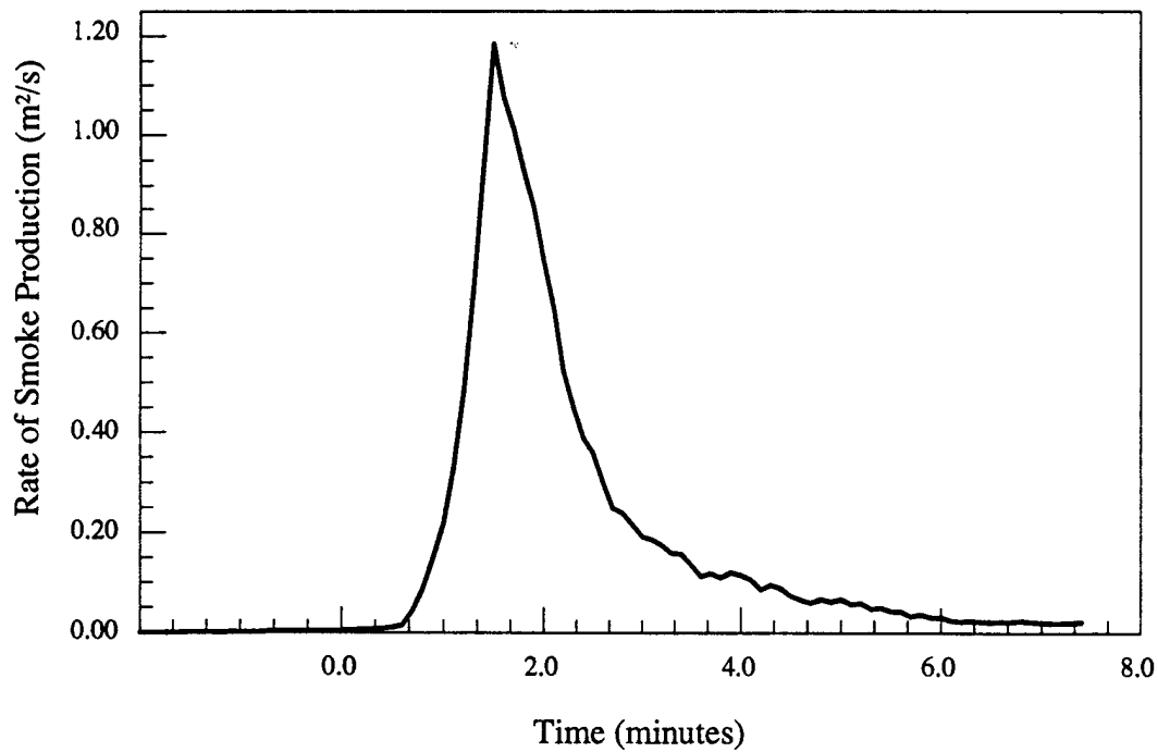
Figure 6.b - Material # 4 - Single chair - Smoke production rate vs. time
