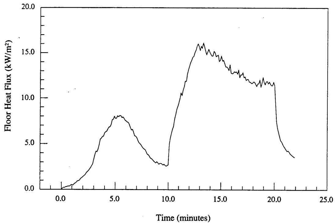
Figure 11.c - Material # 3 - Luggage rack - Floor heat flux vs. time
