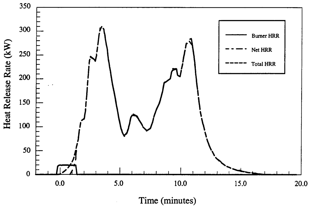
Figure 5.a - Material # 3 - Double chair - Heat release rate vs. time
