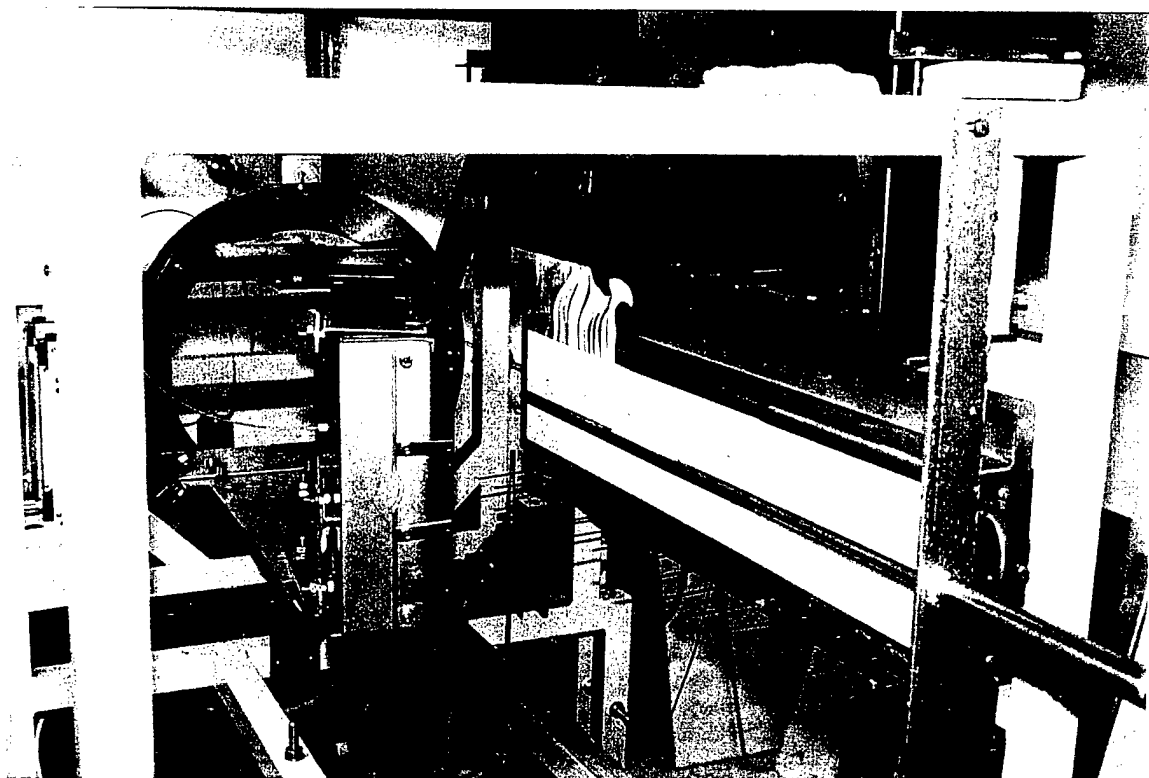
Figure 4. Fume Stack Calibration Burner in Place.
