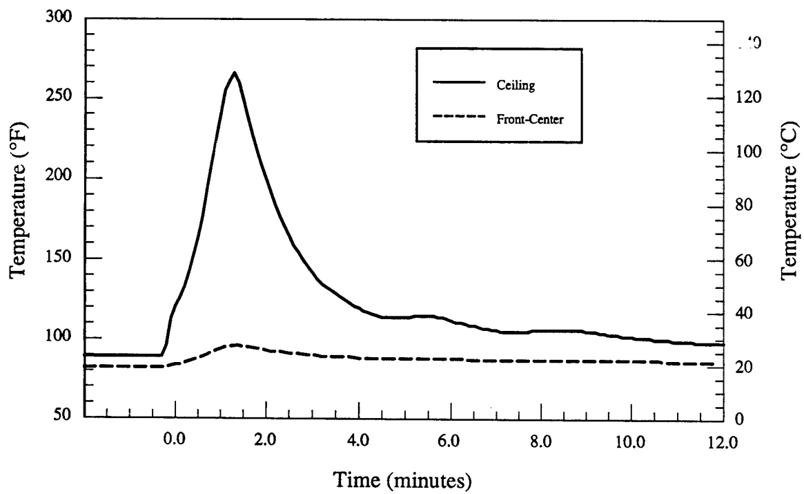
Figure 8.d - Material # 5 - Double chair - Room temperatures vs. time
