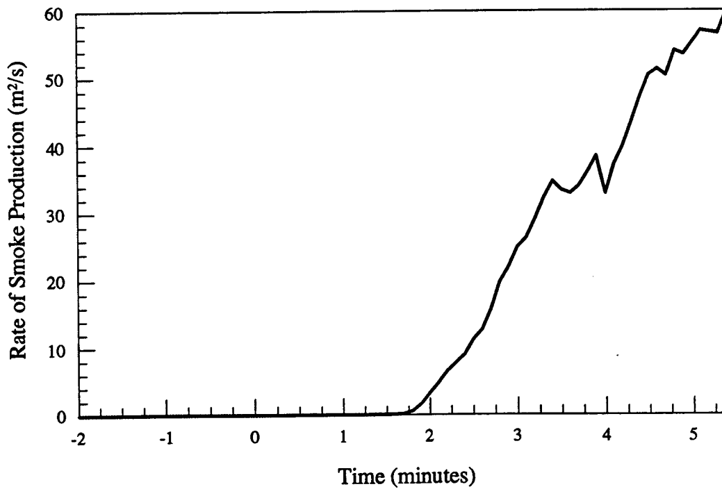
Figure 4.b - Material # 4 - Smoke production rate vs. time
