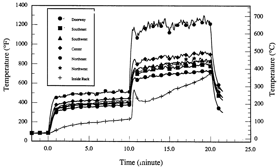
Figure 9.d - Steel - Luggage rack - Room temperatures vs. time
