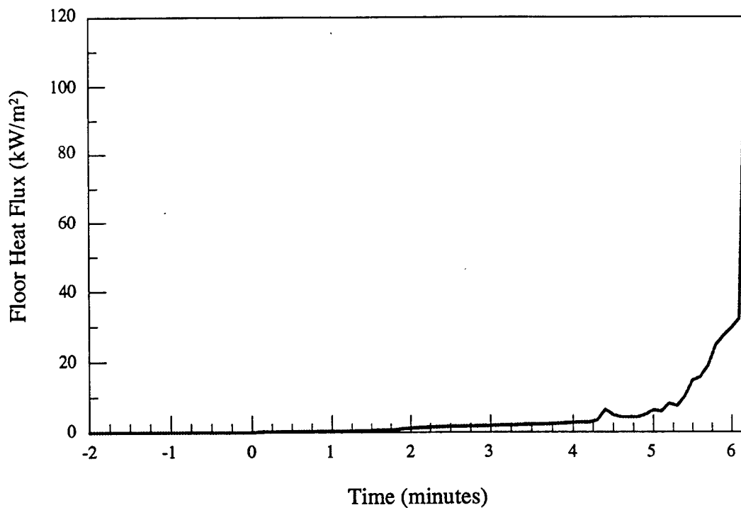
Figure A.3.c - Material # 3 - Floor heat flux vs. time
