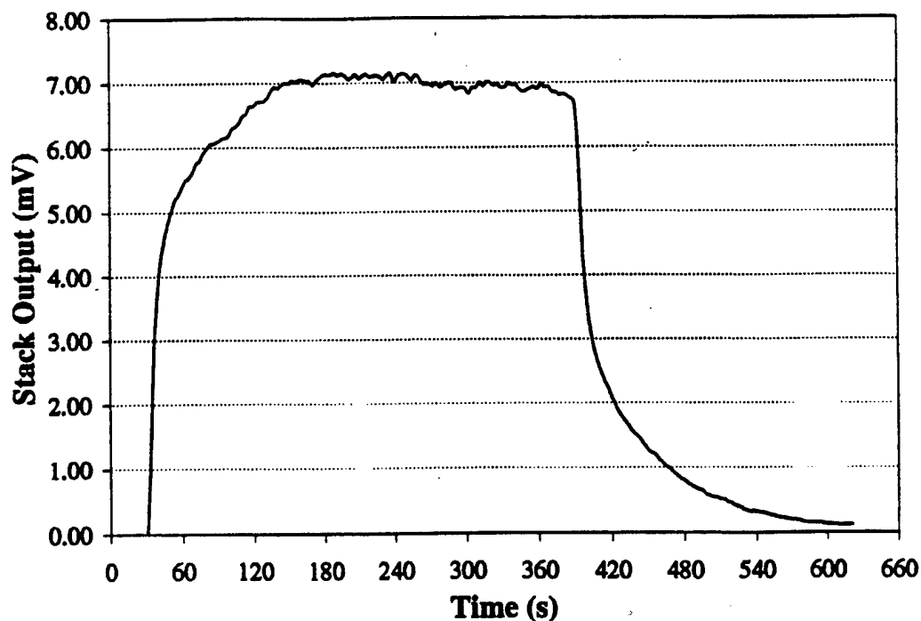
Figure 6.3 – Stack Response to a 7 kW Thermal Pulse
