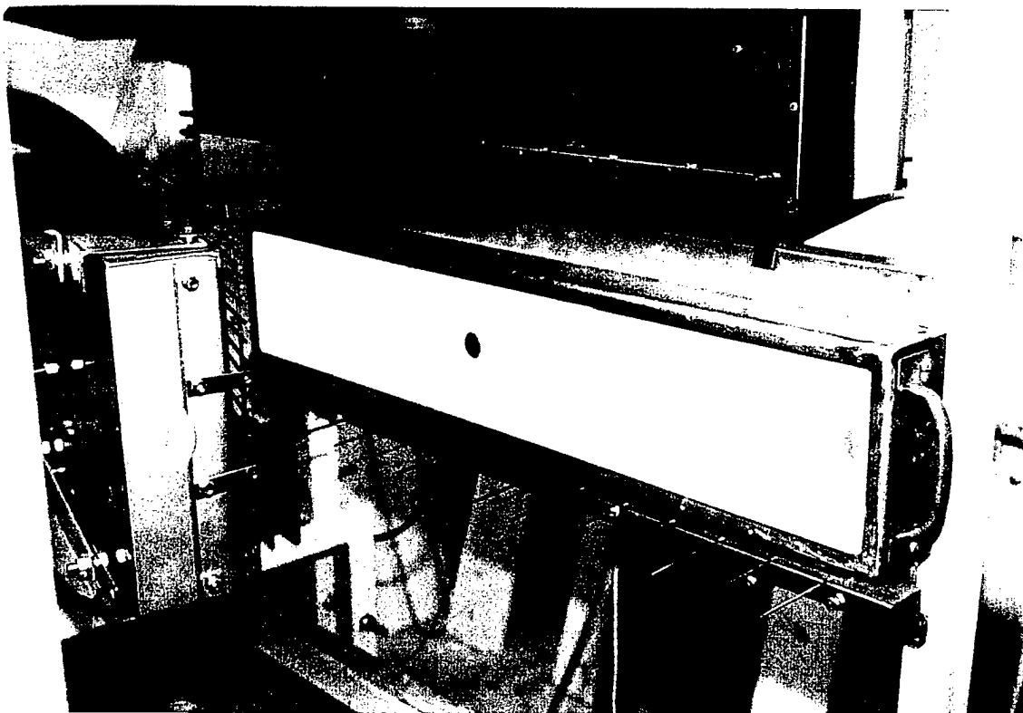
Figure 3. Calibration Board with Radiometer Shown at 350-mm Location.
