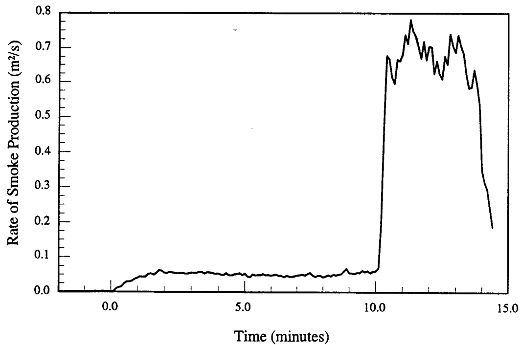
Figure 10.b - Material # 1 - Luggage rack - Smoke production rate vs. time
