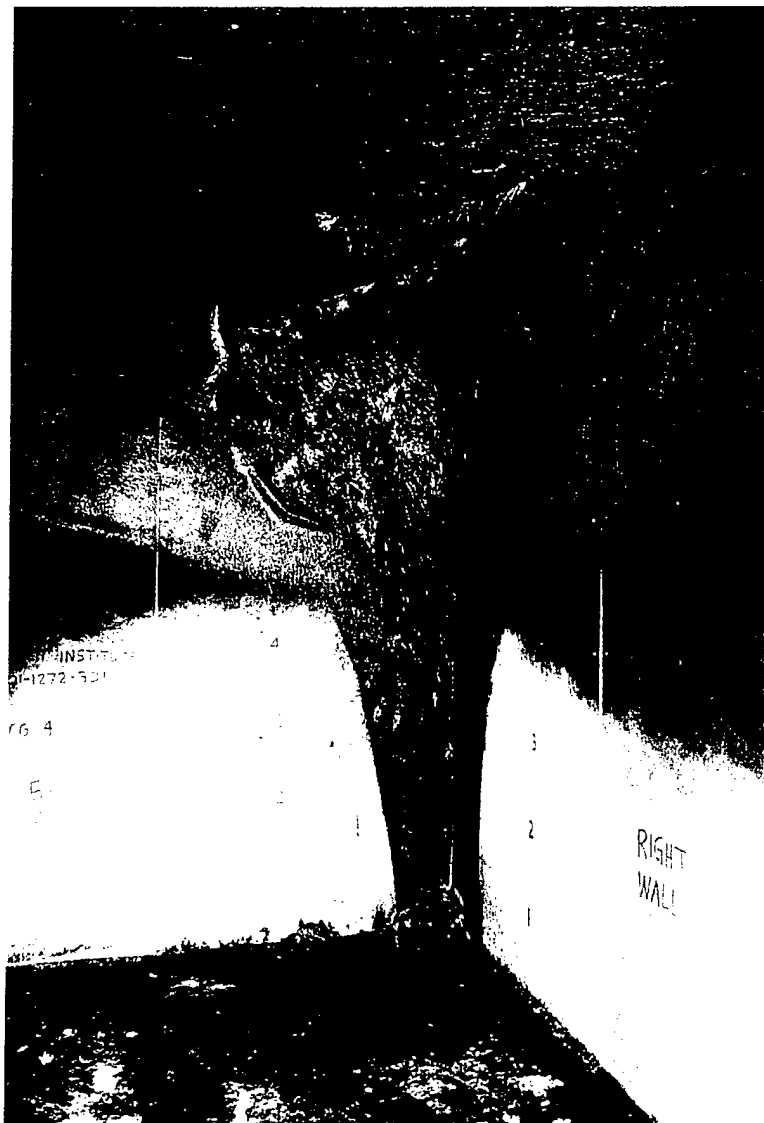
Figure 16. Material No. 4 After Termination of the Room/Corner Test.
