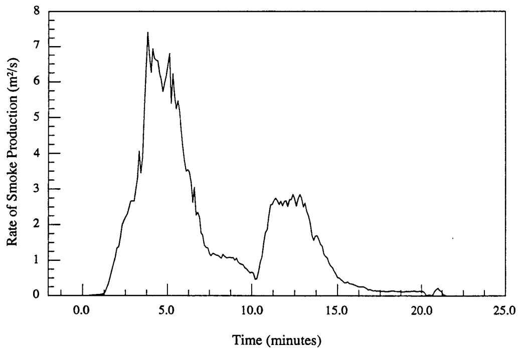
Figure 11.b - Material # 3 - Luggage rack - Smoke production rate vs. time
