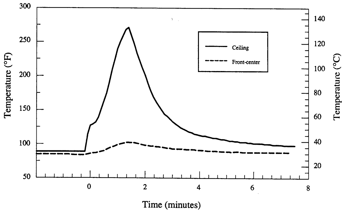
Figure 2.d - Steel - Double chair - Room temperatures vs. time
