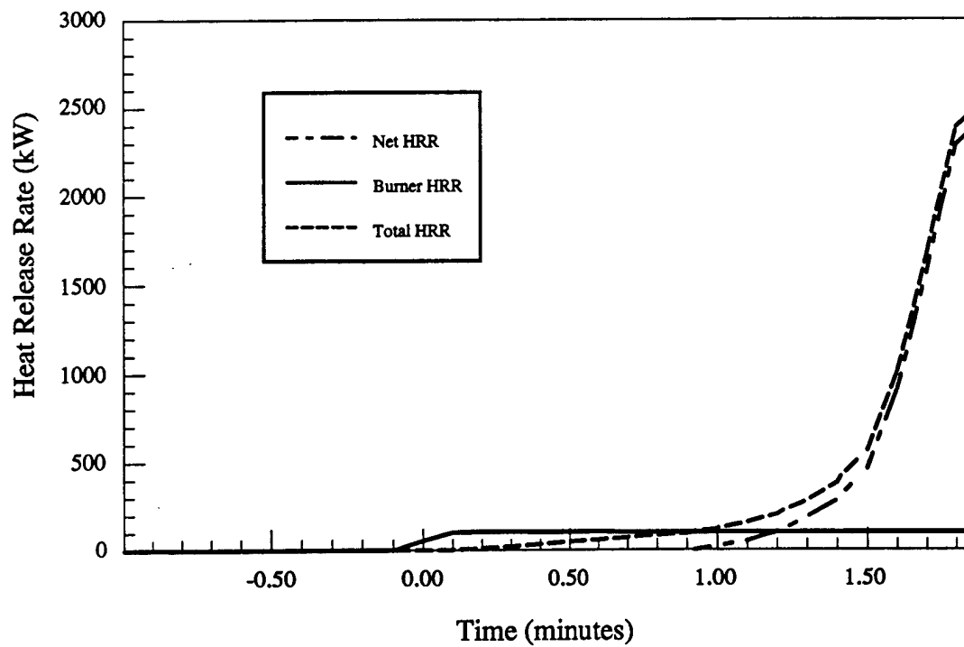
Figure 8.a - Material # 8 - Heat release rate vs. time
