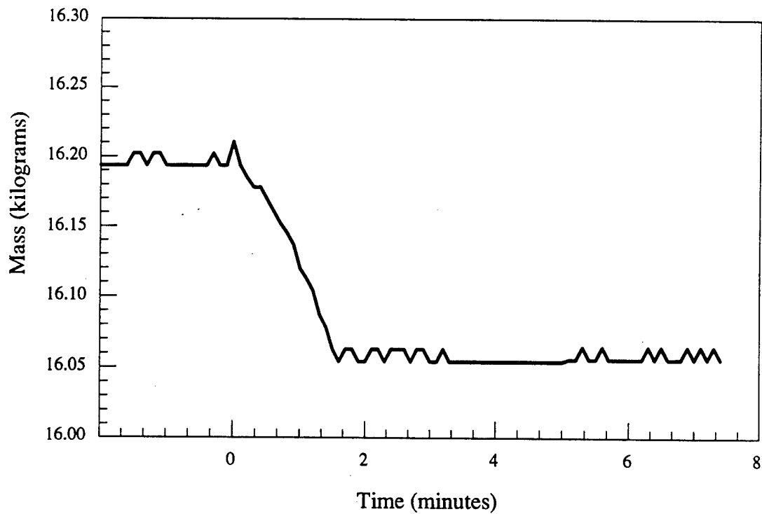
Figure 7.c - Material # 5 - Single chair - Mass vs. time
