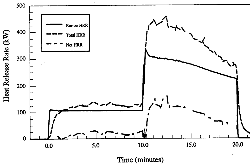
Figure 1.a - Material # 1 - Heat release rate vs. time
