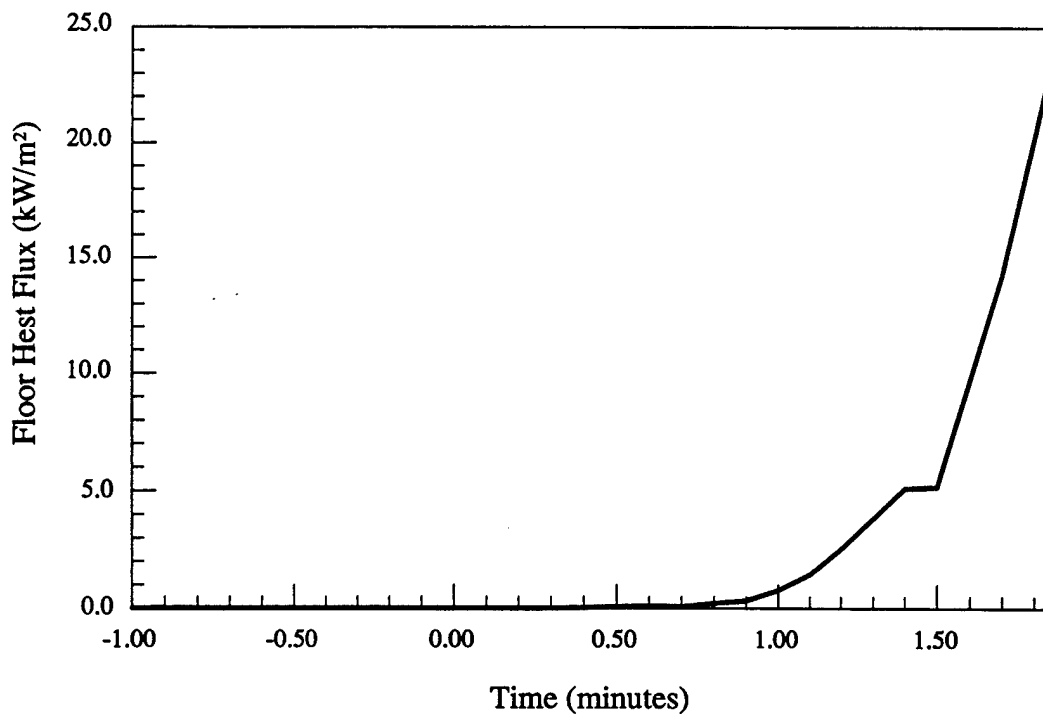
Figure 8.c - Material # 8 - Floor heat flux vs. time
