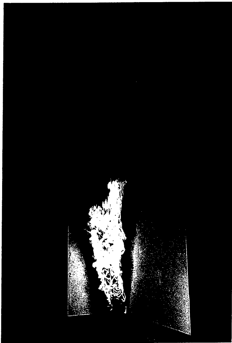
Figure 23. Material No. 6 After 8 Min of Exposure at 300 kW.
