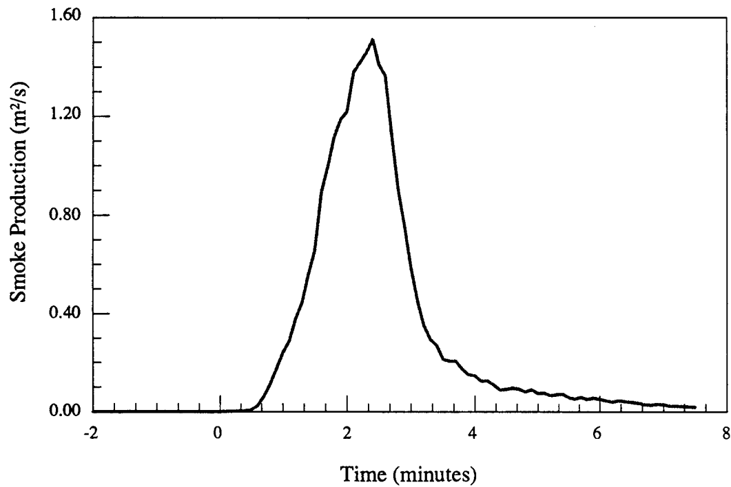
Figure 3.b - Material # 1 - Single chair - Smoke production rate vs. time
