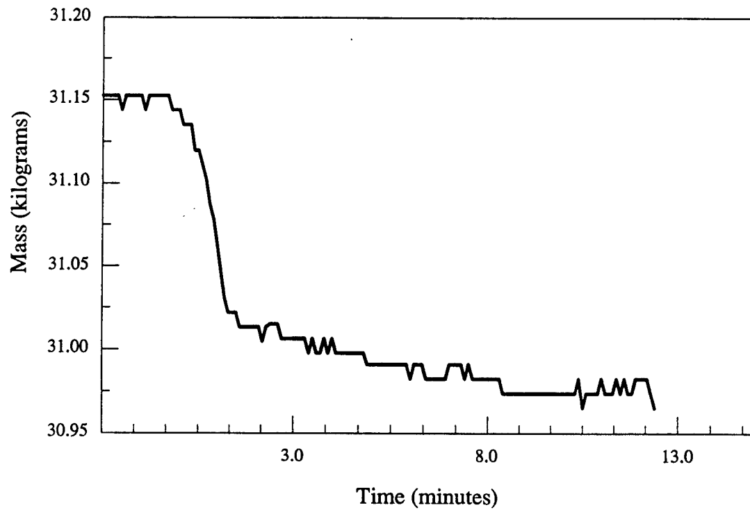
Figure 8.c - Material # 5 - Double chair - Mass vs. time
