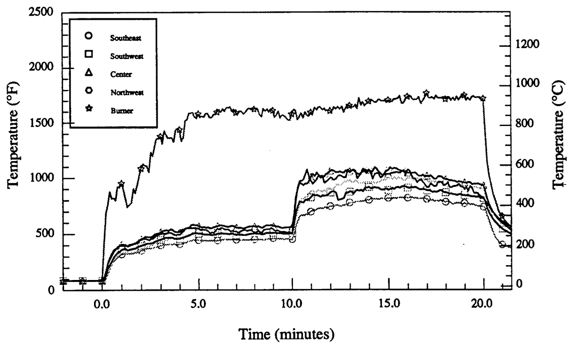
Figure 1.d - Material # 1 - Room temperatures vs. time
