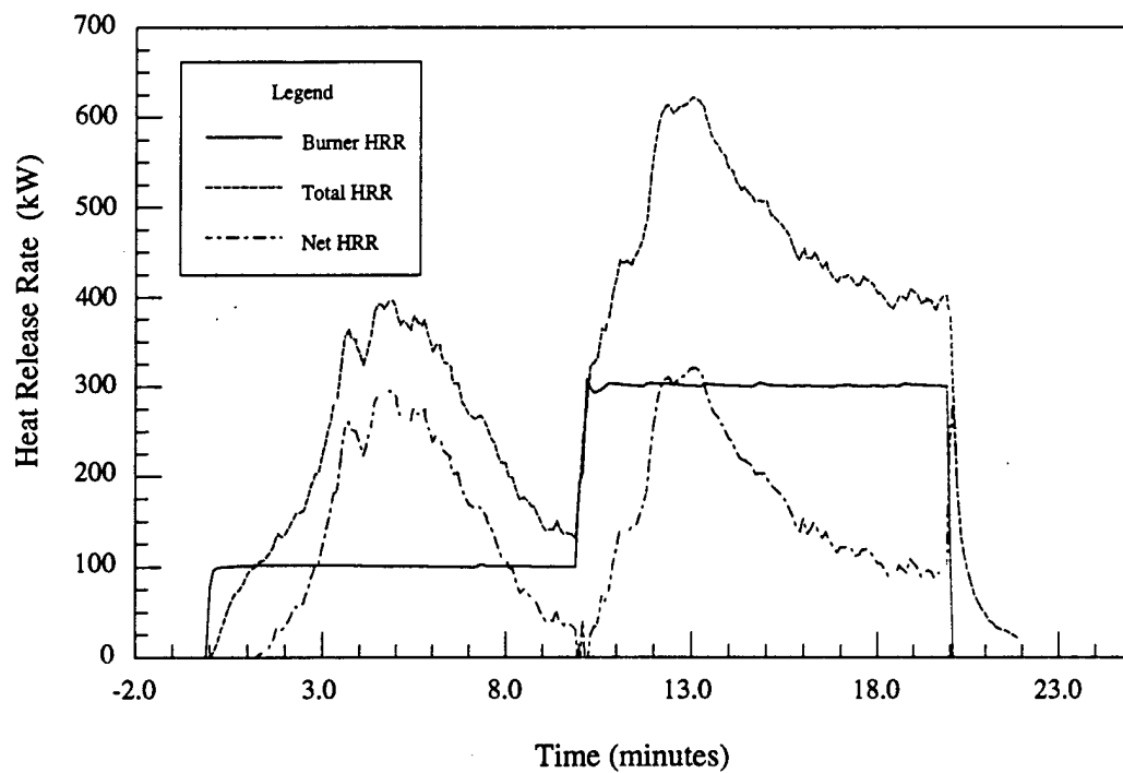
Figure 11.a - Material # 3 - Luggage rack - Heat release rate vs. time
