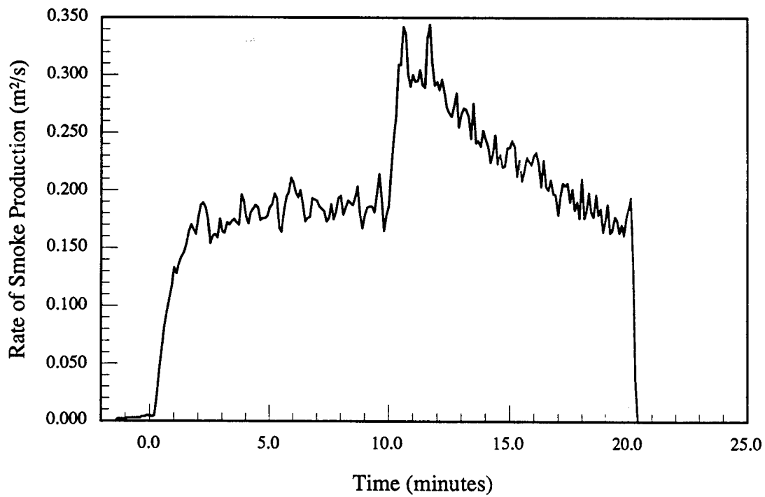
Figure 9.b - Steel - Luggage rack - Smoke production rate vs. time
