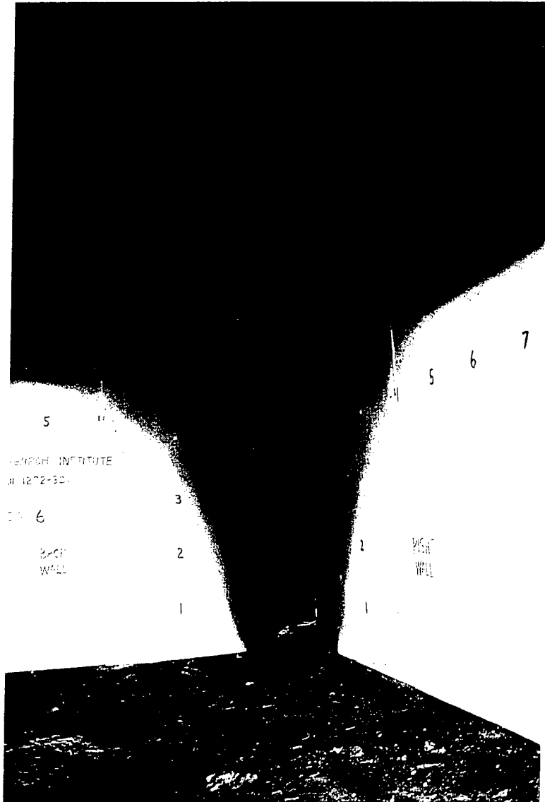
Figure 24. Material No. 6 After Termination of the Room/Corner Test.
