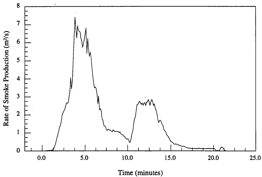
Figure 13.b - Material # 5 - Luggage rack - Smoke production rate vs. time
