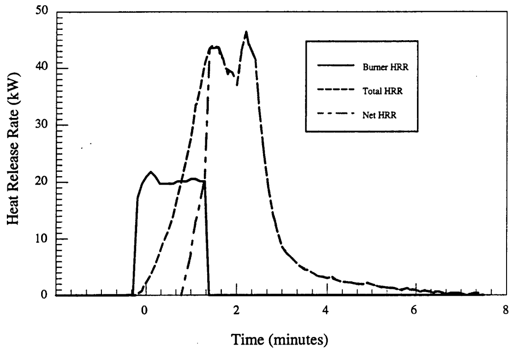
Figure 3.a - Material # 1 - Single chair - Heat release rate vs. time
