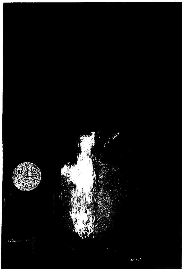
Figure 19. Material No. 5 Just Prior to Flashover.
