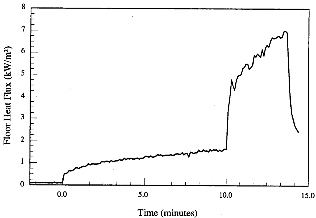
Figure 10.c - Material # 1 - Luggage rack - Floor heat flux vs. time
