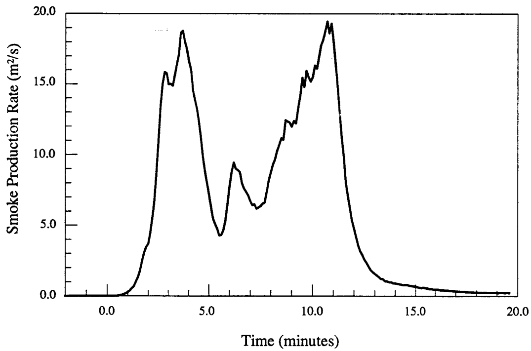
Figure 5.b - Material # 3 - Double chair - Smoke production rate vs. time
