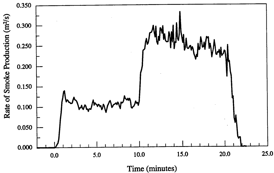
Figure 7.b - Material # 7 - Smoke production rate vs. time
