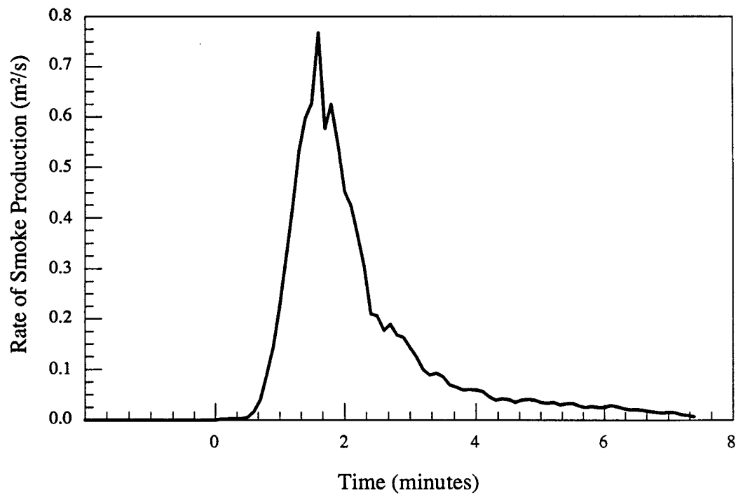
Figure 7.b - Material # 5 - Single chair - Smoke production rate vs. time
