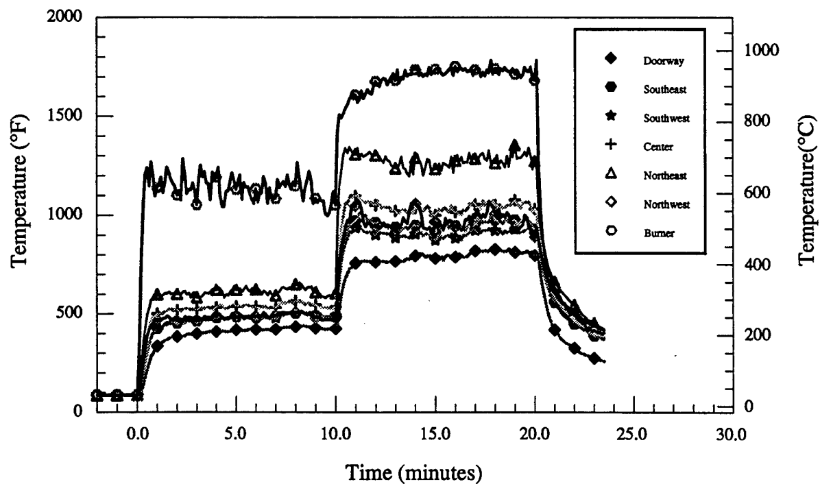
Figure 2.d - Material # 2 - Room temperatures vs. time
