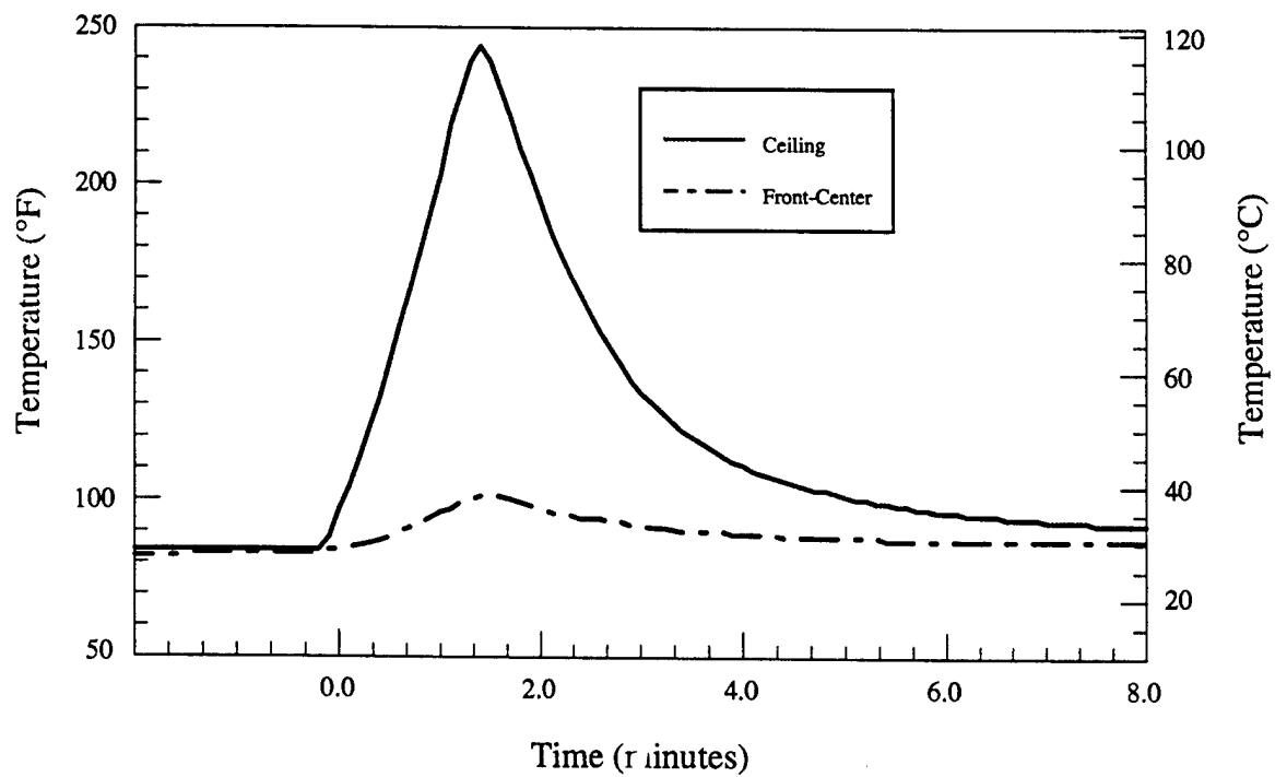
Figure 1.d - Steel - Single Chair - Room temperatures vs. time
