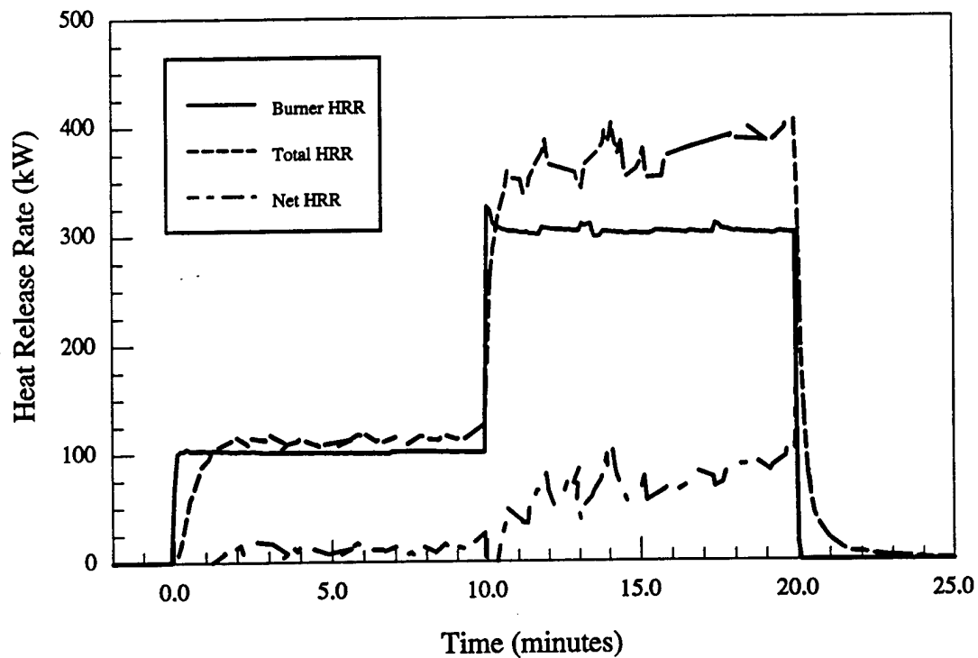
Figure 6.a - Material # 6 - Heat release rate vs. time
