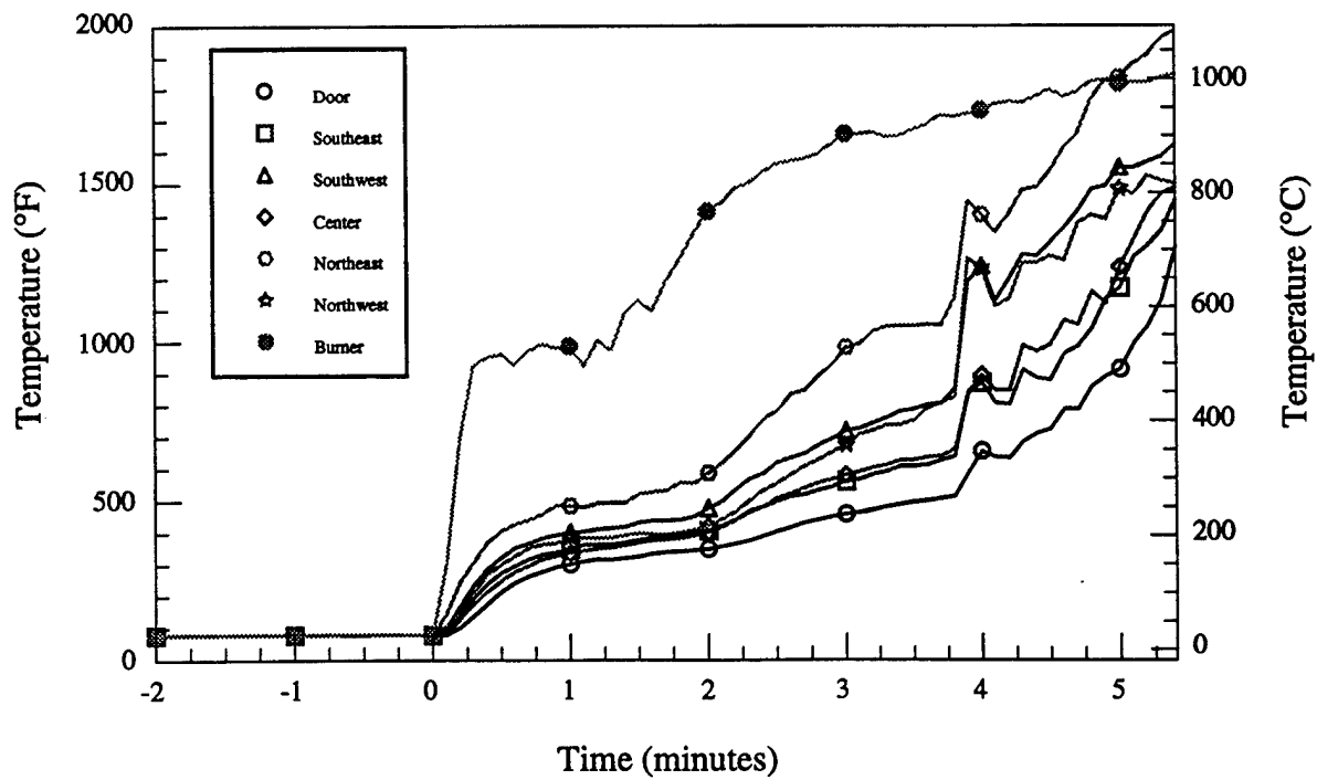
Figure 4.d - Material # 4 - Room temperatures vs. time
