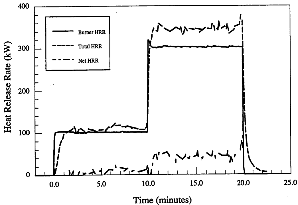
Figure 7.a - Material # 7 - Heat release rate vs. time
