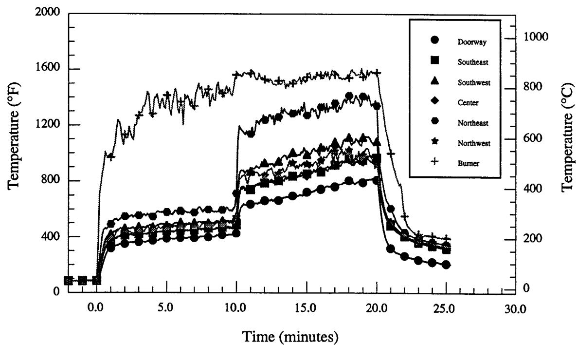
Figure 6.d - Material # 6 - Room temperatures vs. time
