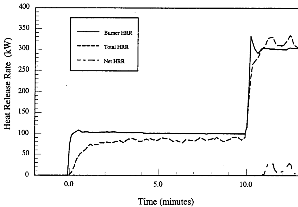
Figure 10.a - Material # 1 - Luggage rack - Heat release rate vs. time
