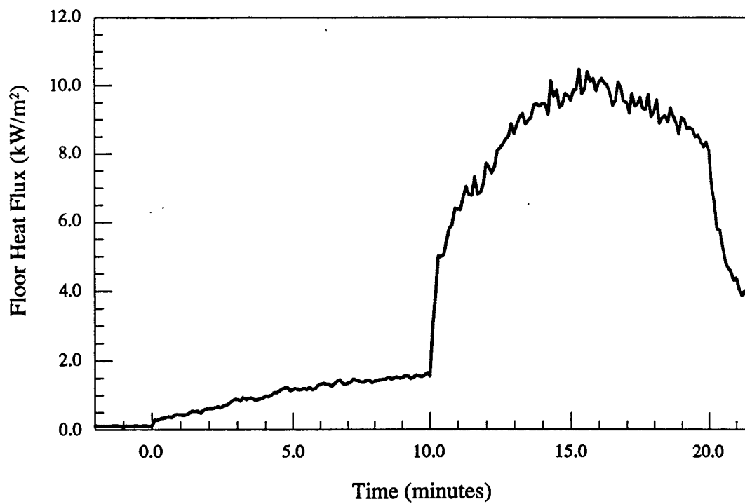
Figure 1.c - Material # 1 - Floor heat flux vs. time
