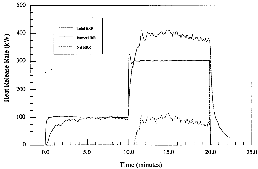
Figure 12.a - Material # 4 - Luggage rack - Heat release rate vs. time
