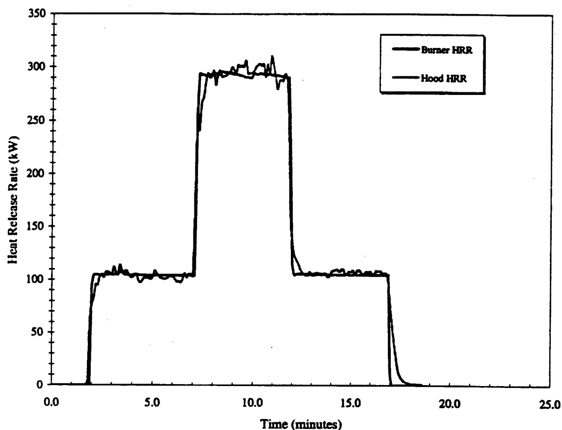
Figure 3.1 - Comparison of Heat Release Rate for Burner and Exhaust Hood Calculated from Calibration Data
