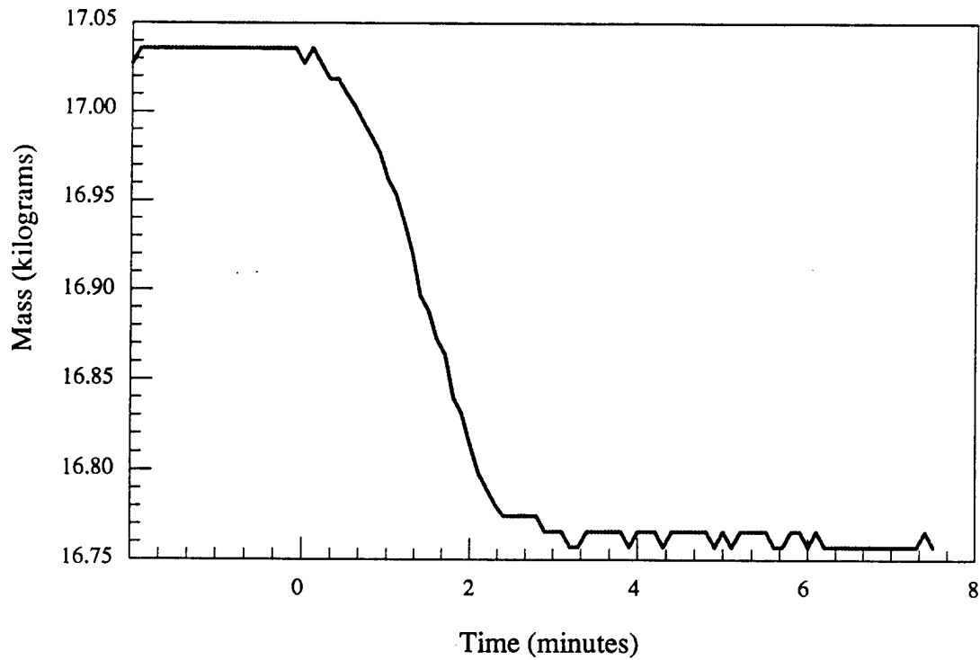
Figure 3.c - Material # 1 - Single chair - Mass vs. time
