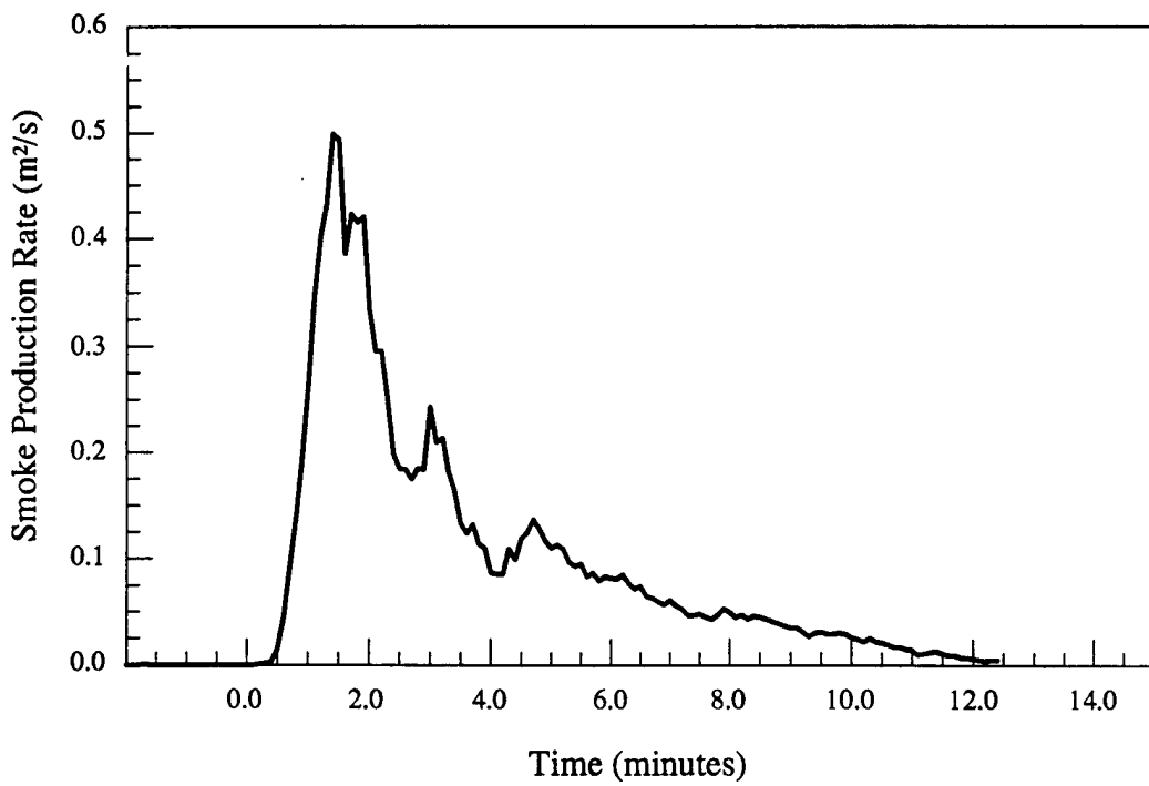
Figure 8.b - Material # 5 - Double chair - Smoke production rate vs. time
