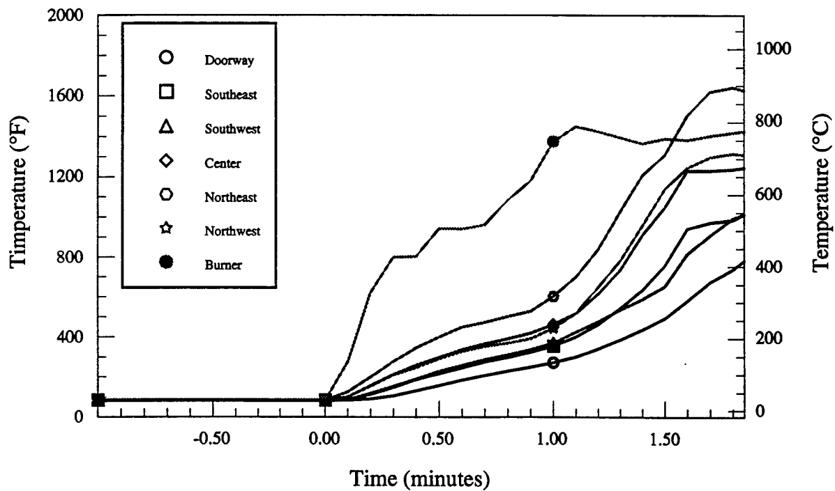
Figure 8.d - Material # 8 - Room temperatures vs. time
