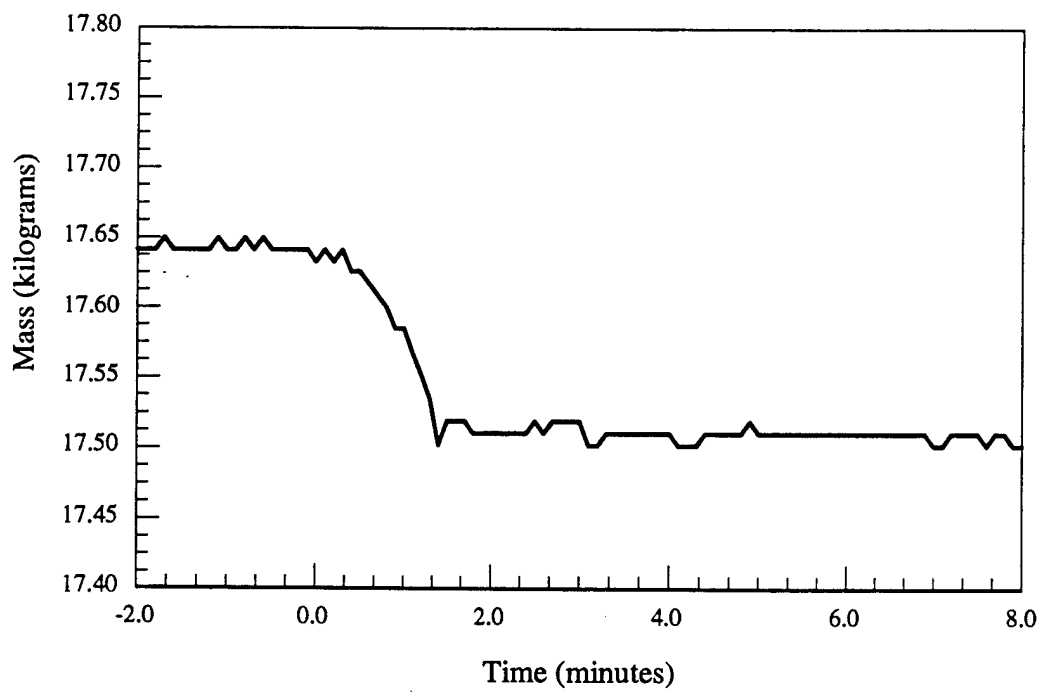
Figure 1.c - Steel - Mass vs. time
