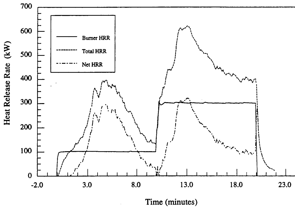
Figure 13.a - Material # 5 - Luggage rack - Heat release rate vs. time
