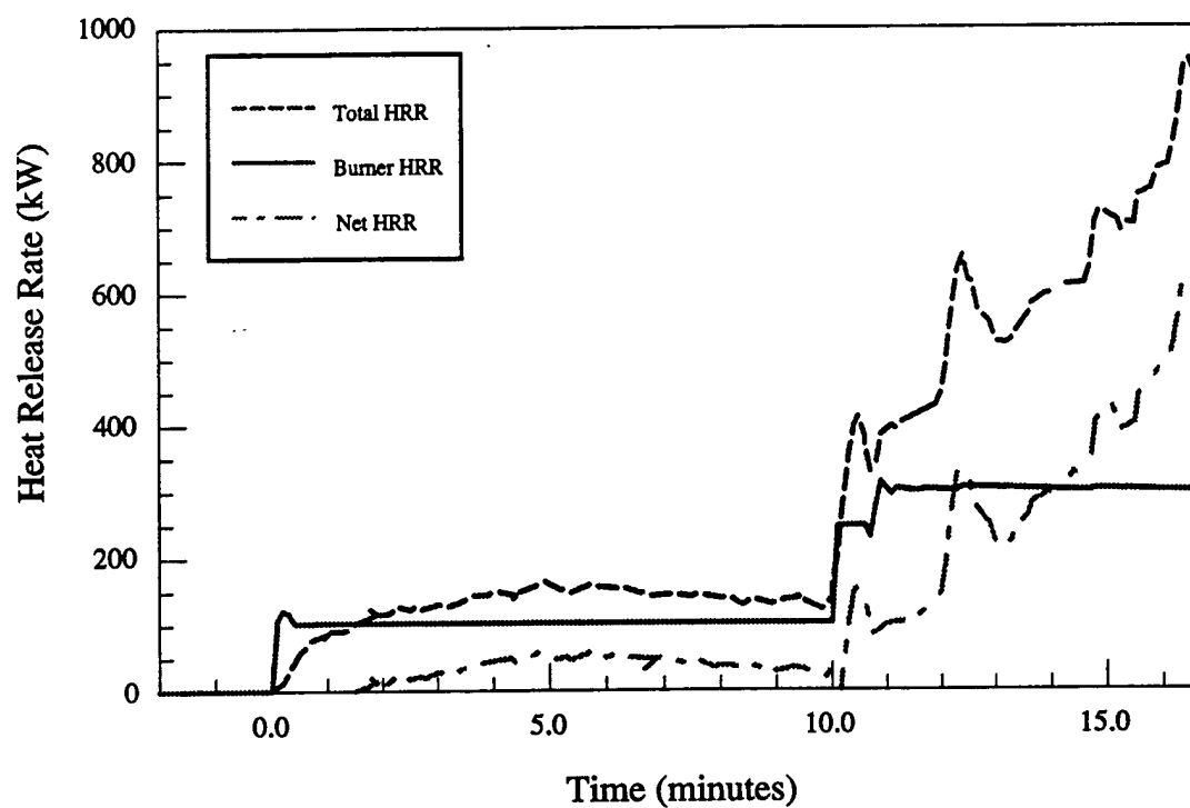
Figure 5.a - Material # 5 - Heat release rate vs. time
