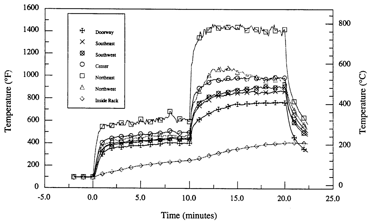
Figure 12.d - Material # 4 - Luggage rack - Room temperatures vs. time
