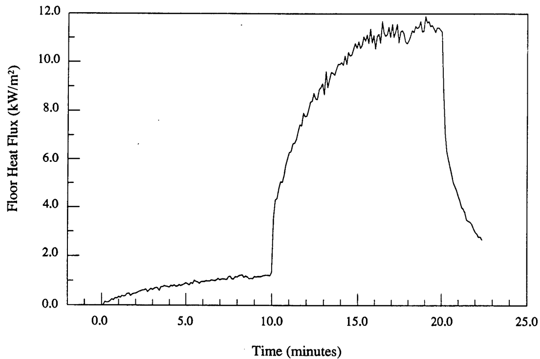
Figure 12.c - Material # 4 - Luggage rack - Floor heat flux vs. time
