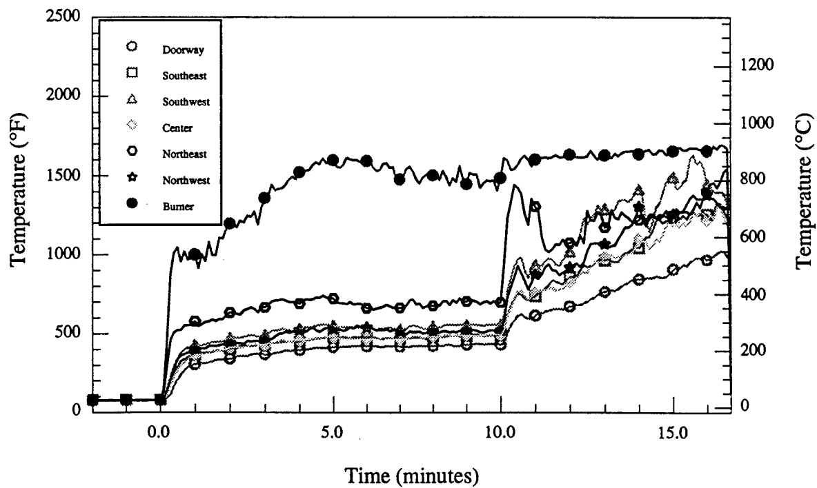
Figure 5.d - Material # 5 - Room temperatures vs. time
