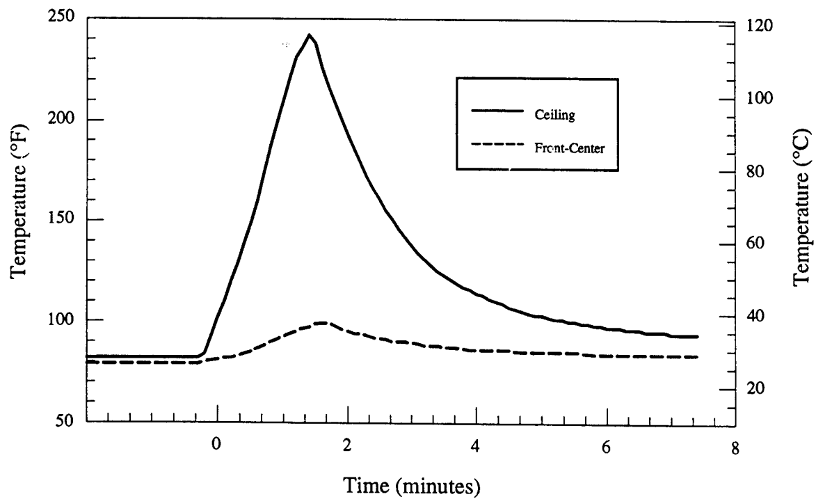
Figure 7.d - Material # 5 - Single chair - Room temperatures vs. time
