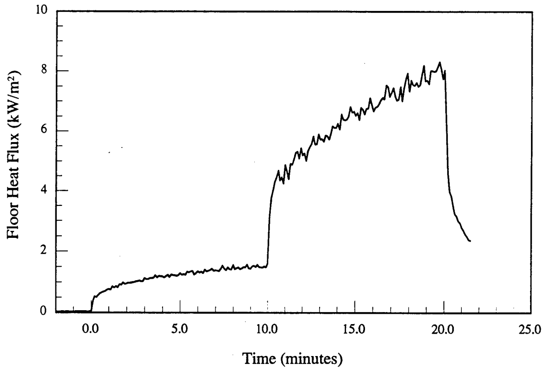
Figure 9.c - Steel - Luggage rack - Floor heat flux vs. time
