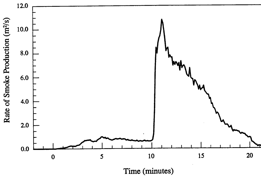
Figure 1.b - Material # 1 - Smoke production rate vs. time
