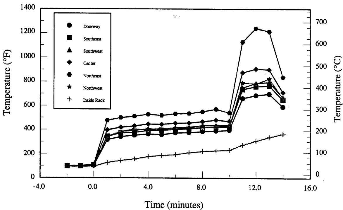
Figure 10.d - Material # 1 - Luggage rack - Room temperatures vs. time
