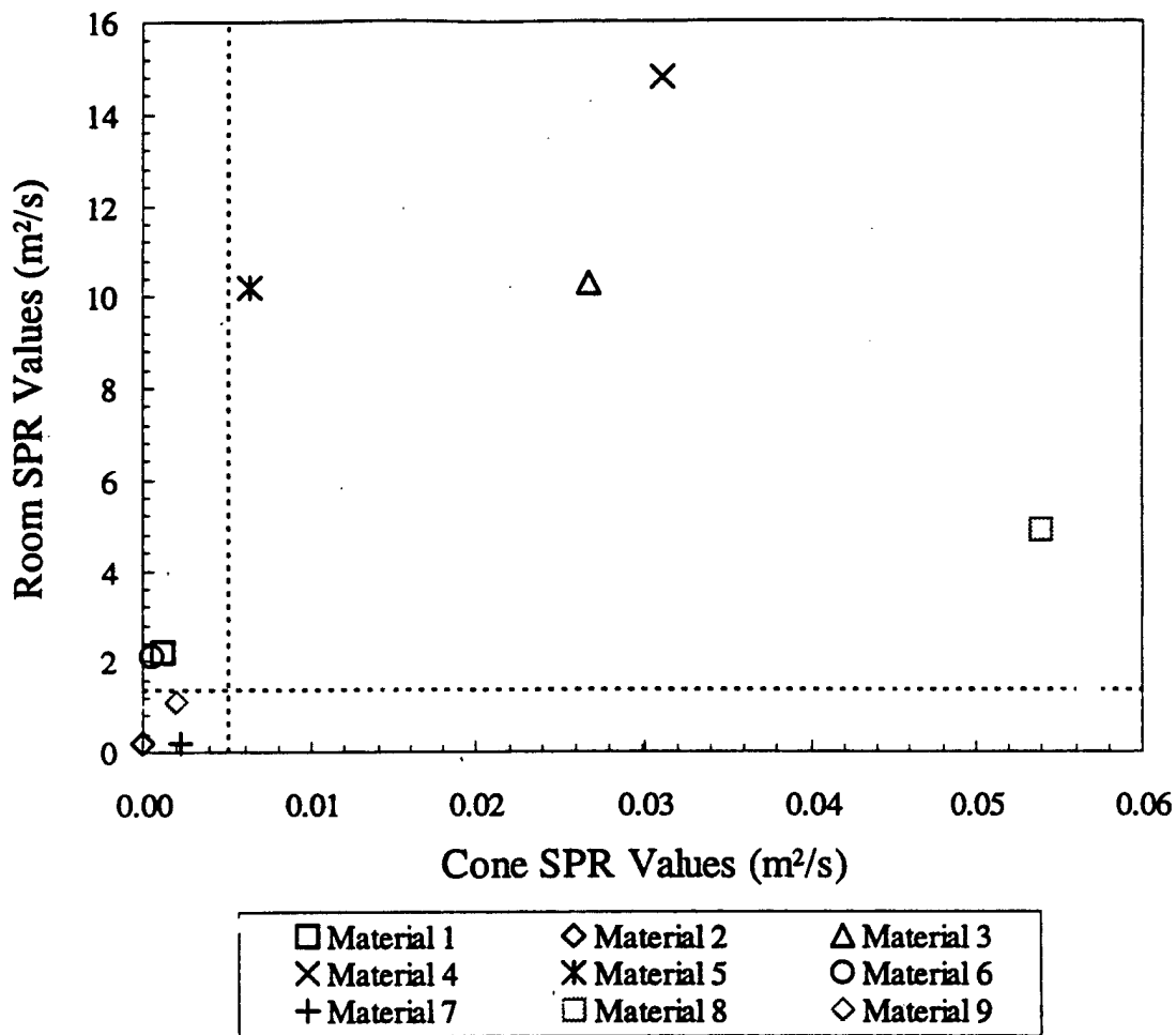
Figure 8-3 – Correlation of Test-Average Smoke Production Rates
