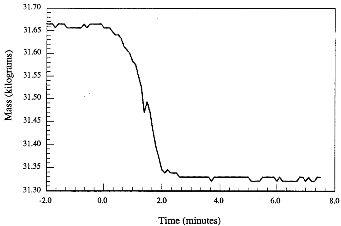
Figure 4.c - Material # 1 - Double chair - Mass vs. time
