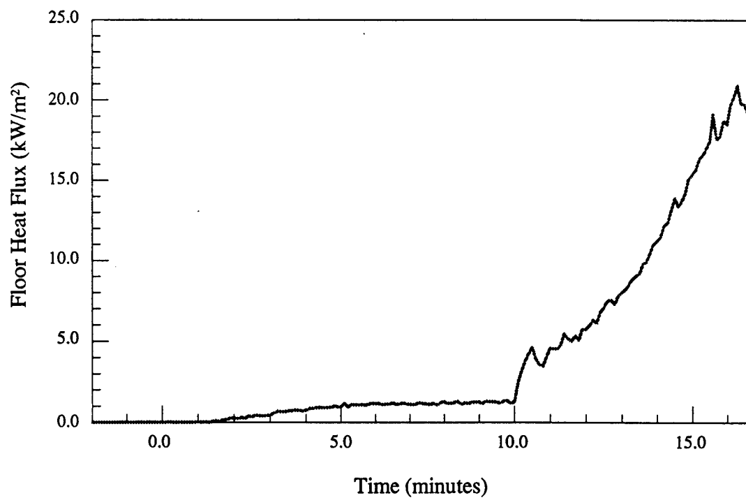
Figure 5.c - Material # 5 - Floor heat flux vs. time
