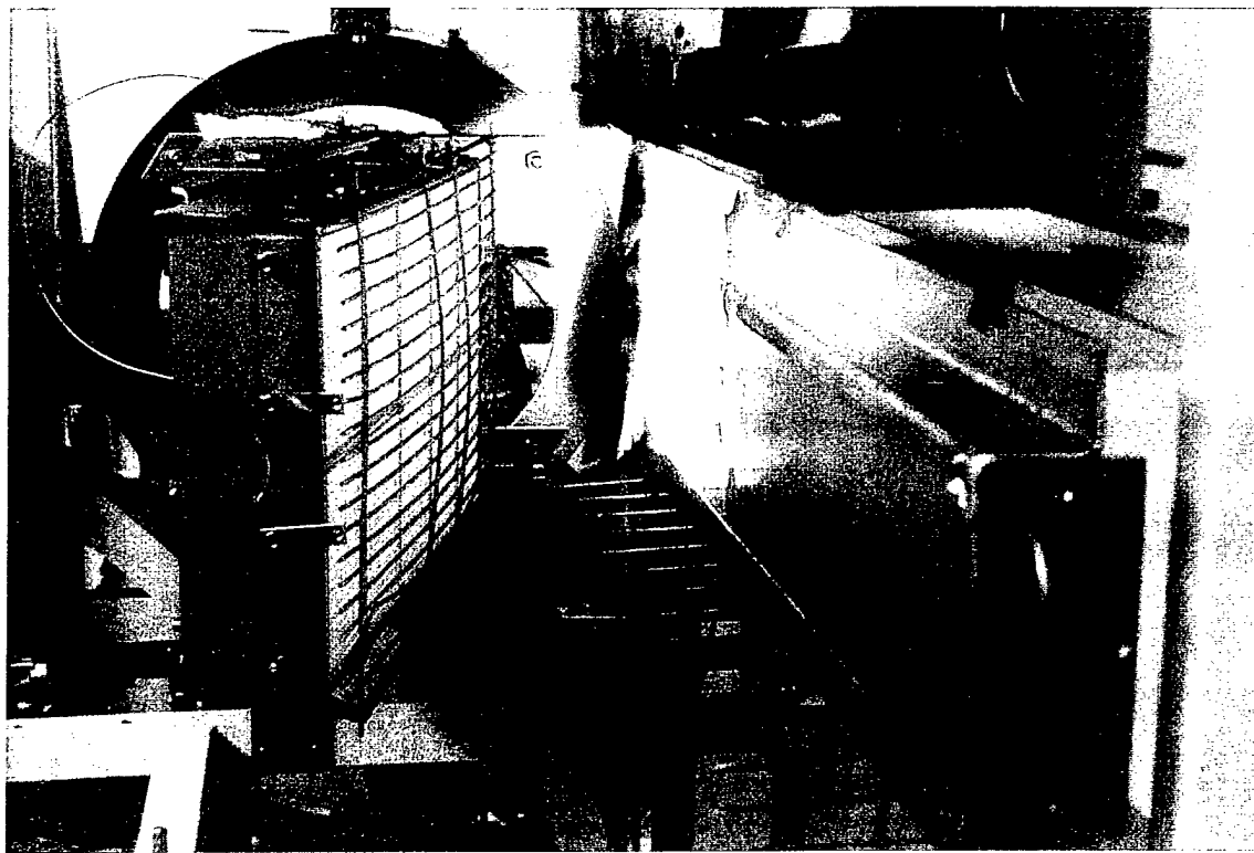
Figure 5. IMO Surface Flammability Test in Progress (Pilot Location Shown).
