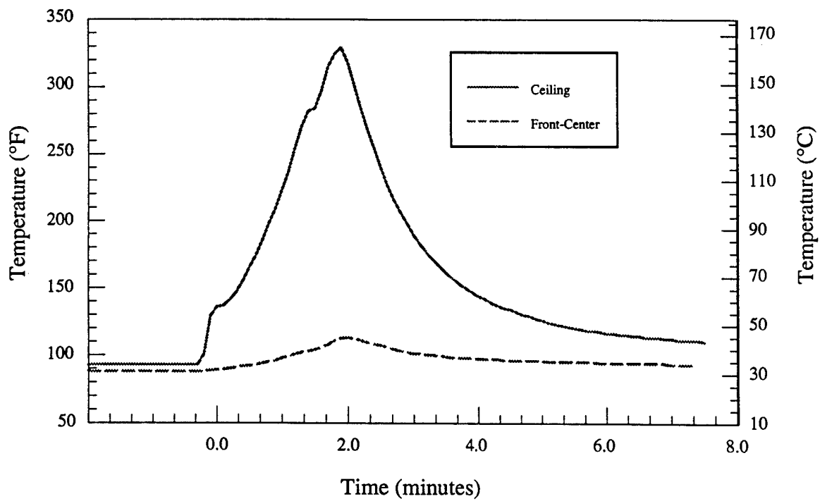
Figure 4.d - Material # 1 - Double chair - Room temperatures vs. time
