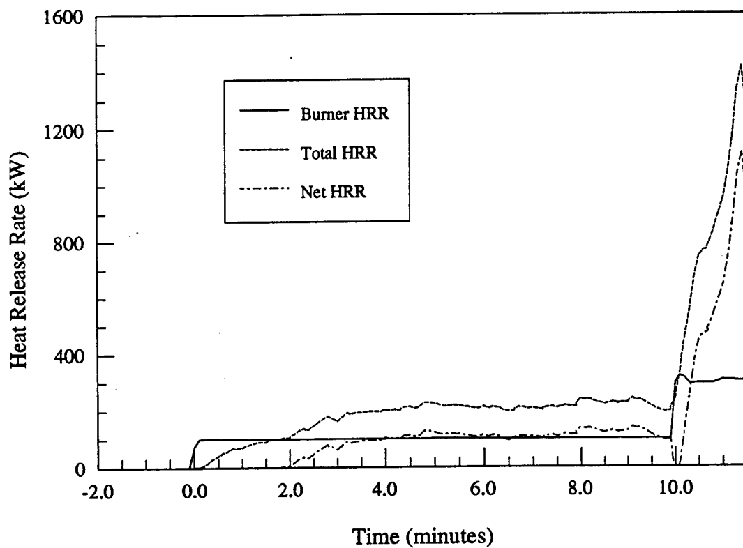
Figure 9.a - Material # 9 - Heat release rate vs. time
