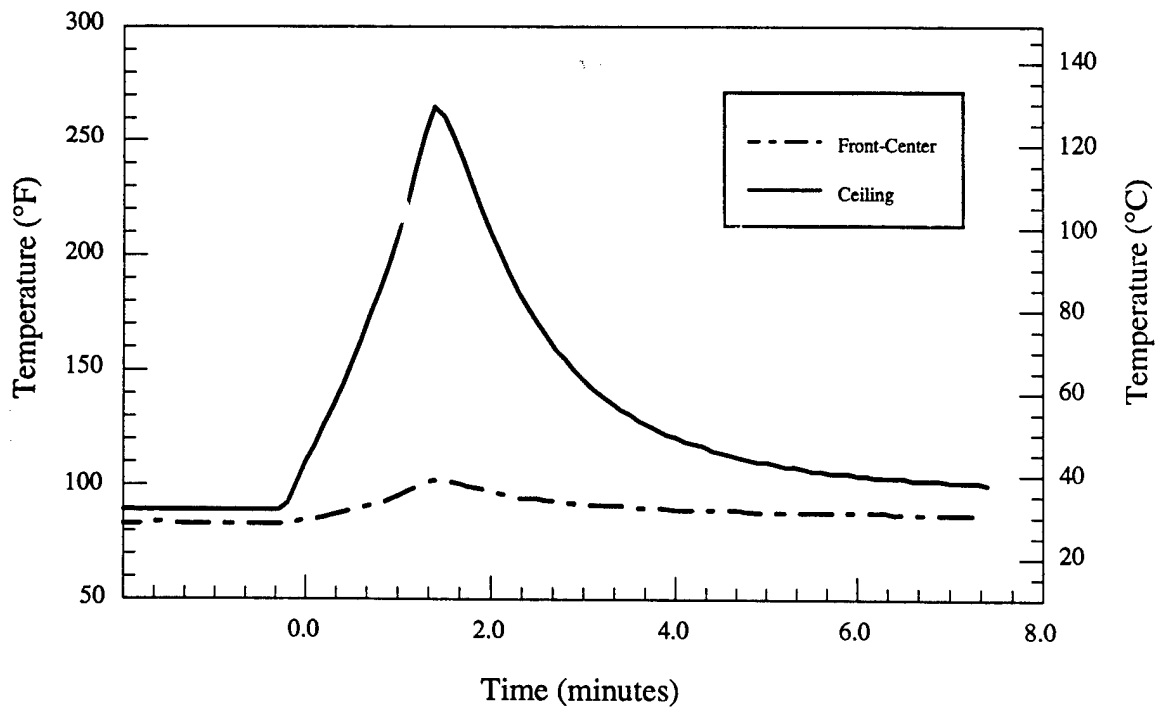
Figure 6.d - Material # 4 - Single chair - Room temperatures vs. time
