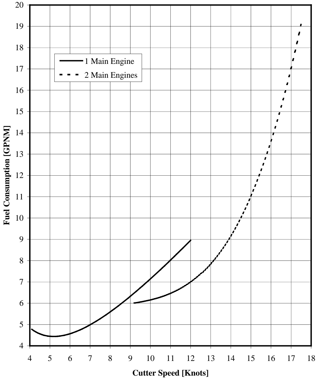
Figure 2-2. Optimum transit speed (includes SSDG and auxiliary boiler fuel consumption) USCGC RESOLUTE (WMEC 620).
