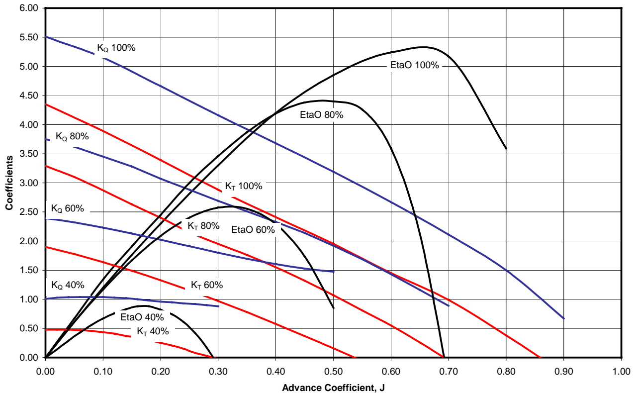
Figure B-5. WLB 225' propeller characteristics (60% pitch interpolated) 10 \times K_T , 100 \times K_Q , 10 \times \text{Eta}_O .
