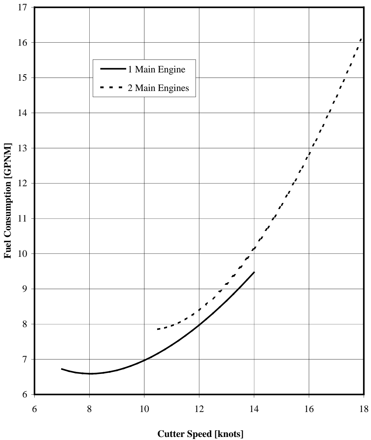
Figure 2-6. Optimum transit speed (includes SSDG fuel consumption) USCGC TAHOMA (WMEC 908).
