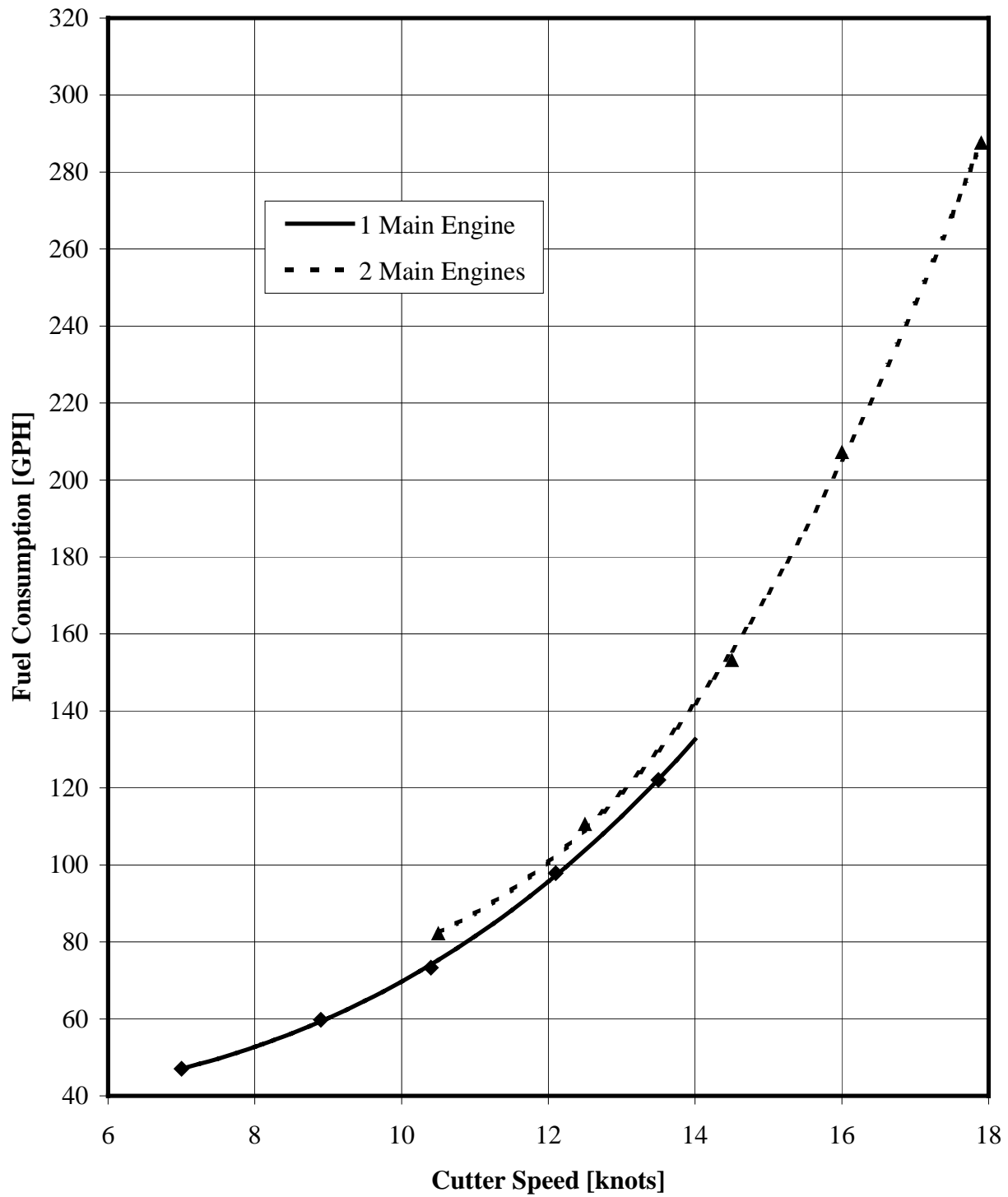
Figure 2-5. Fuel consumption versus speed (includes SSDG fuel consumption) USCGC TAHOMA (WMEC 908).
