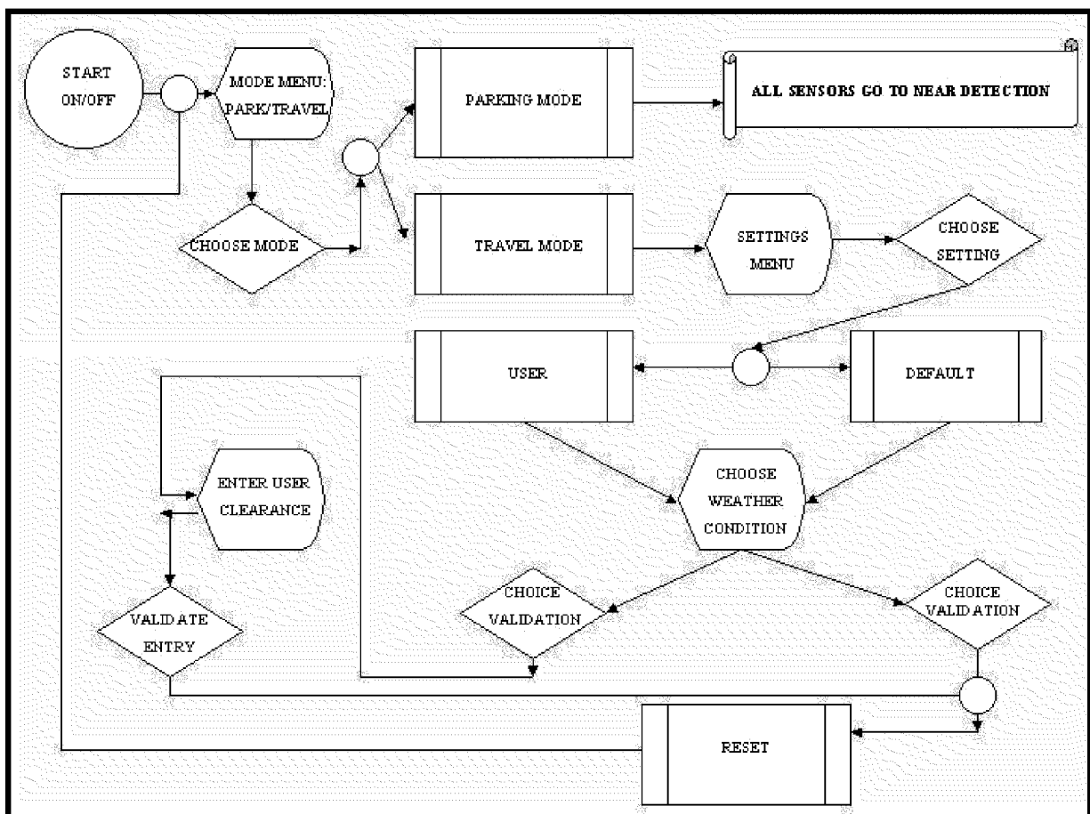
Figure 15. AVAILS-HCI Flowchart
