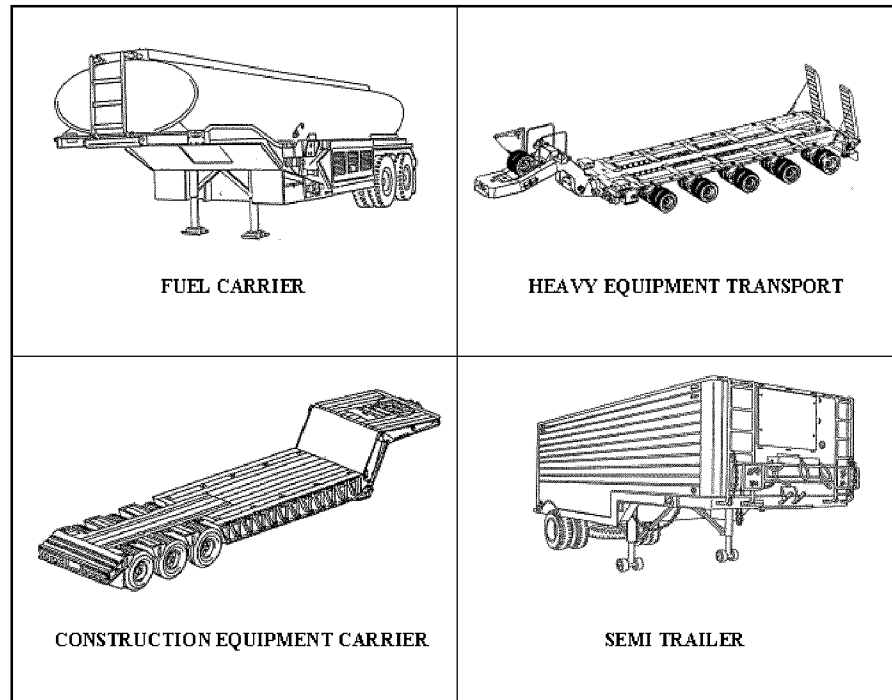
Figure 4. Trailers (From: [21])
