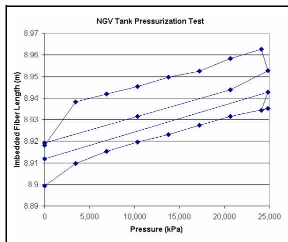
Figure 4. Plot of the Measured Fiber Length During the Tank Pressurization Test
