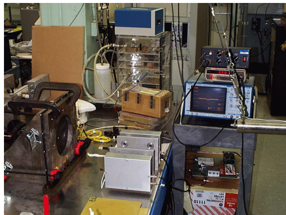
Figure 2. Ram Impact Experimental Set-up
