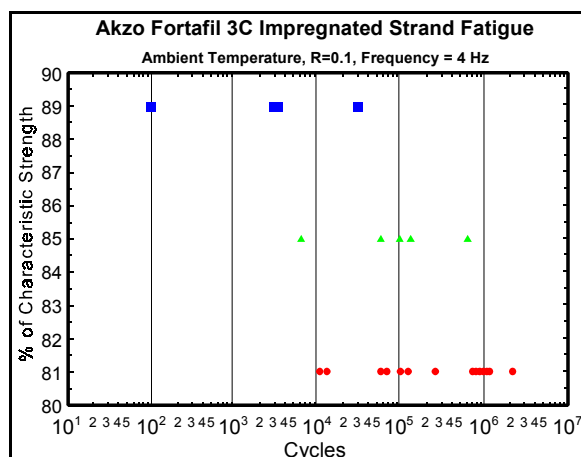
Figure 2. Large Tow-Size Carbon Fiber Strand Fatigue Data
