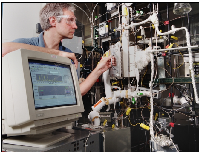
Argonne National Laboratory Microreactor for Testing Fuels
