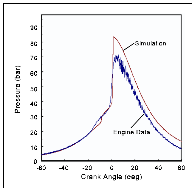
Lawrence Livermore National Laboratory HCCI Combustion Model Results
