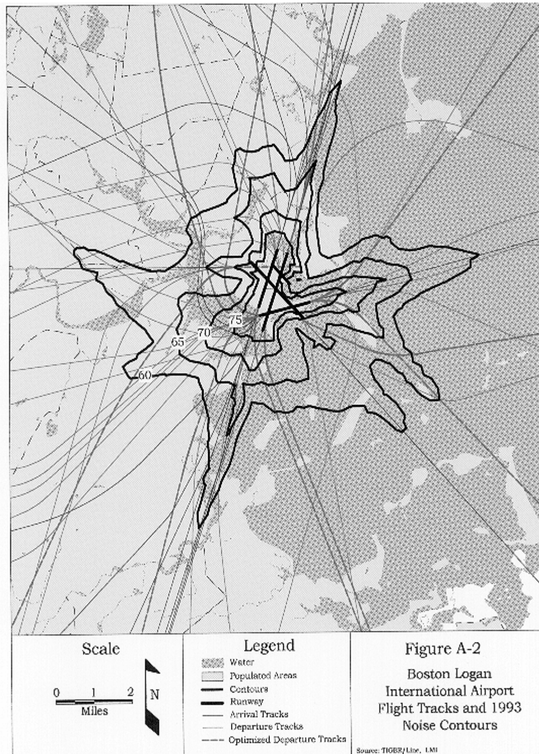
Figure A-2. Boston Logan International Airport Flight Tracks and 1993 Noise Contours
