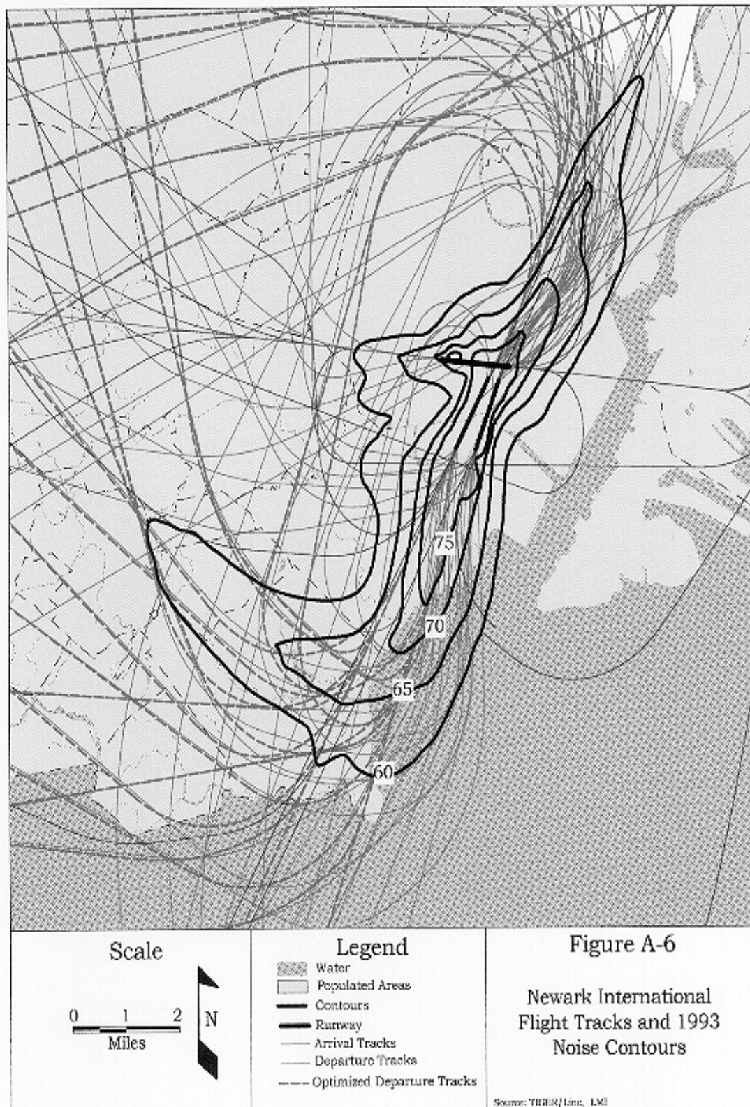
Figure A-6. Newark International Airport Flight Tracks and 1993 Noise Contours
