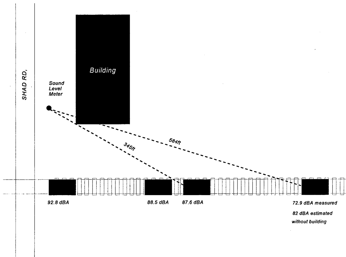
Figure 1. Effect of a Building on the Measured Sound Level During a Locomotive Pass-by
