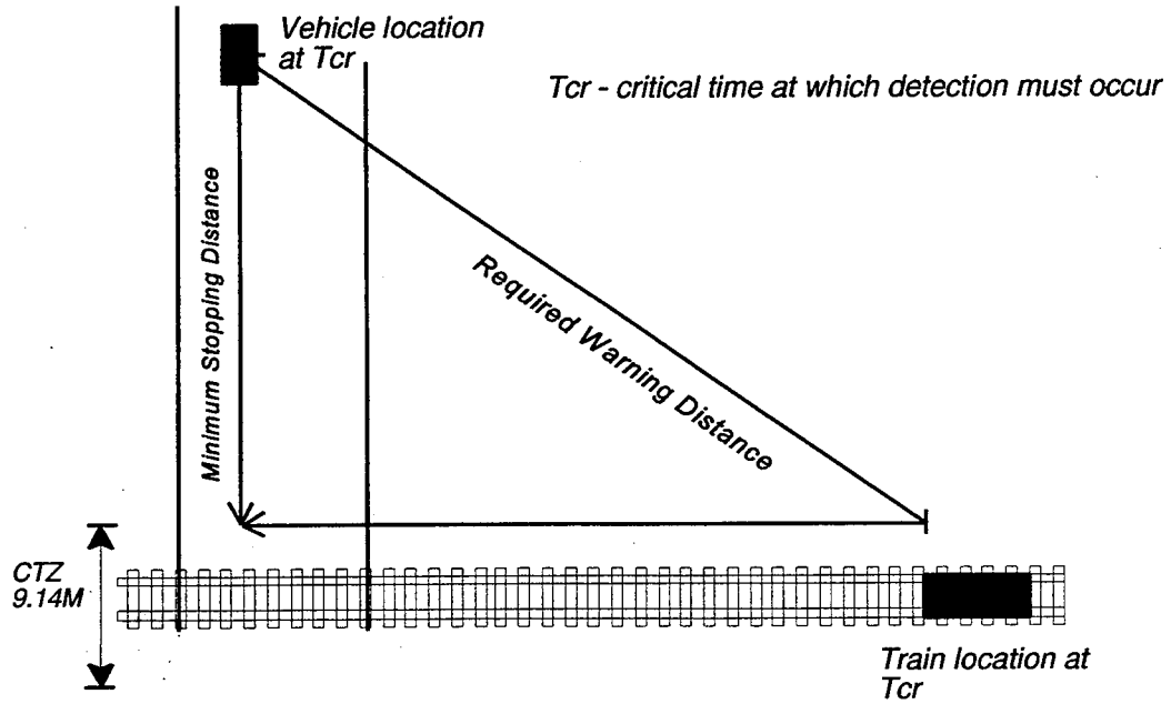
Figure 5. Required Warning Distance
