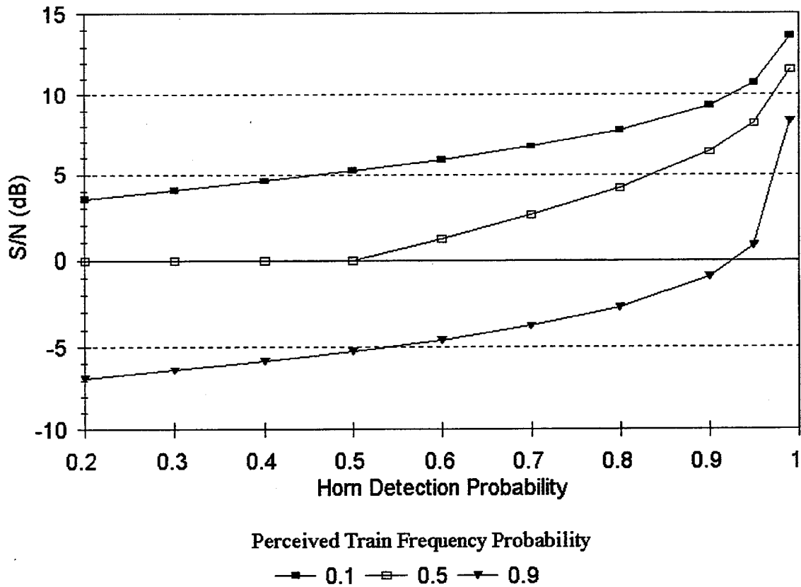
Figure 4. Horn Detection Probability vs. S/N
