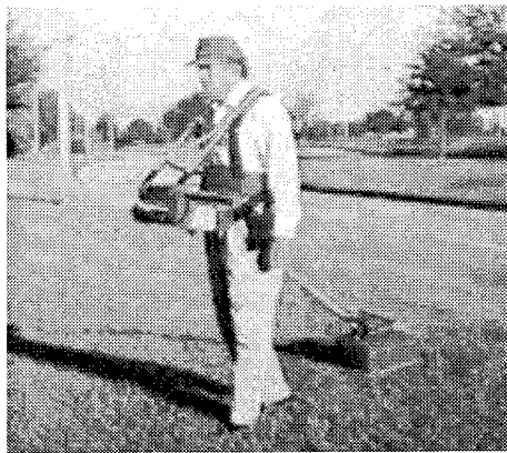
Figure 10. Hand-Pulled GPR.
