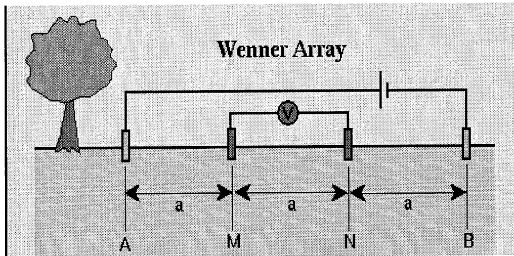
Figure 6. Wenner Array (18).
