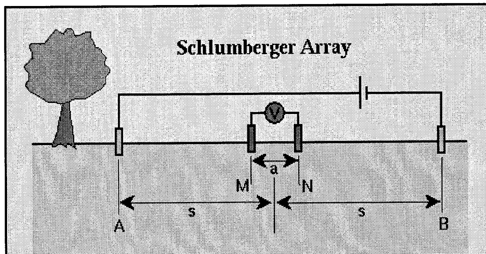
Figure 7. Schlumberger Array (18).
