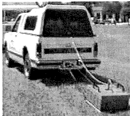
Figure 11. Truck-Pulled GPR.
