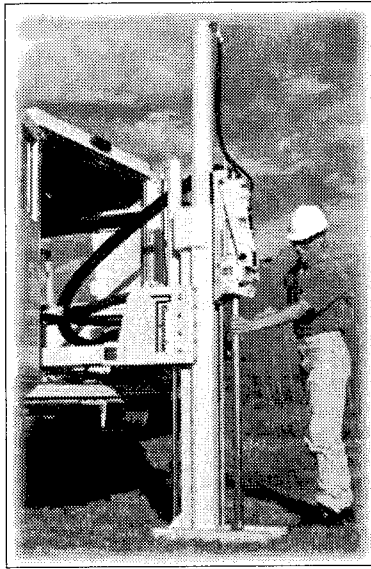
Figure 14. Truck-Mounted Geoprobe (20).
