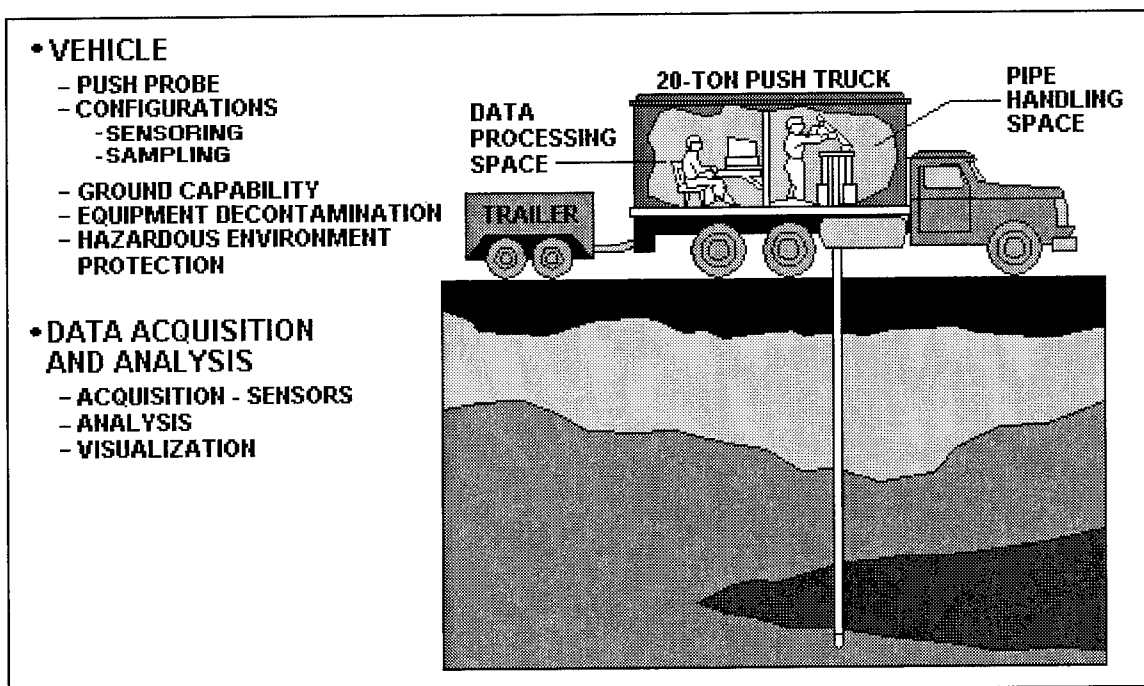
Figure 15. CPT Diagram (16).
