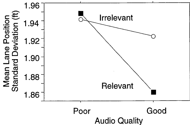
Figure 19. Mean lane position standard deviation for message quality by relevance interaction.
