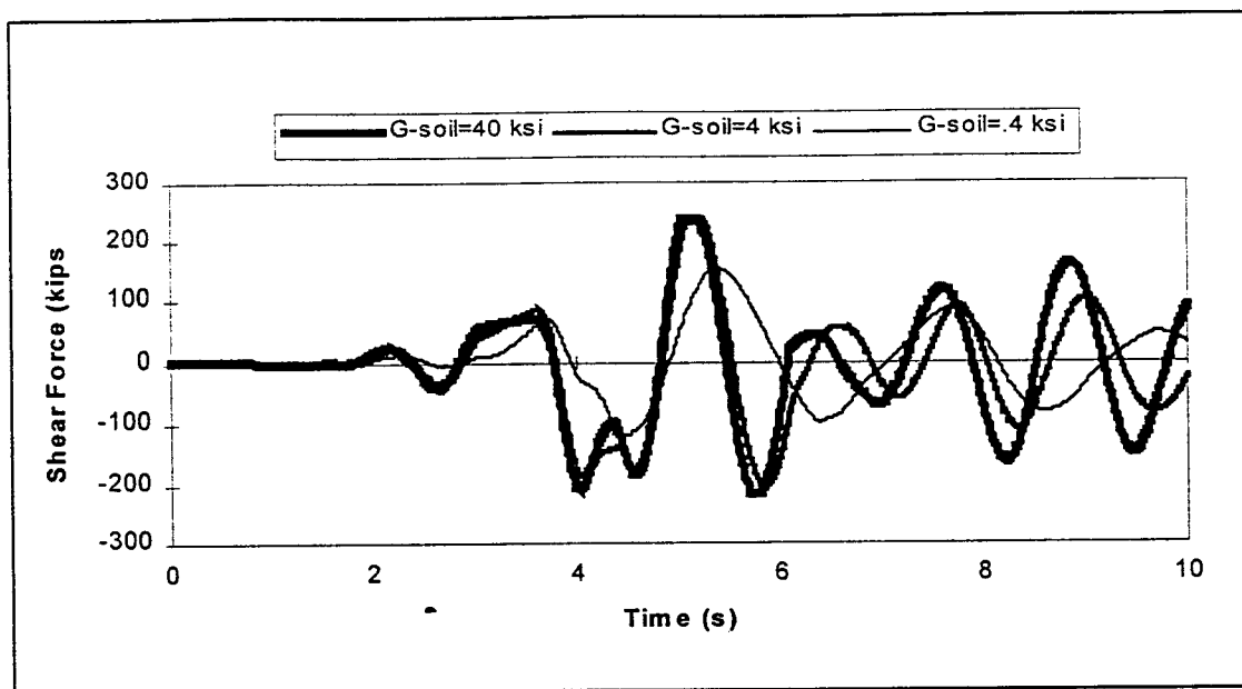
Figure 7-8 Shear force time histories for Clements Bridge, pier #1. Different soil shear moduli under Parkfield earthquake. (2-D model, \mu=0.6 at bearings, \text{PGA}=0.18g ).
