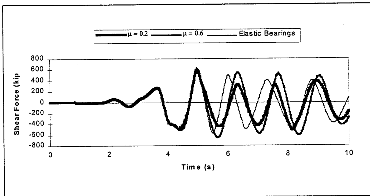
Figure 7-15 Shear force time histories for Alexander Bridge pier. Different bearing frictional coefficients under Parkfield earthquake. (2-D model, G\text{-soil}=4 ksi, \text{PGA}=0.18g )
