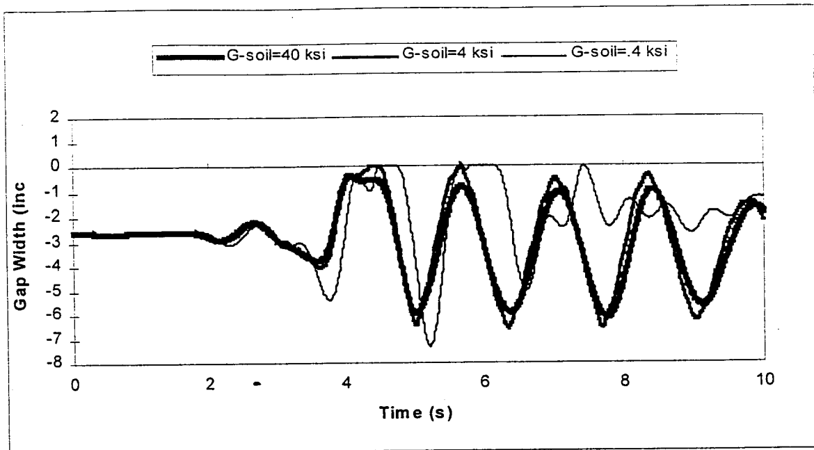
Figure 7-14 Gap width time histories for Alexander Bridge, abutment #1. Different soil shear moduli under Parkfield earthquake. (2-D model, \mu=0.6 at bearings, \text{PGA}=0.18g ).
