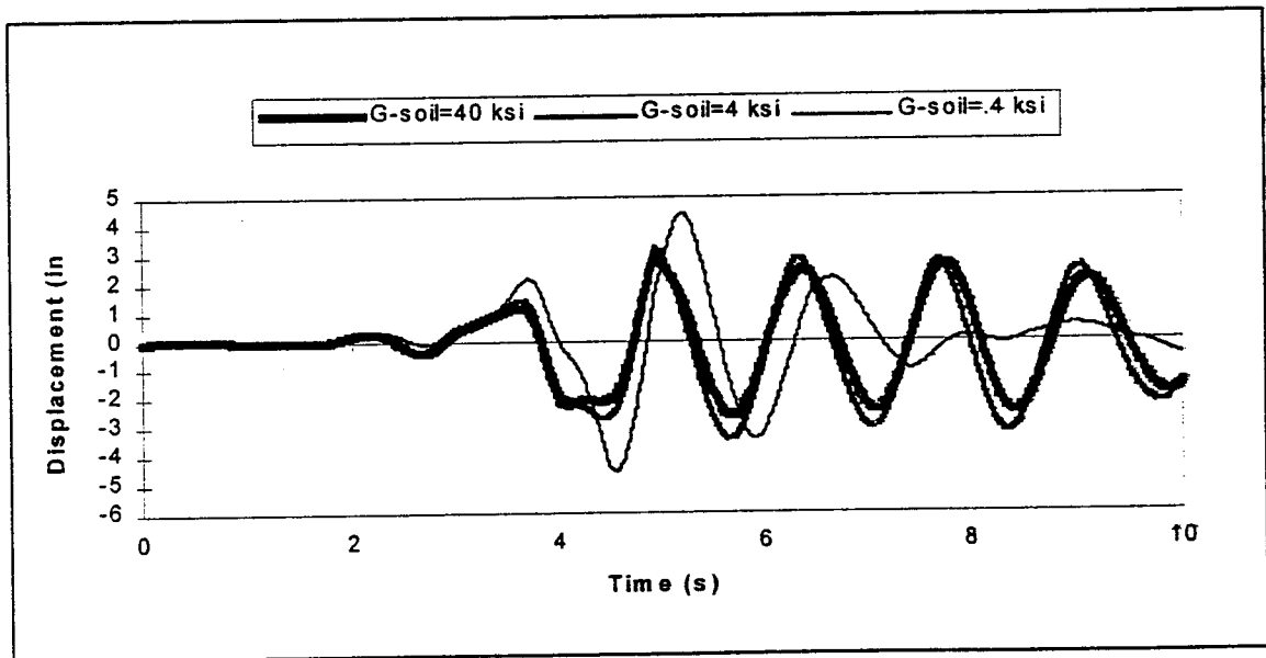
Figure 7-13 Top displacement time histories for Alexander Bridge pier. Different soil shear moduli under Parkfield earthquake. (2-D model, \mu=0.6 at bearings, \text{PGA}=0.18g ).
