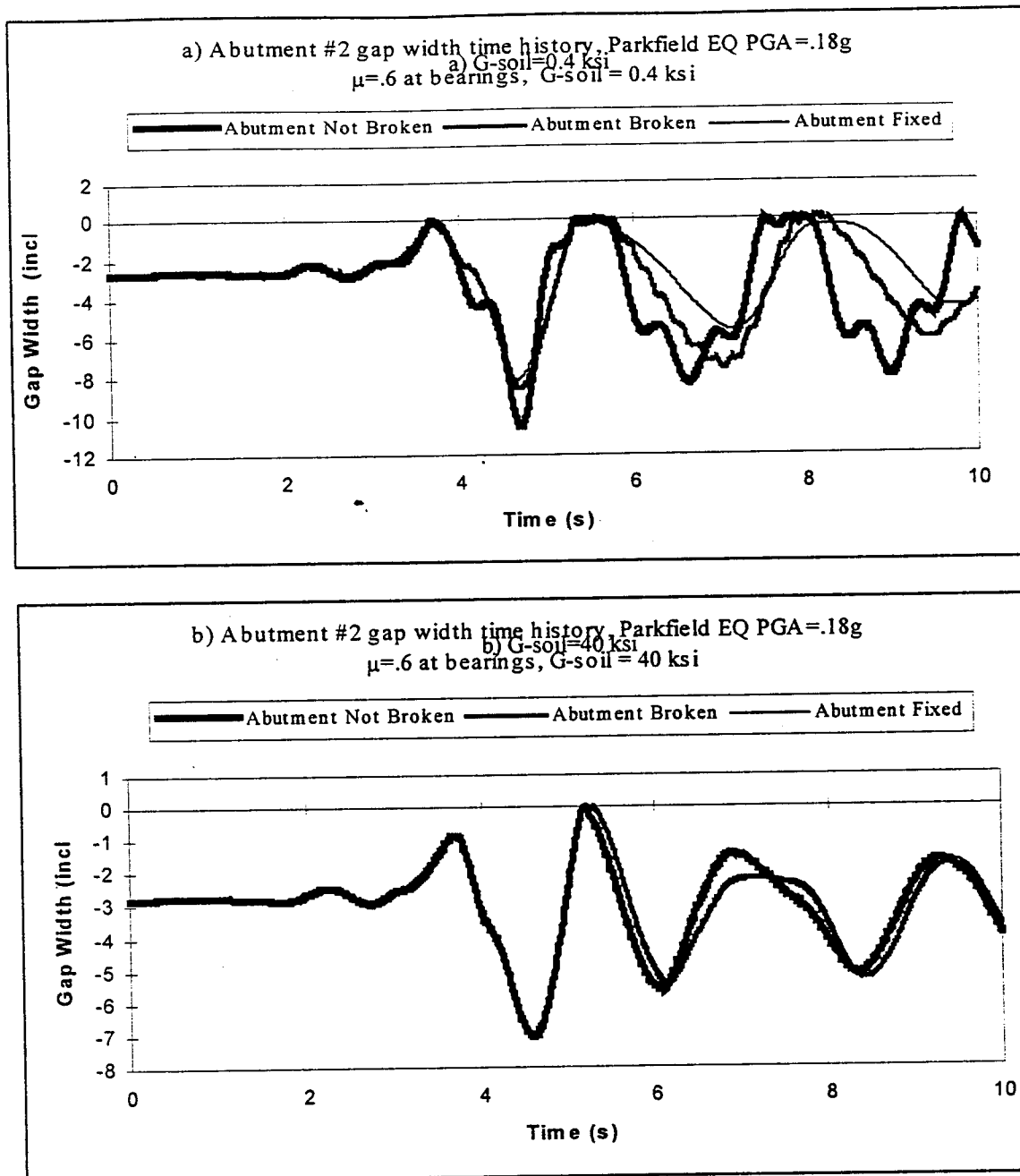
Figure 7-11 Gap width time histories for Clements Bridge abutment #2. Different SSI models under Parkfield earthquake (2-D model, \mu=0.6 at bearings, PGA=0.18g).
