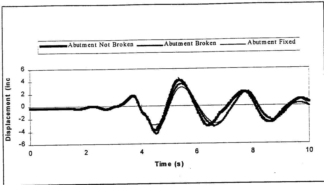
Figure 7-12 Top displacement time histories for Clements Bridge, pier #1. Different abutment models under Parkfield earthquake. (2-D model, \mu=0.6 at bearings, G_{\text{soil}} = 0.4 ksi, \text{PGA}=0.18g ).
