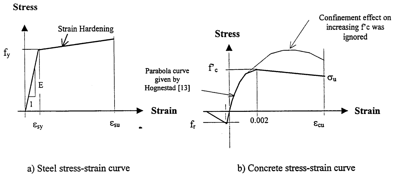
Figure 4-1 Stress-strain curves for steel and concrete
