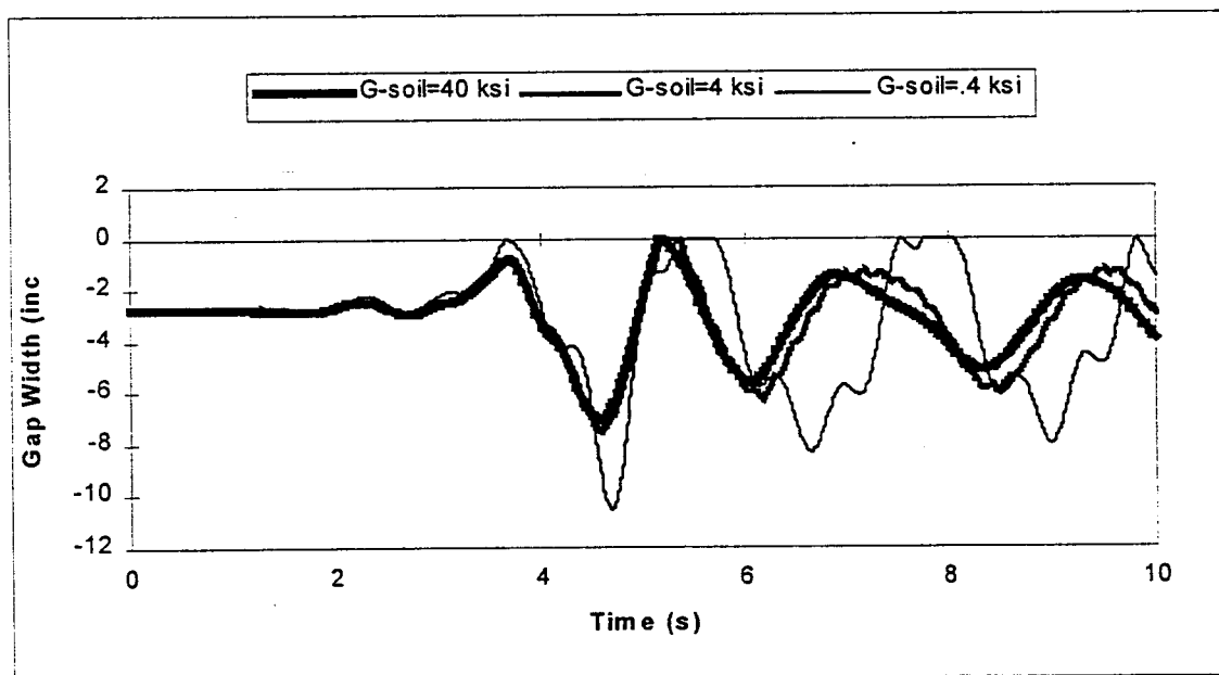
Figure 7-9 Gap width time histories for Clements Bridge, abutment #2. Different soil shear moduli under Parkfield earthquake (2-D model, \mu=0.6 at bearings, \text{PGA}=0.18g ).
