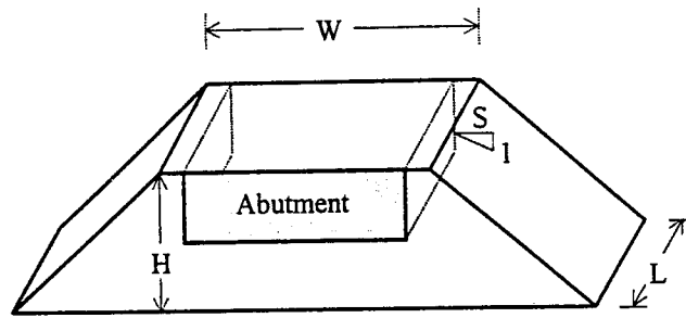
Figure 3-6 Abutment embankment dimensions used in calculating transverse and vertical stiffnesses
