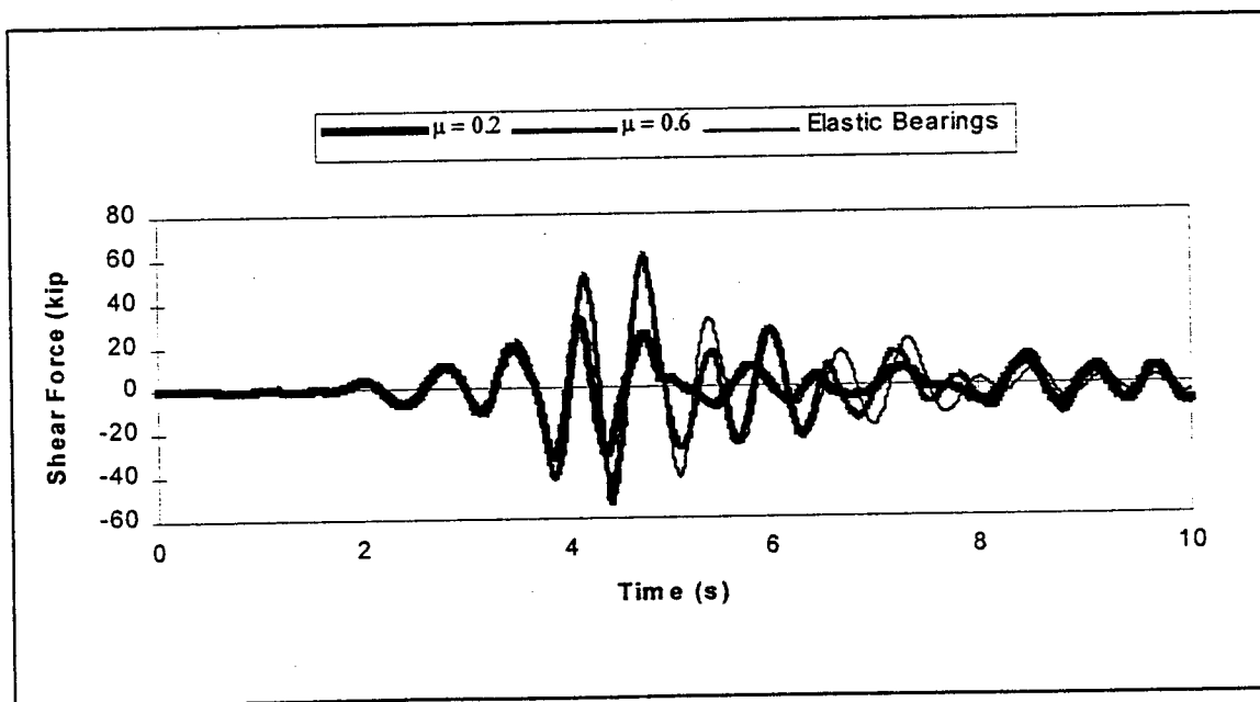
Figure 7-20 Bridge-5 shear force time histories for pier #1, column type-3. Different bearing frictional coefficients under Parkfield earthquake. (2-D model, G-soil=4 ksi, PGA=0.18g)
