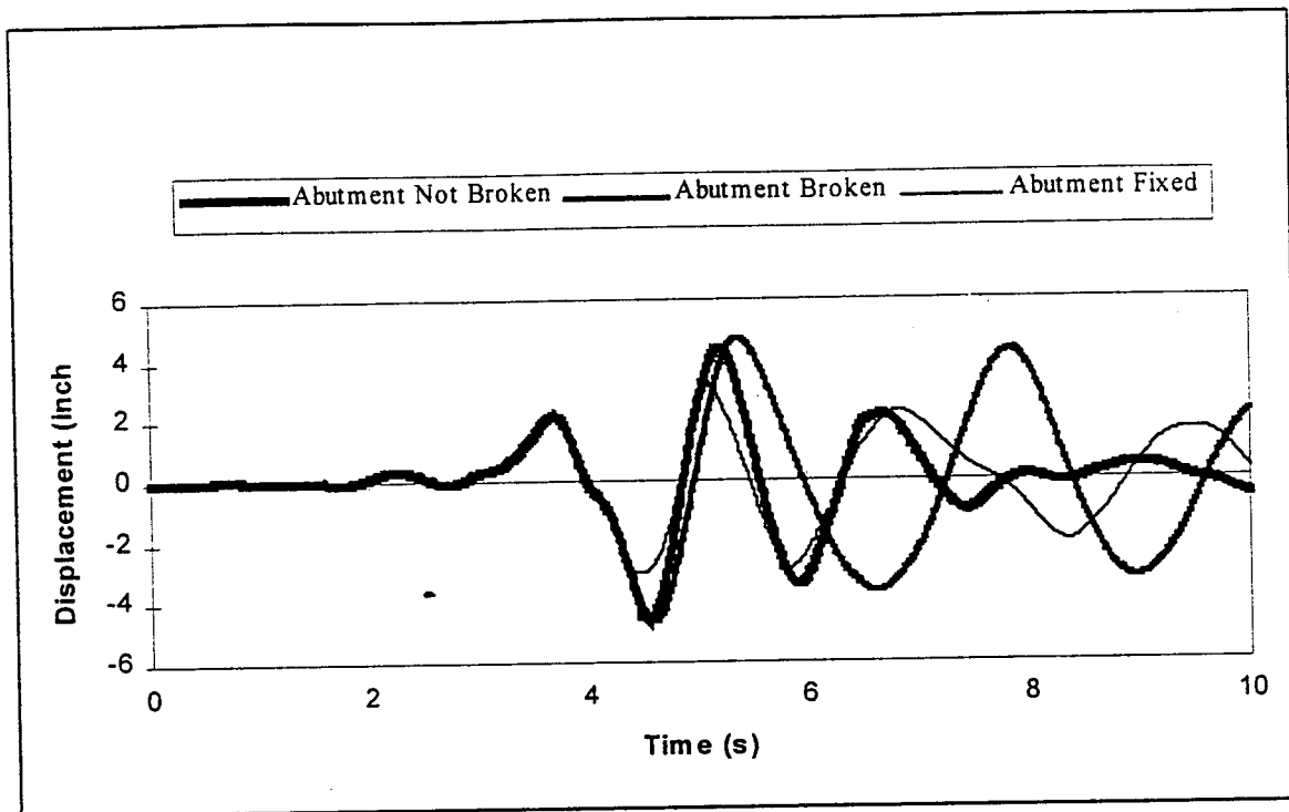
Figure 7-17 Top displacement time histories for Alexander Bridge pier. Different abutment models under Parkfield earthquake. (2-D model, \mu=0.6 at bearings, G_{\text{soil}} = 0.4 ksi, \text{PGA}=0.18g )
