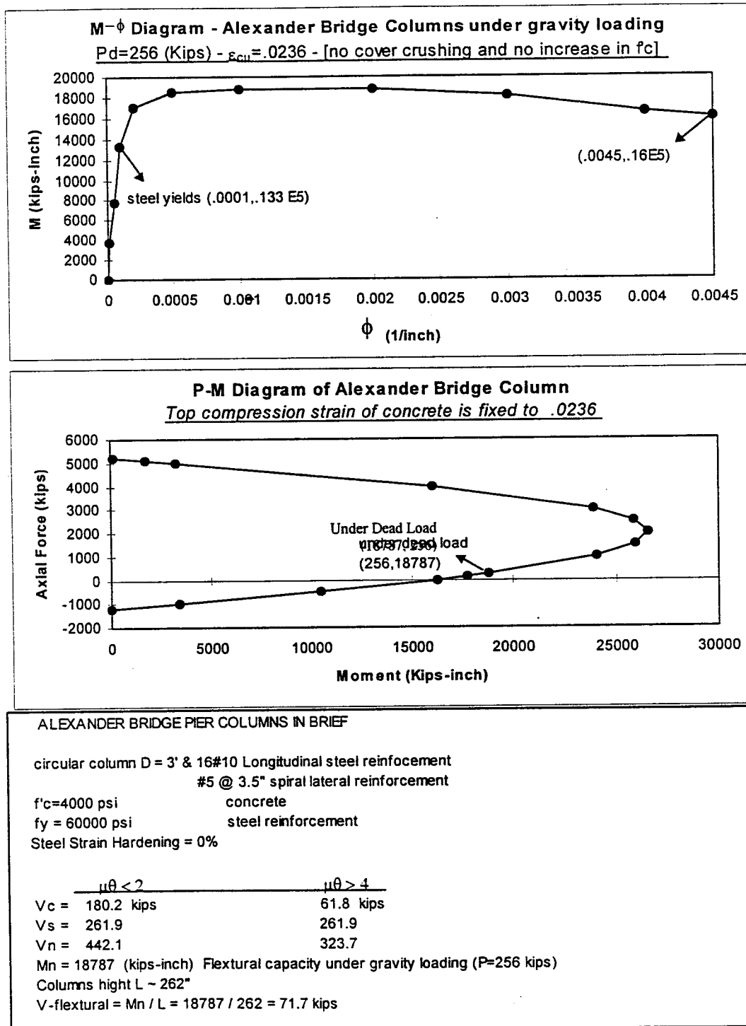
Figure 4-3 Capacity of Alexander Bridge pier column
