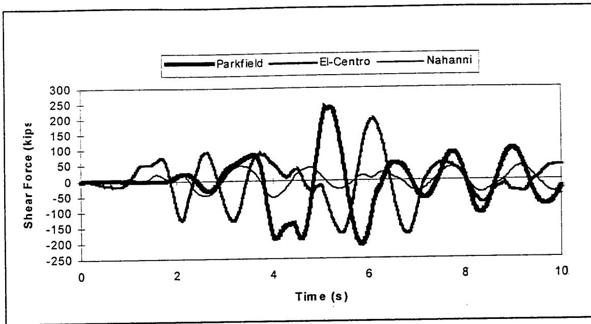
Figure 7-3 Clements Bridge shear force time histories of Pier #1 columns (2 columns) for three earthquake records with PGA of 0.18g (2-D model, \mu=0.6 at bearings, G_{soil}=4 ksi).
