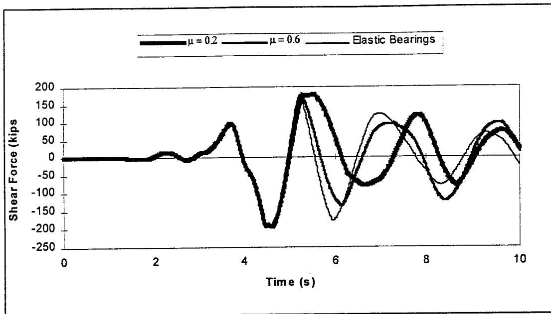
Figure 7-10 Shear time histories for Clements Bridge, pier #2. Different bearing frictional coefficients under Parkfield earthquake. (2-D model, G-soil=4 ksi, PGA=0.18g).
