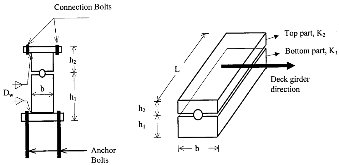
Figure 2-5 Fixed bearing general shape and components
