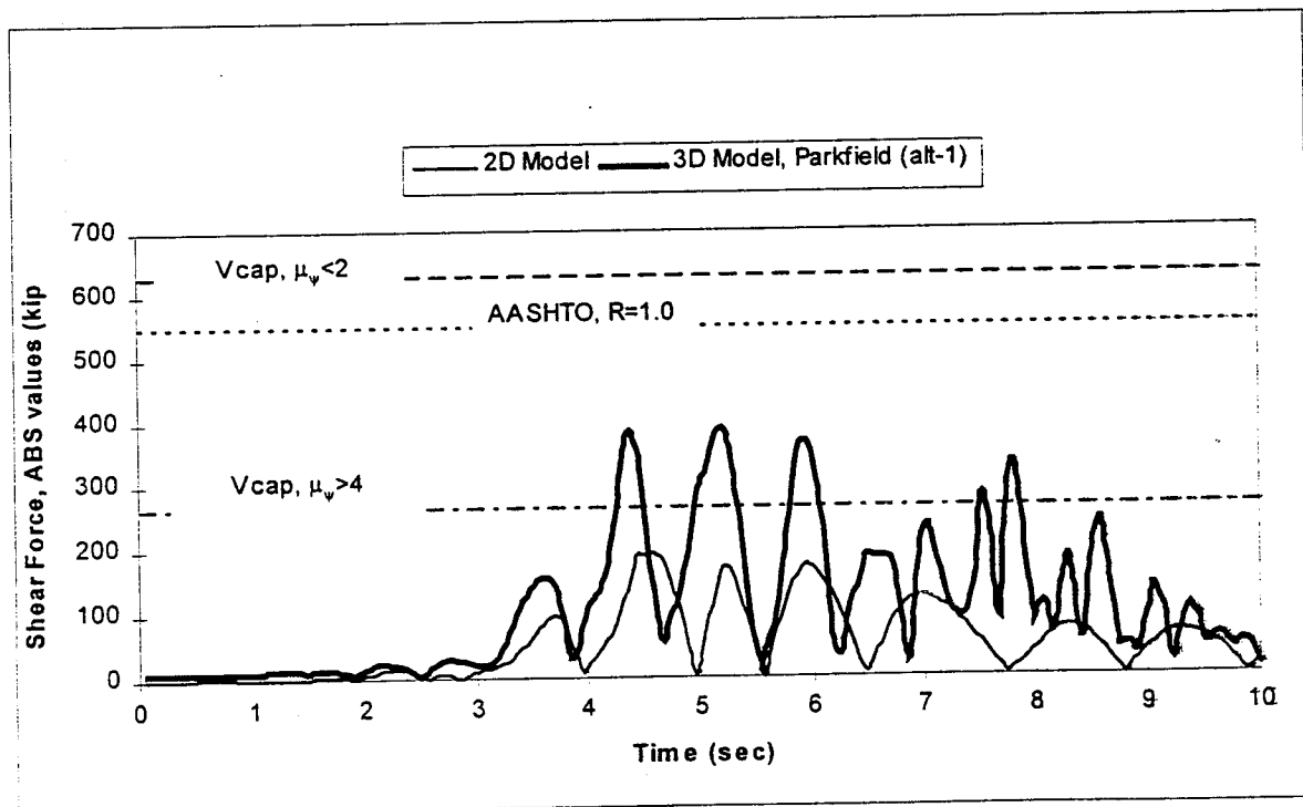
Figure 8-3 Pier column shear time history comparison of Clements Bridge for 2-D and 3-D models (Parkfield (alt-1) record, G-soil=4 ksi, Elastic bearings)
