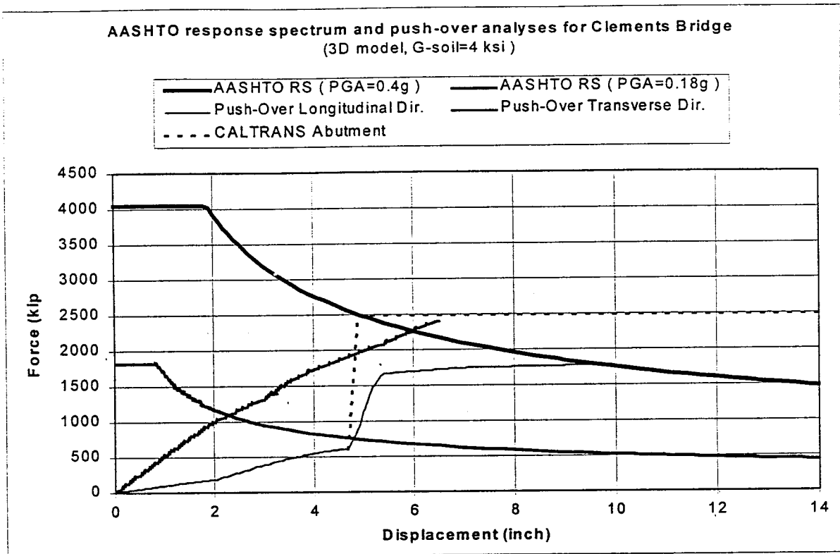
Figure 8-4 Push over analyses for Clements Bridge (3-D model, G-soil=4 ksi)
