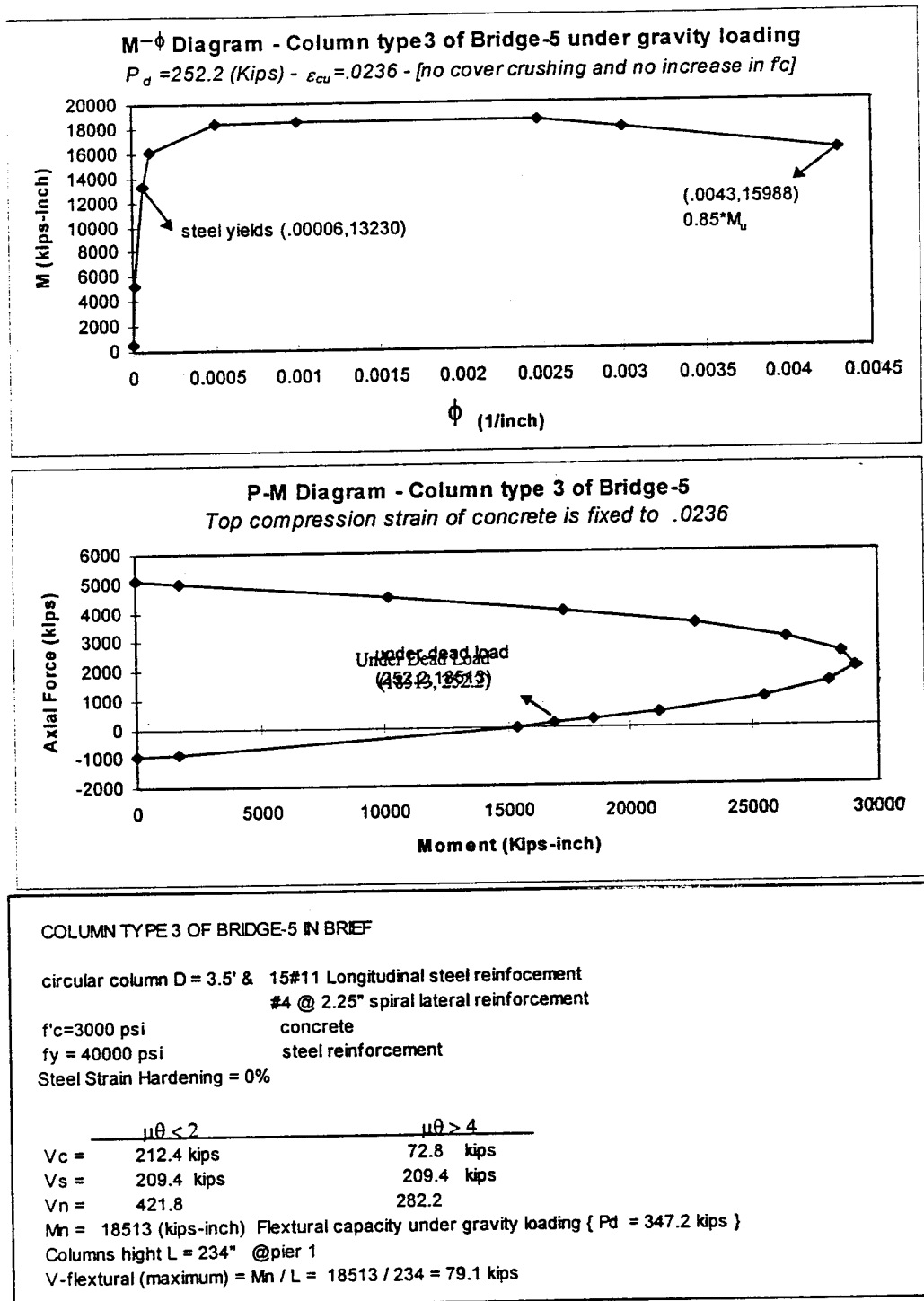
Figure 4-6 Capacity of column type-3 from Bridge-5
