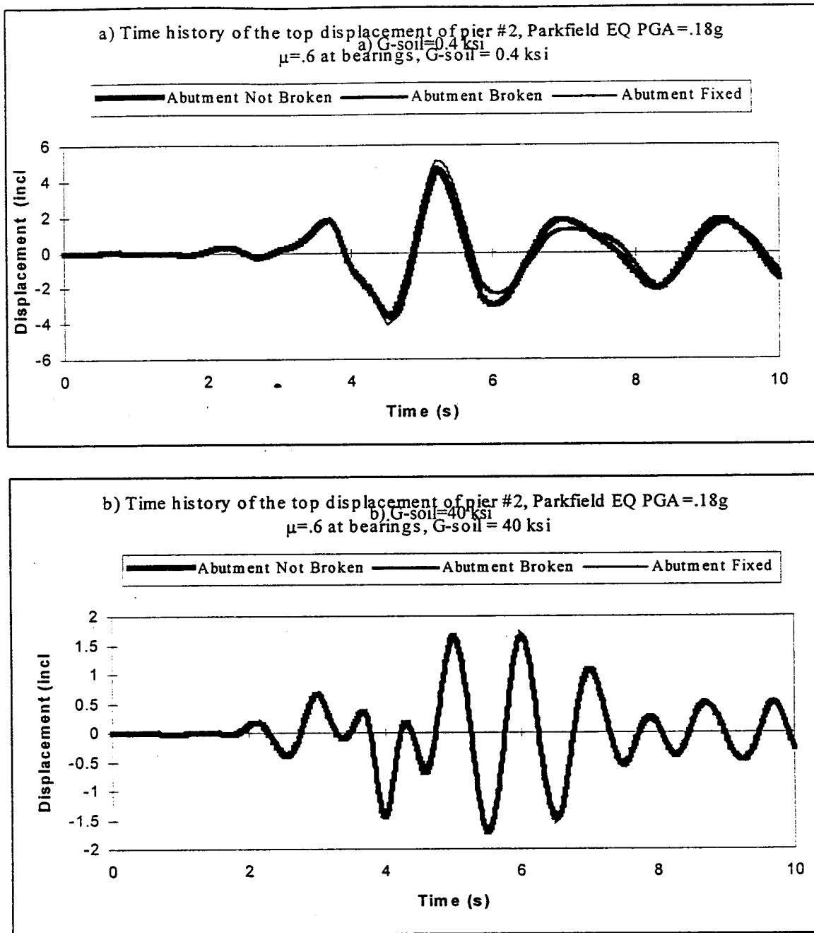
Figure 7-21 Top displacement time histories for Bridge-5, pier #2. Different SSI models under Parkfield earthquake. (2-D model, \mu=0.6 at bearings, PGA=0.18g)
