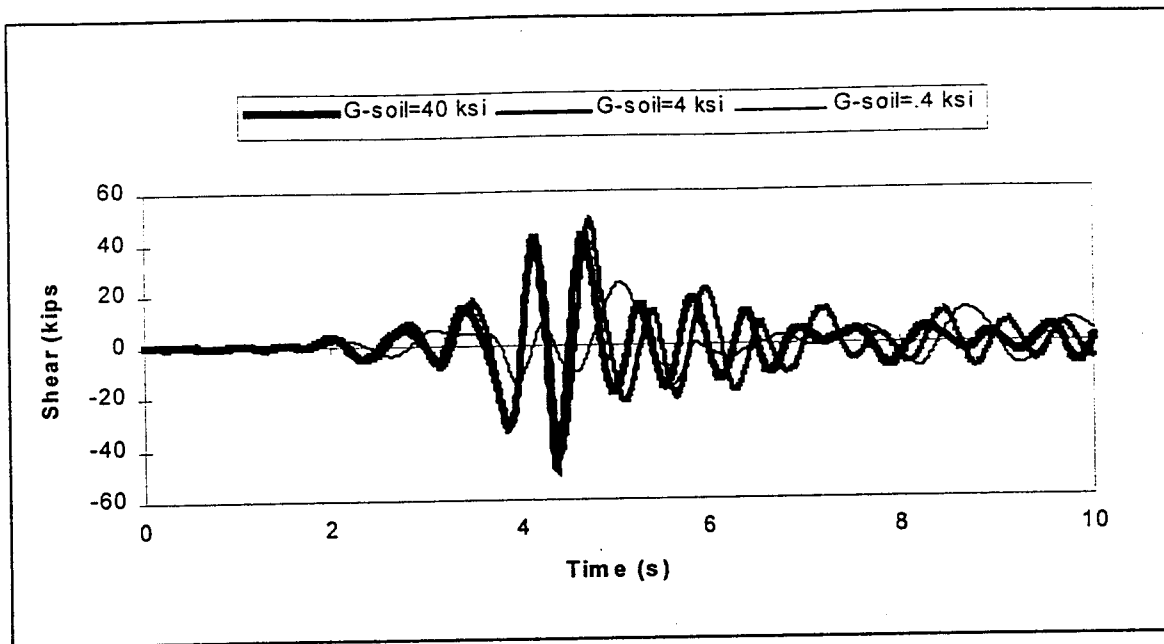
Figure 7-19 Bridge-5 shear time histories for pier #1, column type-1. Different soil shear moduli under Parkfield earthquake. (2-D model, \mu=0.6 at bearings, PGA=0.18g).
