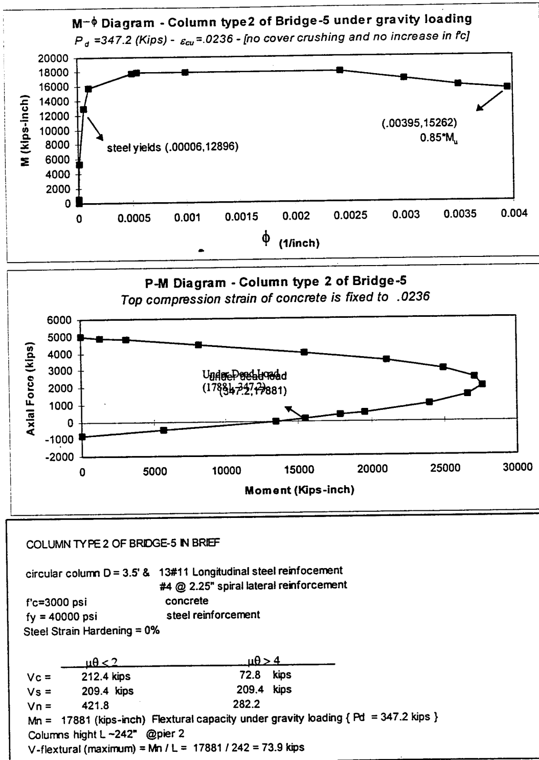
Figure 4-5 Capacity of column type-2 from Bridge-5
