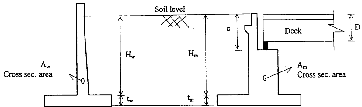
a) Typical wing wall section
