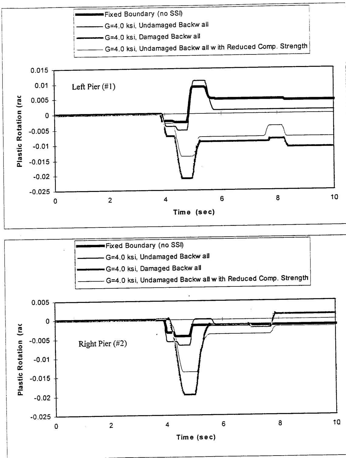
Figure 7-7 Time histories of plastic rotation at the base of pier columns in Clements Bridge abutment for various SSI models under Parkfield record scaled to 0.4g PGA (2-D model, elastic bearings)
