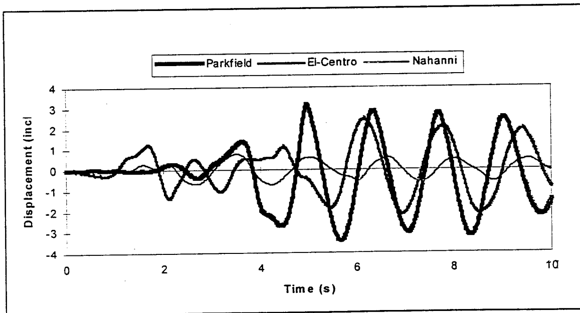
Figure 7-4 Alexander Bridge pier top displacement time histories for three earthquake records with PGA of 0.18g (2-D model, \mu=0.6 at bearings, G_{soil}=4 ksi).
