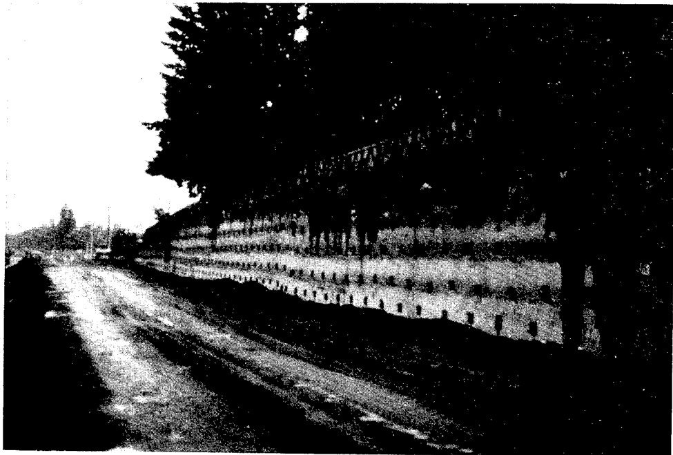
Figure A-2. Black Lake Interchange, WADOT Olympia, WA - Soil Nail Wall Construction
