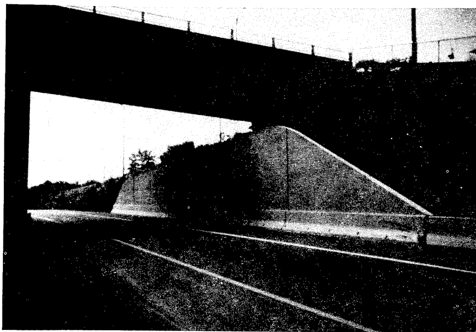
Figure A-5. I-5, WADOT Tacoma, WA - Soil Nail Wall in Tacoma (Bridge End Slope Removal)
