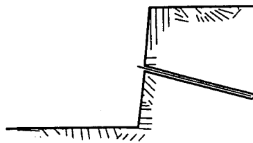
STEP 3. Install and Grout Nail
