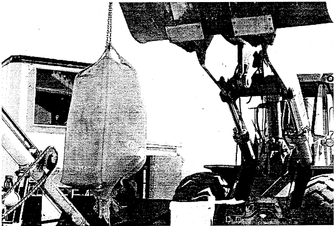
Figure 5. An overview of the crumb rubber system.
