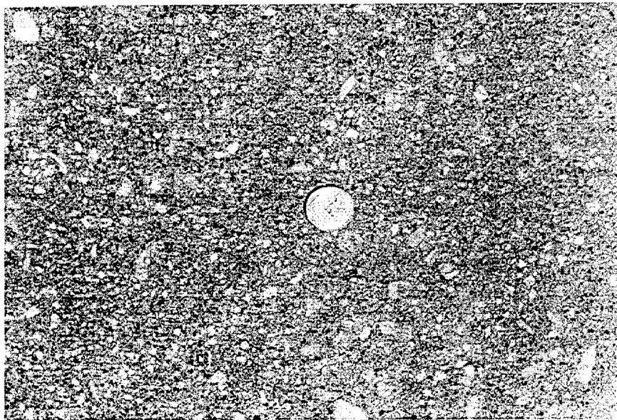
Figure 10. Surface of the 20 lb/ton. Notice the rubber particles on the surface.
