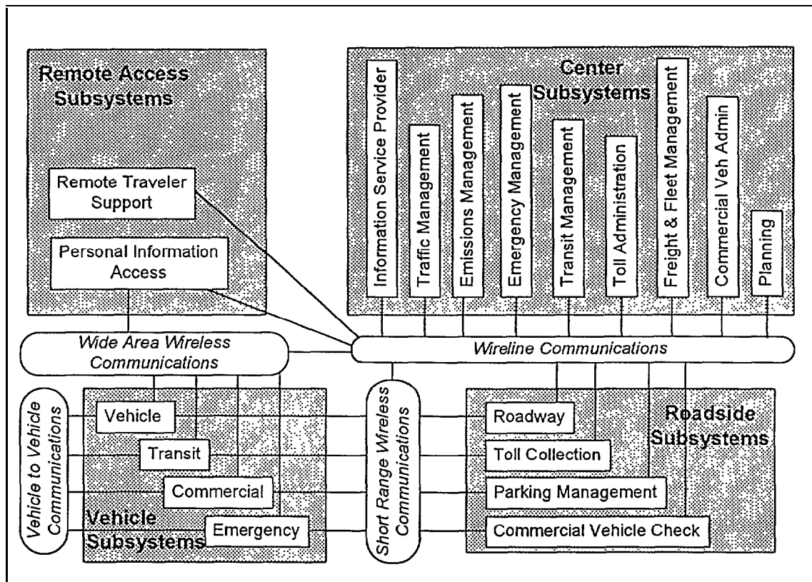
Figure 1: ITS Architecture Subsystems and Communications
