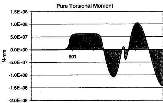
Figure 75: Straining actions for Br. 607 (Dead load)
