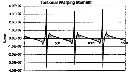
Figure 85: Straining actions for Br.538c (Dead load)
