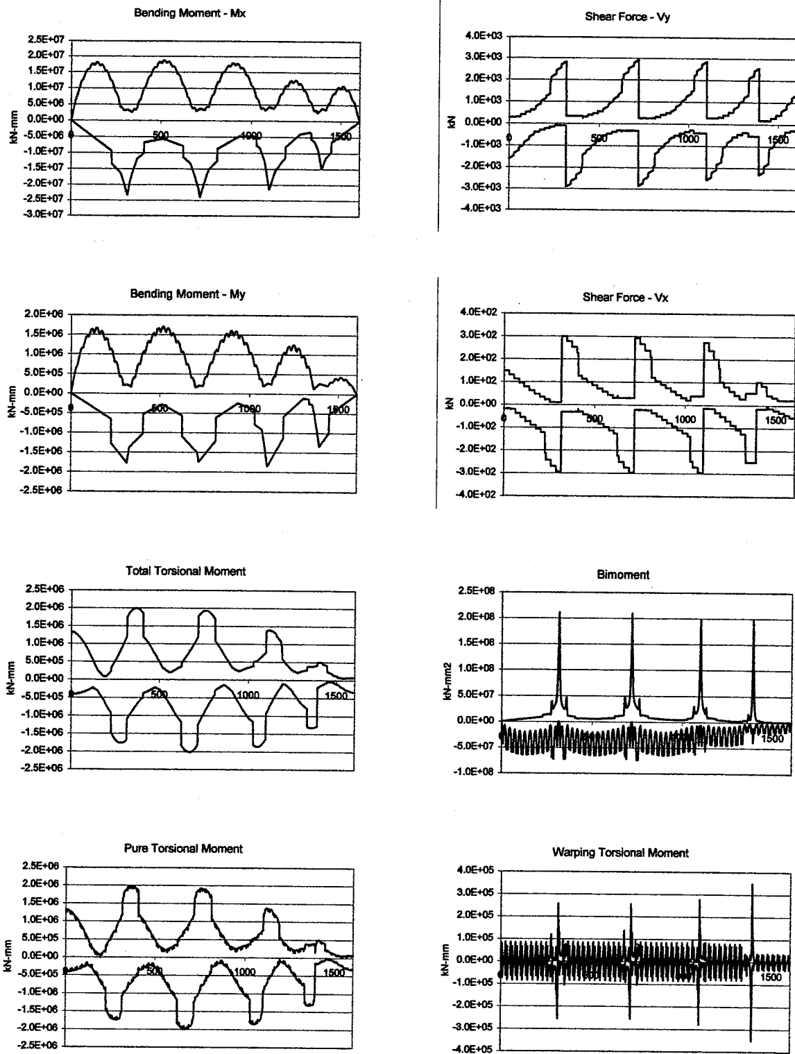
Figure 94: Straining actions for Br.541b (Live load envelope)
