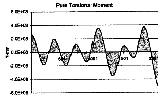
Figure 97: Straining actions for Br.542a (Dead load)
