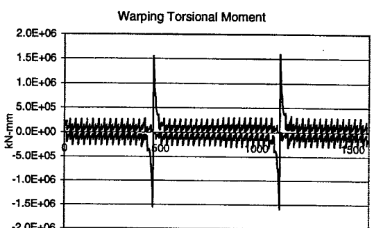
Figure 74: Straining actions for Br. 607 (Live load envelope)
