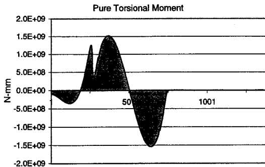
Figure 71: Straining actions for Br. 601 (Dead load)
