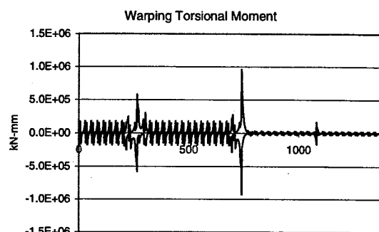
Figure 70: Straining actions for Br. 601 (Live load envelope)
