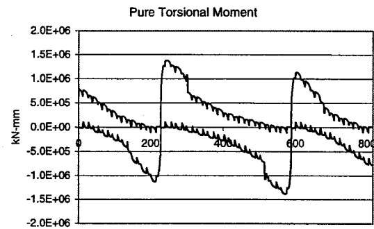
Figure 64: Straining actions for Br. 521 (Live load envelope)
