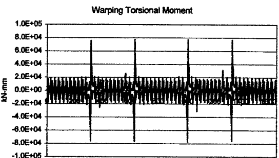
Figure 76: Straining actions for Br.528 (Live load envelope)
