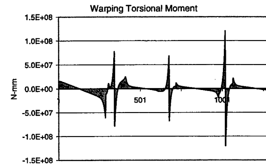
Figure 69: Straining actions for Br. 598 (Dead load)
