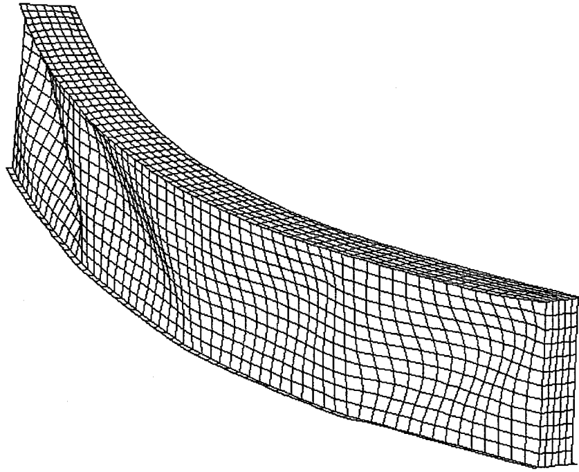
Figure 3: Deformed shape of Verification Girder II (Yabuki et al.)
