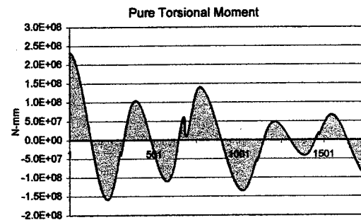
Figure 83: Straining actions for Br.538b (Dead load)
