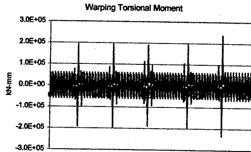
Figure 96: Straining actions for Br.542a (Live load envelope)
