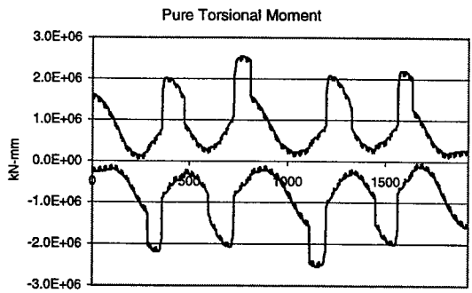
Figure 62: Straining actions for Br. 390 (Live load envelope)
