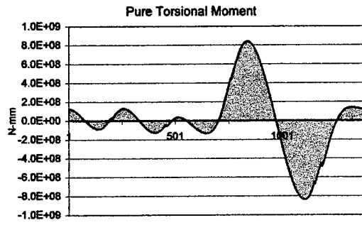
Figure 79: Straining actions for Br.537 (Dead load)
