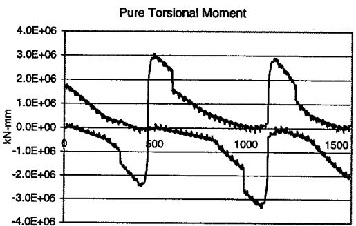
Figure 74: Straining actions for Br. 607 (Live load envelope)
