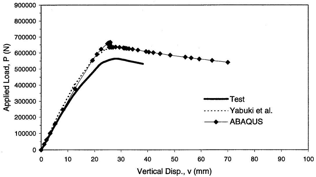
Figure 5: Load-deflection relationship for Girder M-5
