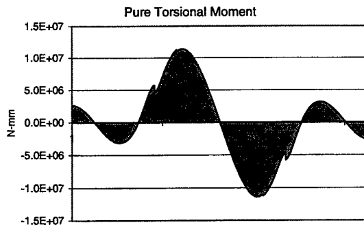
Figure 65: Straining actions for Br. 521 (Dead load)
