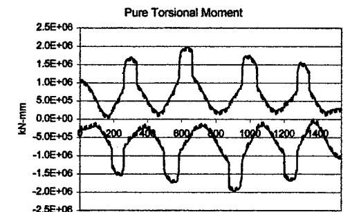
Figure 88: Straining actions for Br.539 (Live load envelope)
