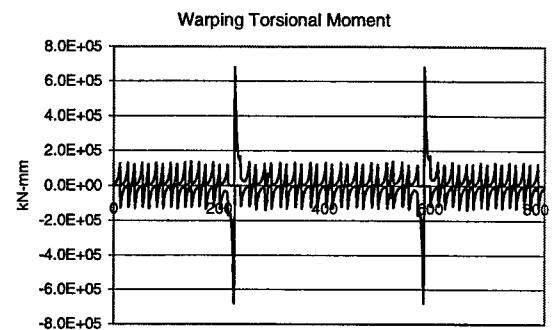
Figure 64: Straining actions for Br. 521 (Live load envelope)
