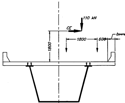
b) Tandem Load (one axle shown)
