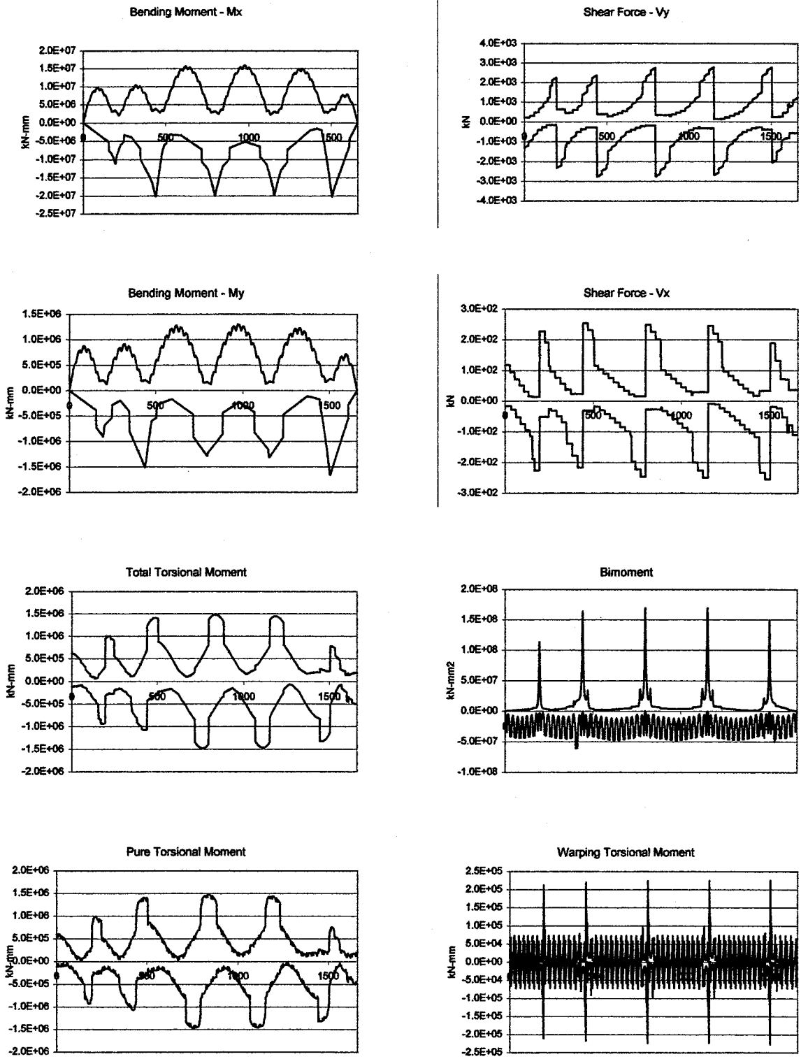
Figure 90: Straining actions for Br.540 (Live load envelope)
