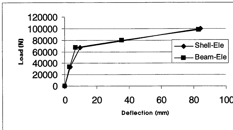
Figure 13: Stiffener study after modification
