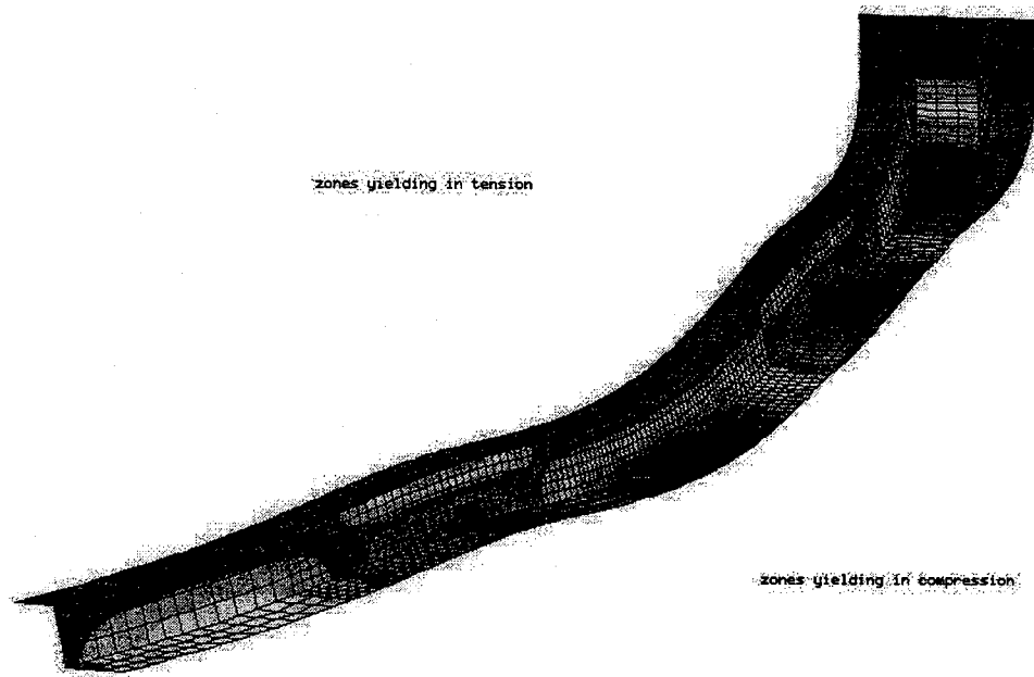
Figure 20: Contours of normal stresses in the longitudinal direction (entire bridge)
