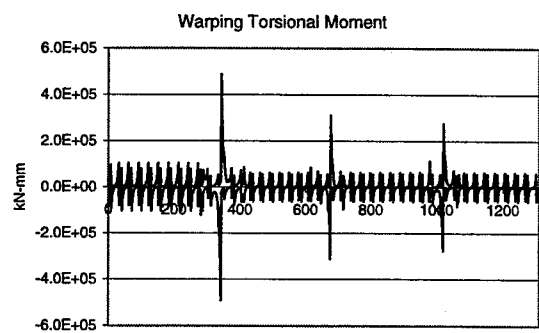
Figure 68: Straining actions for Br. 598 (Live load envelope)
