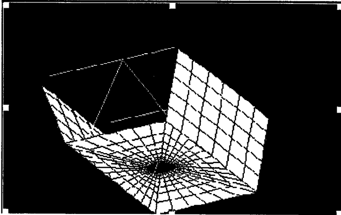
Distribution of stresses in the vicinity of the hole.
