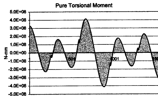
Figure 89: Straining actions for Br.539 (Dead load)
