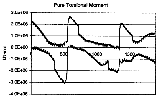
Figure 72: Straining actions for Br. 606 (Live load envelope)
