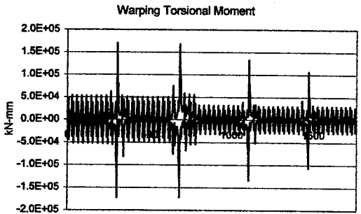
Figure 82: Straining actions for Br.538b (Live load envelope)
