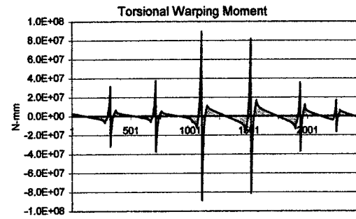
Figure 87: Straining actions for Br.538d (Dead load)
