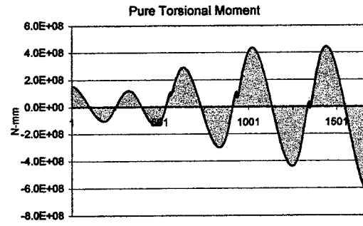
Figure 93: Straining actions for Br.541a (Dead load)
