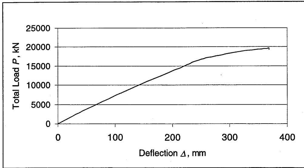
Figure 22: Load-deflection relationship of mid-span point for Bridge 538
