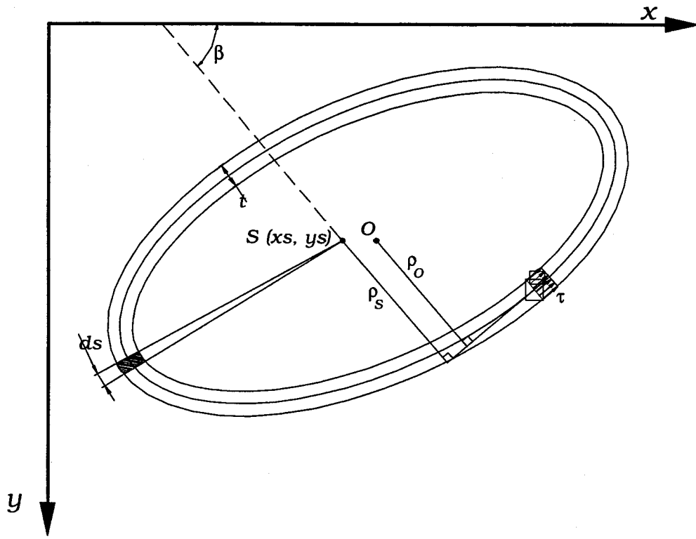
Figure 59: Closed thin-walled cross-section
