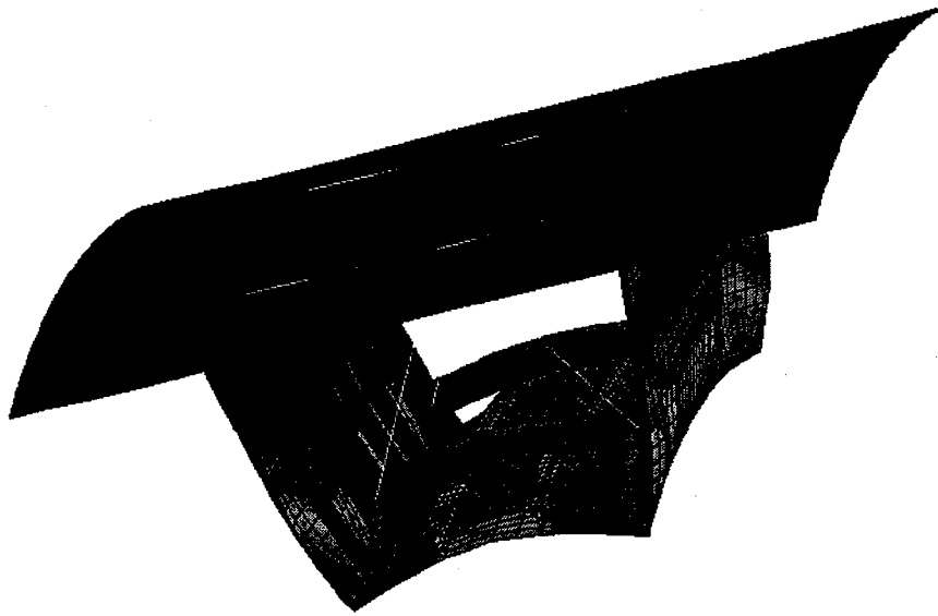
Figure 29: Contours of normal stresses. (negative moment without hole)
