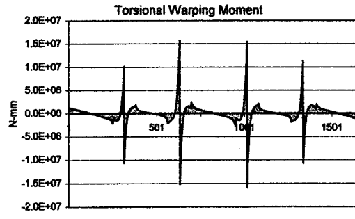
Figure 77: Straining actions for Br.528 (Dead load)
