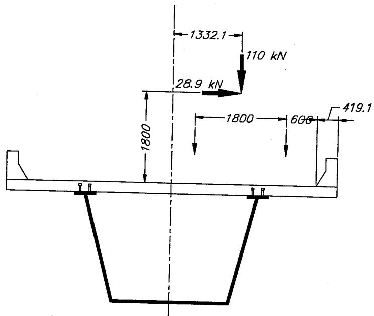
b) Tandem Load (one axle shown)
