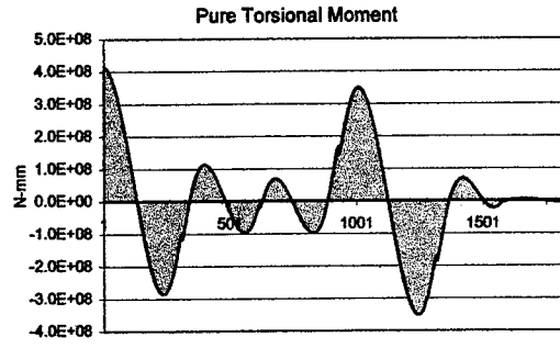
Figure 99: Straining actions for Br.542b (Dead load)
