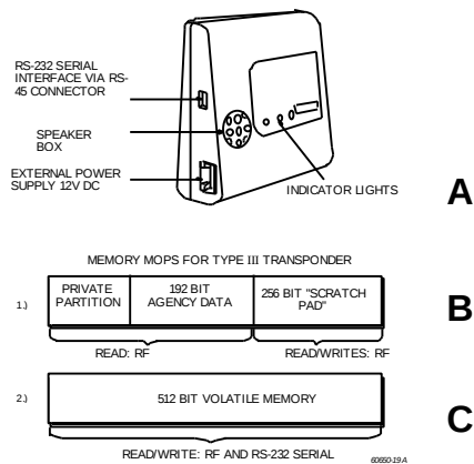
EXHIBIT 3-3 Transponder and Memory Area
