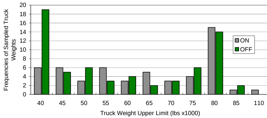
Figure10: Frequencies of Sampled Truck Weights with DTSWS On or Off
