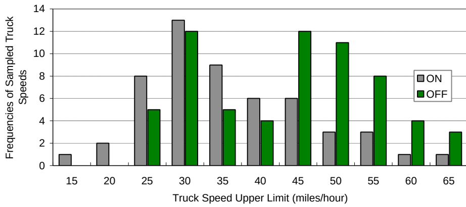
Figure 9: Frequencies of Sampled Truck Speeds with DTWS On or Off
