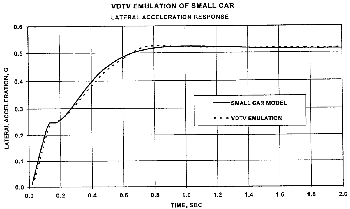
Figure 8 Small Car Emulation Comparison for 0.5g Steady State Lateral Acceleration
