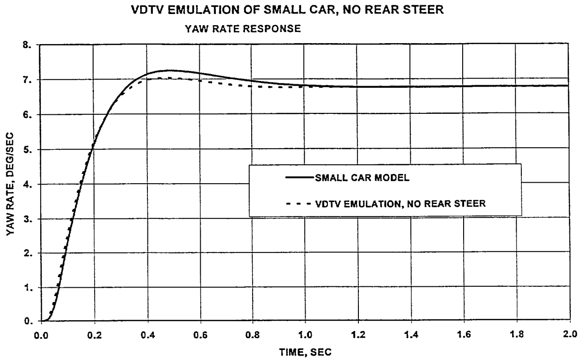
Figure 11a Emulation of Yaw Rate Response without Rear Steer
