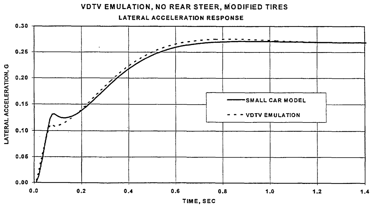
Figure 13a Lateral Acceleration Response, Modified tires
