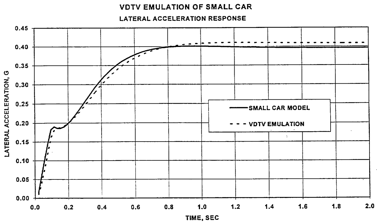
Figure 7 Small Car Emulation Comparison for 0.4g Steady State Lateral Acceleration
