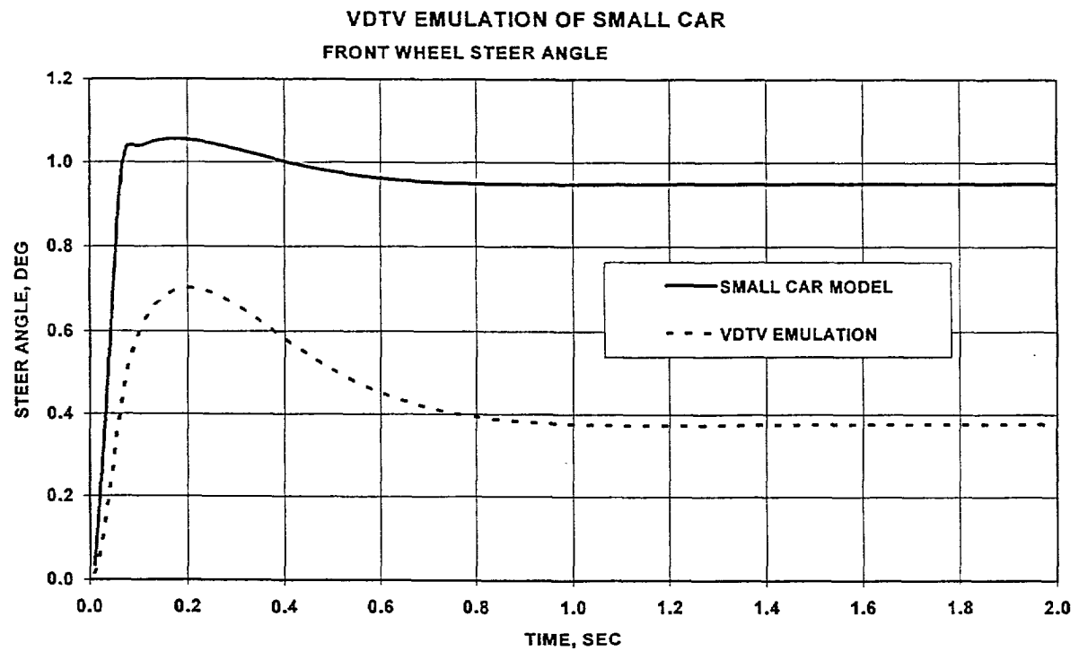
Figure 6e Front Road Wheel Angle
