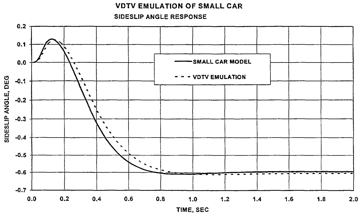
Figure 6d Sideslip Angle
