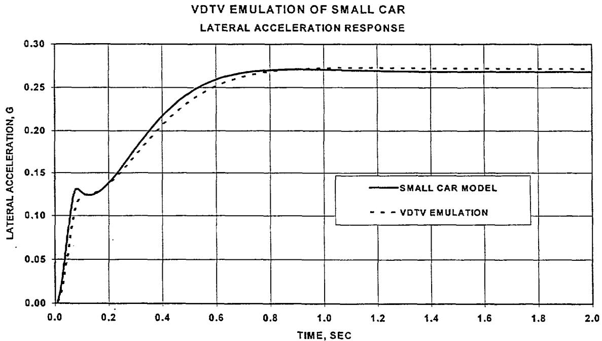
Figure 6 Comparison of Vehicle Responses between Small Car Model and VDTV Emulation 6a Lateral Acceleration
