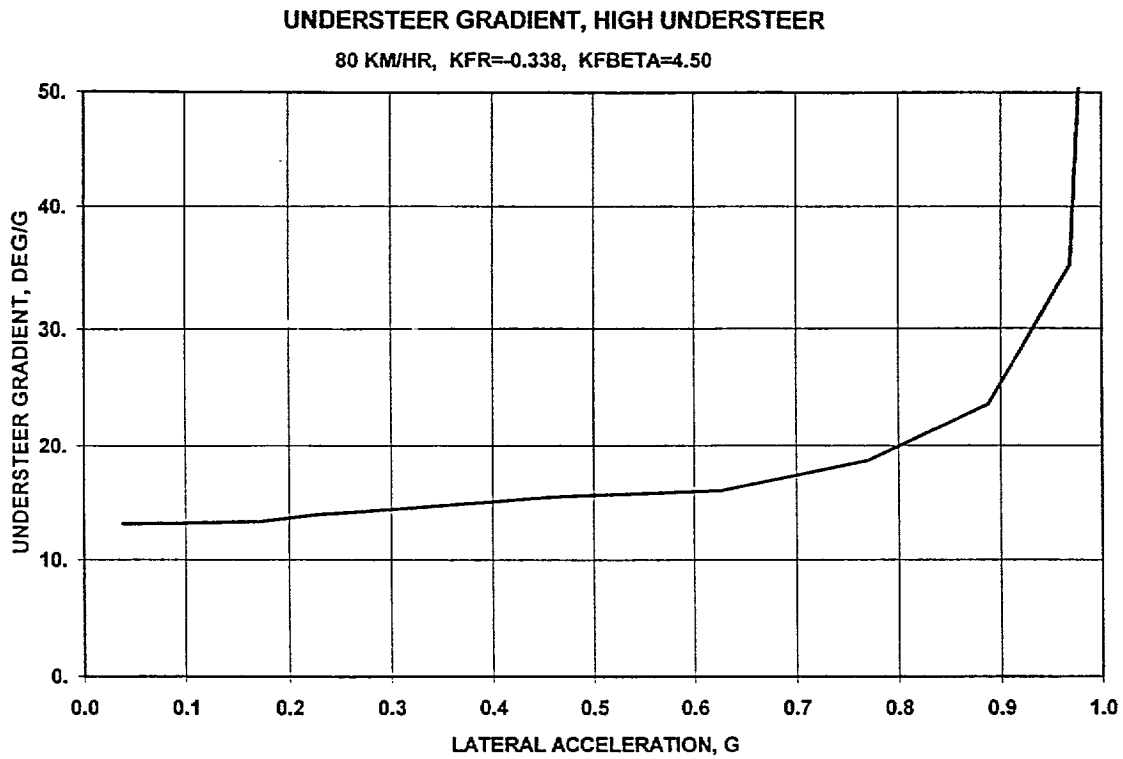
Figure 1 Variation of Understeer Gradient with Lateral Acceleration, High Understeer
