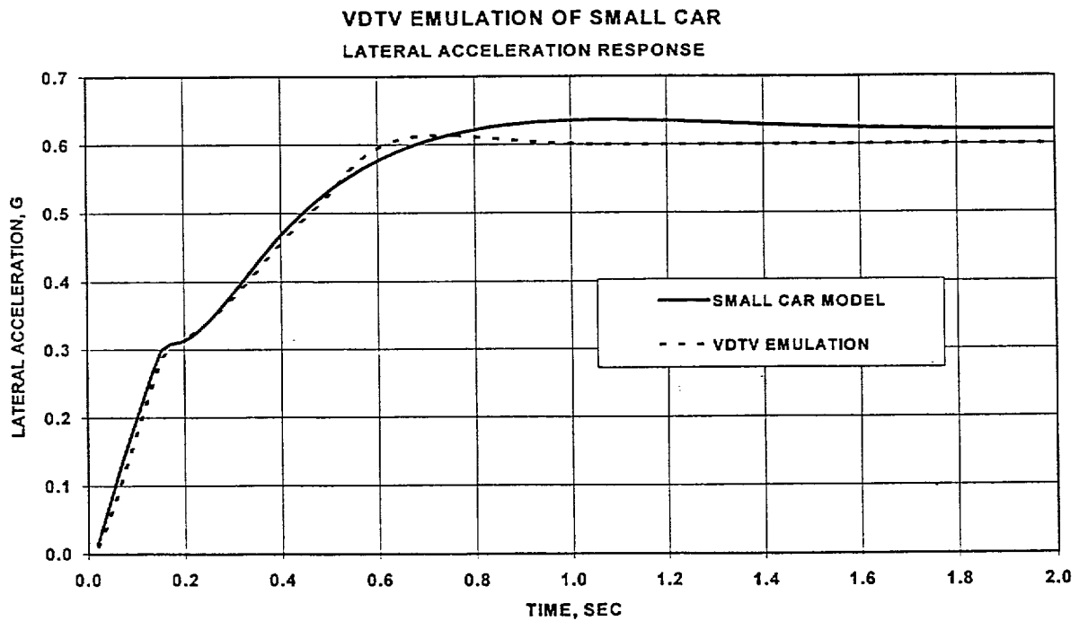
Figure 9 Small Car Emulation Comparison for 0.6g Steady State Lateral Acceleration
