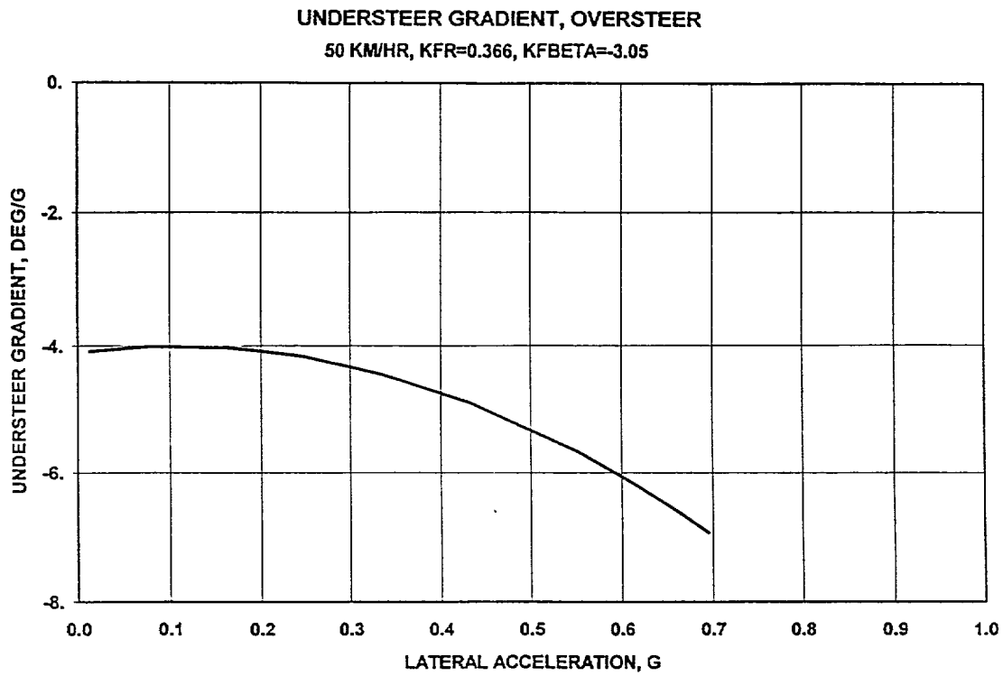
Figure 3 Understeer Gradient Variation with Lateral Acceleration, Oversteer
