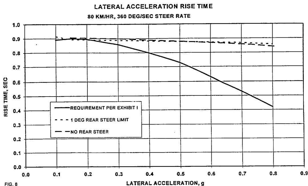
Figure 5 Long Lateral Acceleration Rise Times vs Lateral Acceleration
