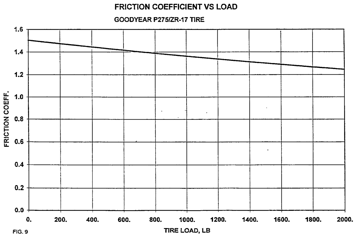
Figure 2 P275/ZR-17 Tire Friction Coefficients vs Load
