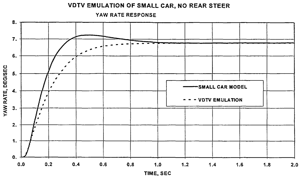
Figure 12b Yaw Rate Response (Lateral Acceleration Response Matched)
