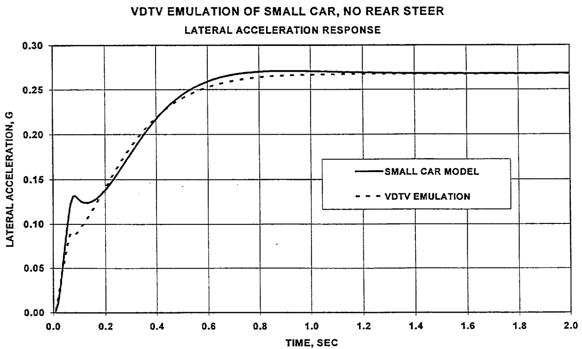
Figure 12a Lateral Acceleration Response (Matched )
