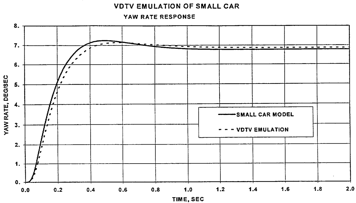
Figure 6b Yaw Rate
