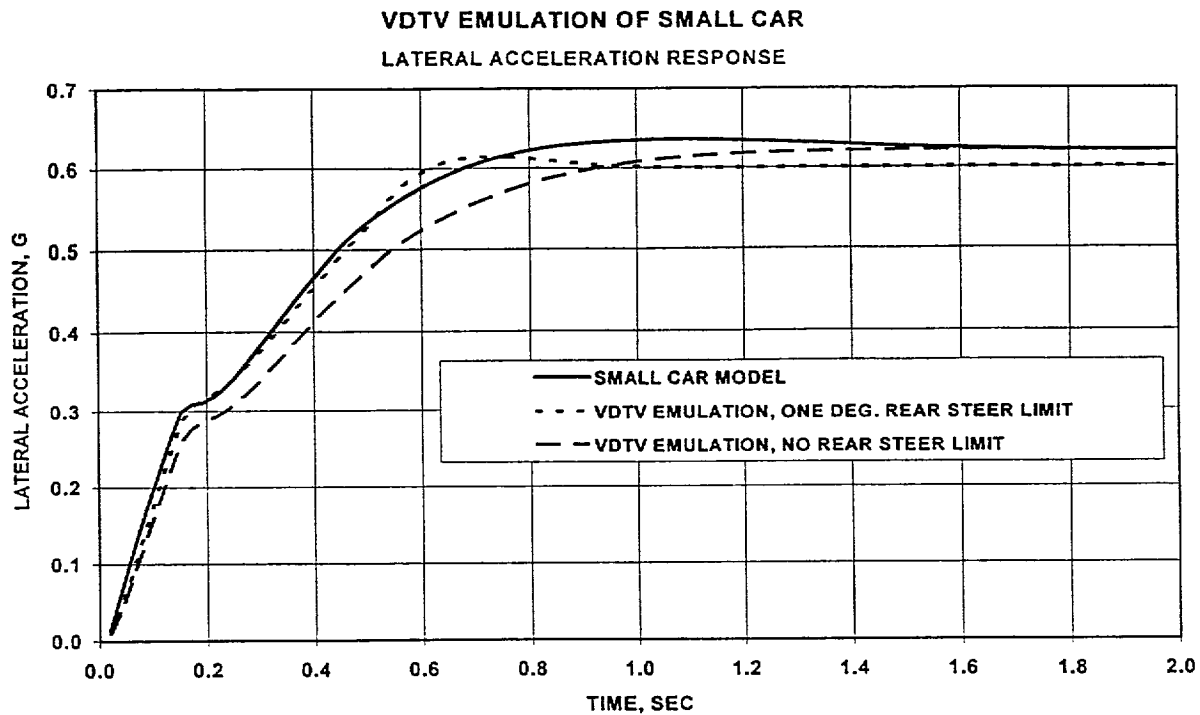
Figure 10 Comparison of Small Car Emulation with Limited and Unlimited Rear Steer
