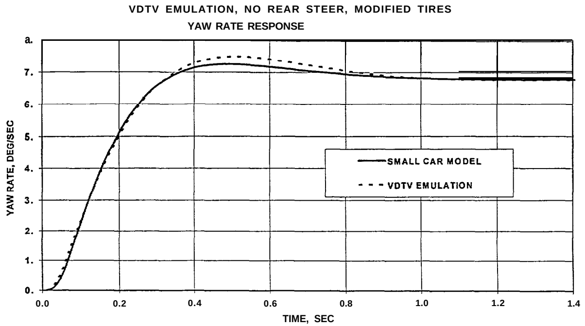
Figure 13b Yaw Rate Response (Modified Tires)
