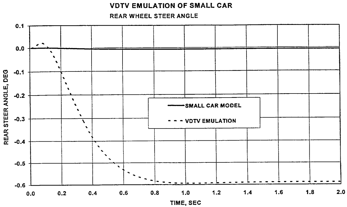
Figure 6f Rear Road Wheel Angle
