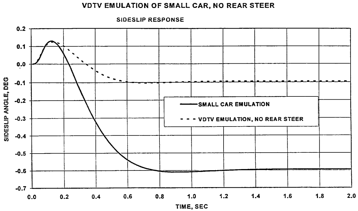
Figure 11c Sideslip Response (Lateral Acceleration Matched for No Rear Steer)
