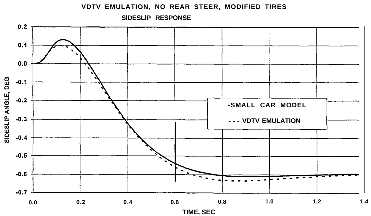
Figure 13c Sideslip Angle Response (Modified Tires)
