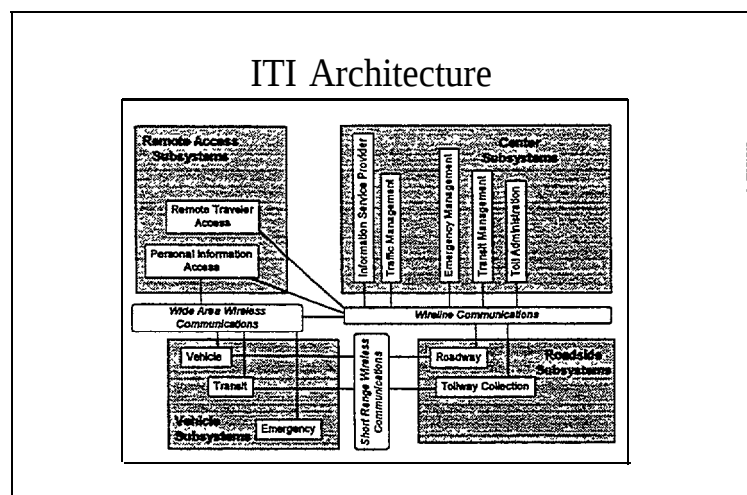
Figure 2. National Architecture Framework for Transportation Infrastructure” (3)
