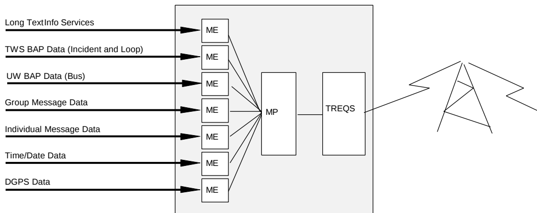
Figure 3-6. Message Data System (MDS) Information Flow at the SCS Network Node.
