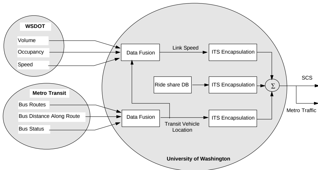
Figure 3-8. UW SWIFT Functions.
