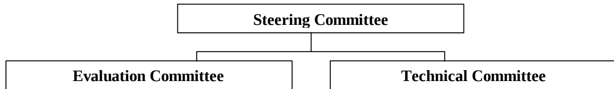
Figure 3-3. SWIFT Committees.
