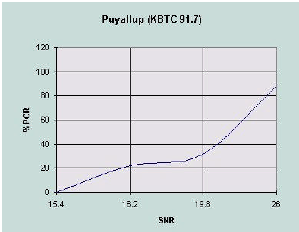
Figure 3-23. PCR versus SNR Performance for KBTC at Site #8.
