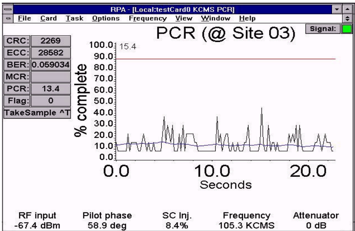
Figure 3-25. Suspected KCMS Multi-path Signal Measured at Site #3 with Omni Antenna.
