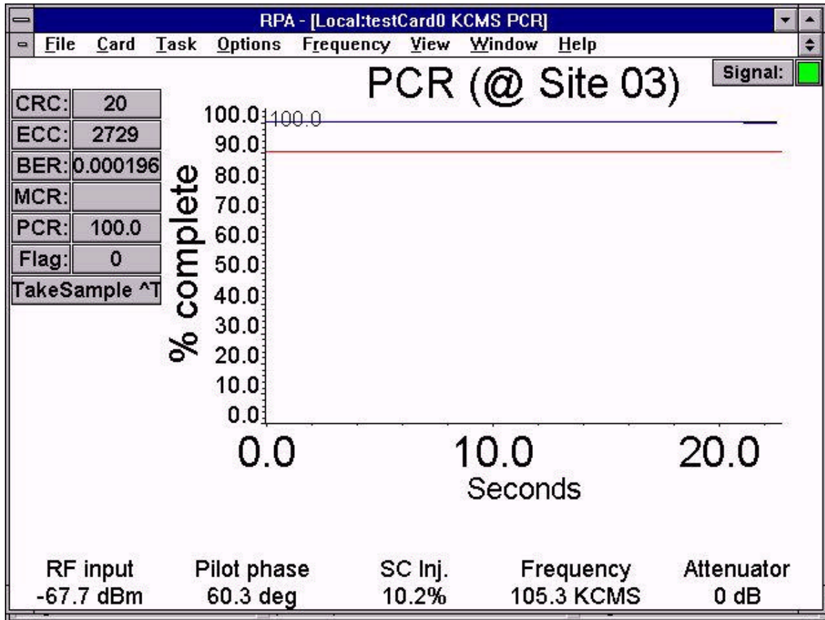
Figure 3-26. Same KCMS Multi-path Signal Measured at Site #3 with Directional FM Antenna.
