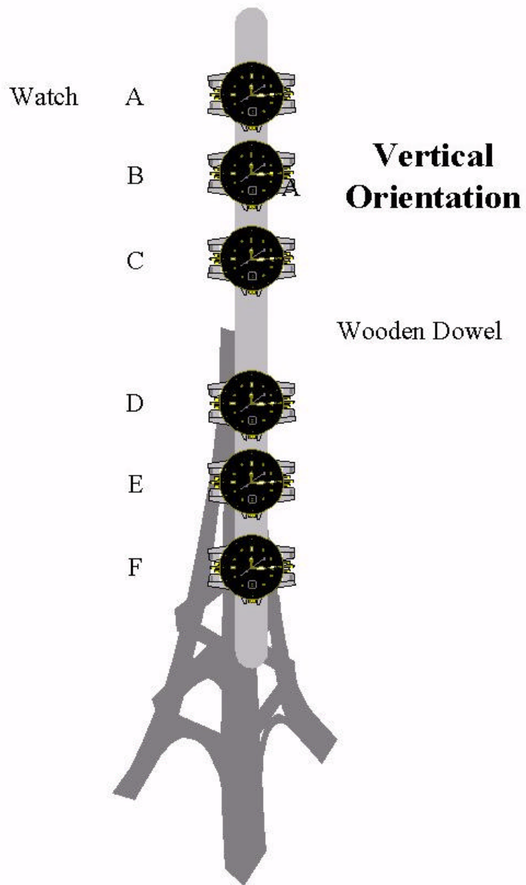
Figure 2-3. Drawing of Seiko MessageWatch Vertical Test Configuration.
