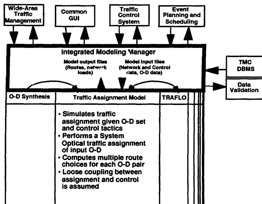
Figure 2-32. The Integrated Modeling Manager Subsystem
