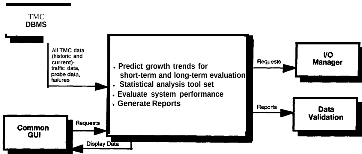
Figure 2-31. The Historical Data Analysis Subsystem
