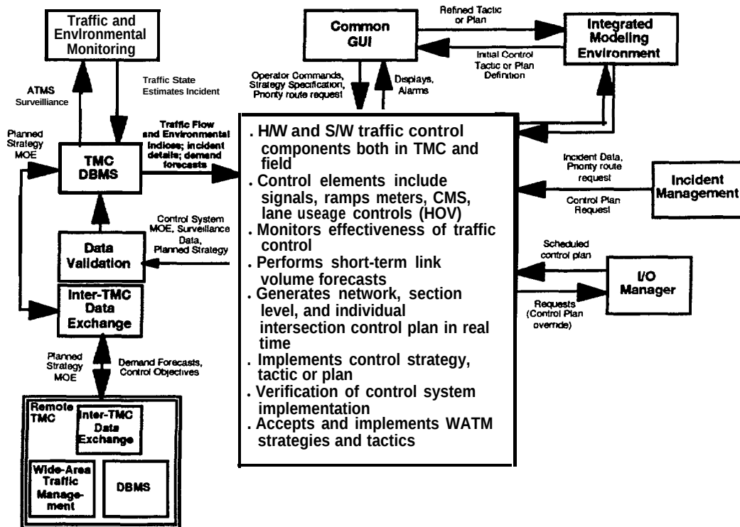
Figure 2-17. The Traffic Control Subsystem
