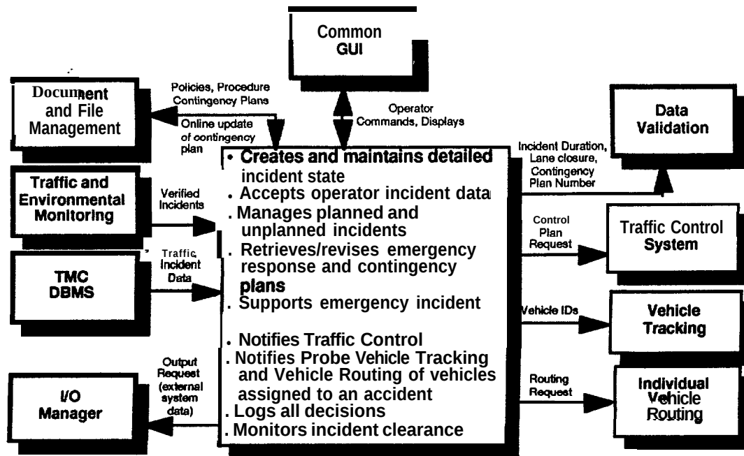
Figure 2-16. The Incident Management Subsystem
