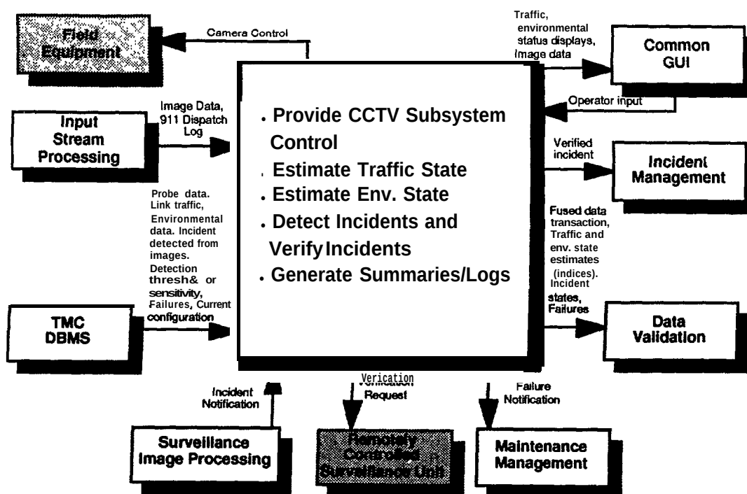
Figure 2-8. The Traffic and Environmental Monitoring Subsystem
