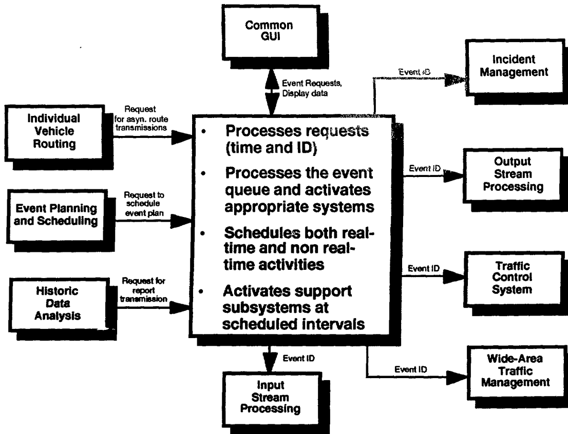
Figure 2-3. The I/O Manager Subsystem
