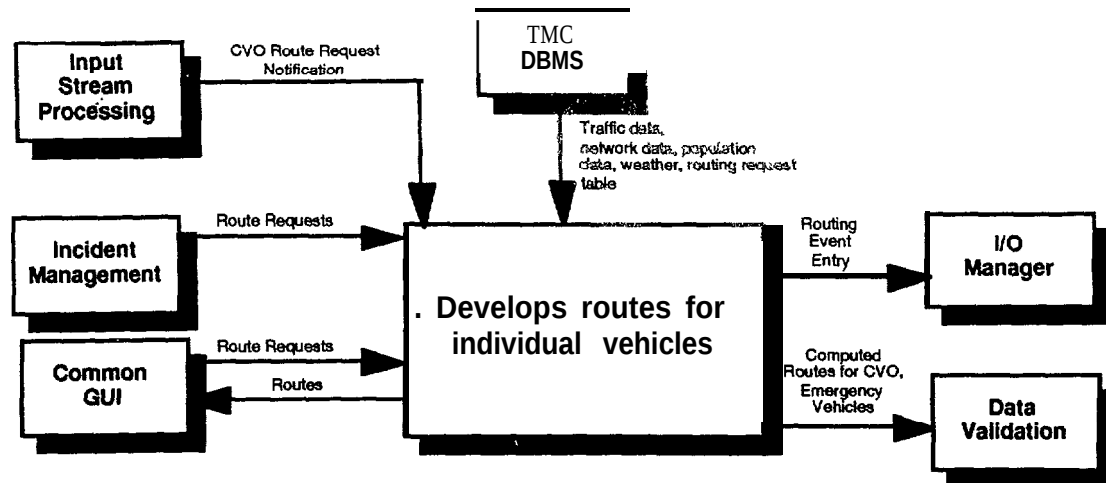
Figure 2-20 The Individual Vehicle Routing Subsystem
