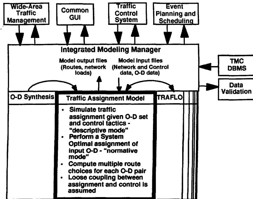
Figure 2-29. The Dynamic Traffic Assignment Subsystem
