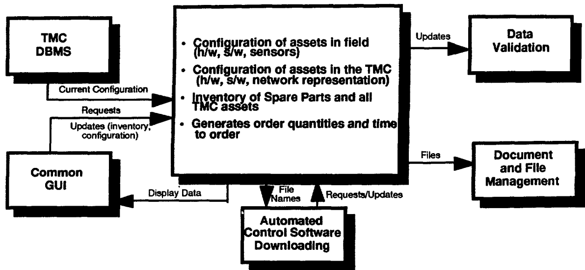
Figure 2-23. The Configuration and Inventory Management Subsystem
