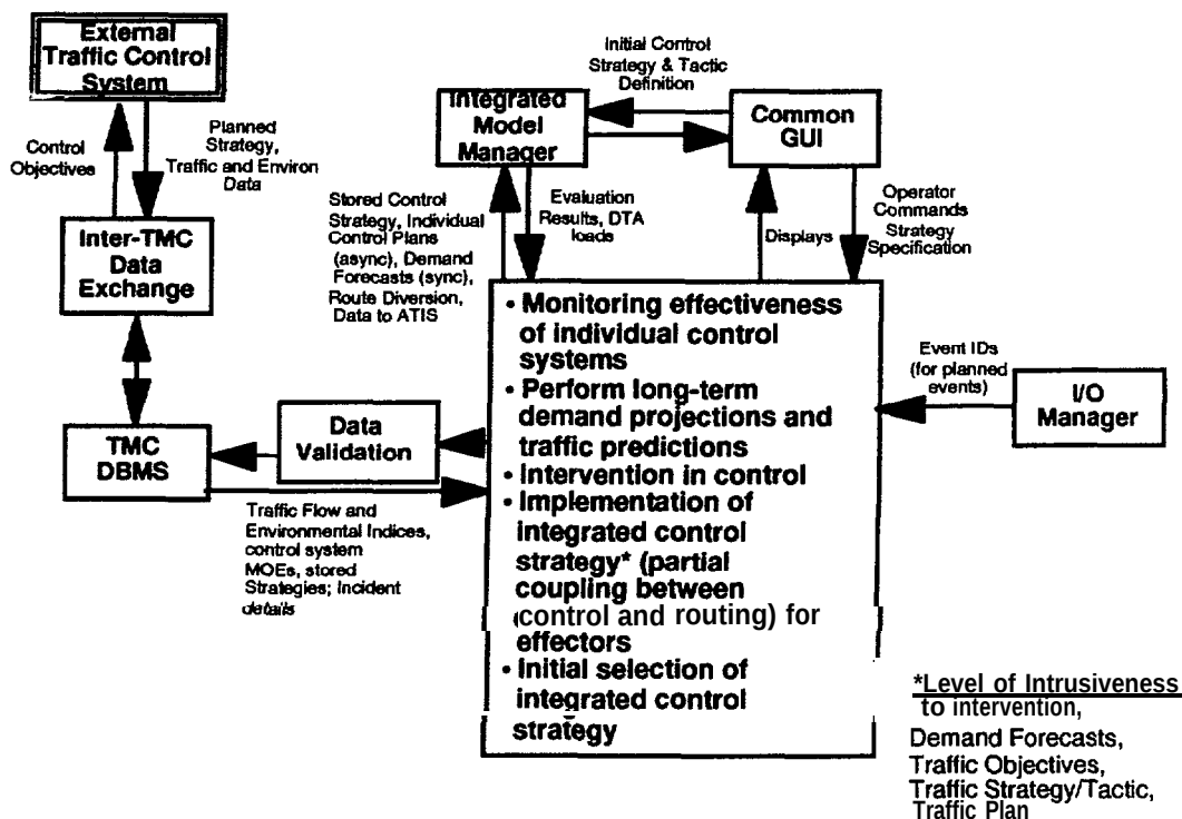
Figure 2-19. The Wide-Area Traffic Management Subsystem
