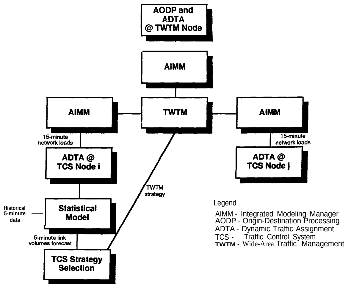
Figure 230. Dynamic Traffic Assignment Subsystem Interfaces
