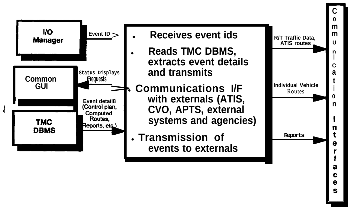
Figure 2-5. The Output Stream Processing Subsystem
