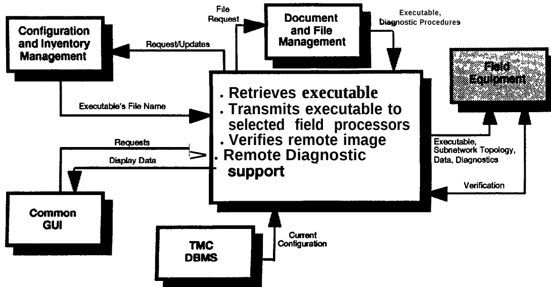
Figure 2-22. The Automated Control Software Downloading Subsystem
