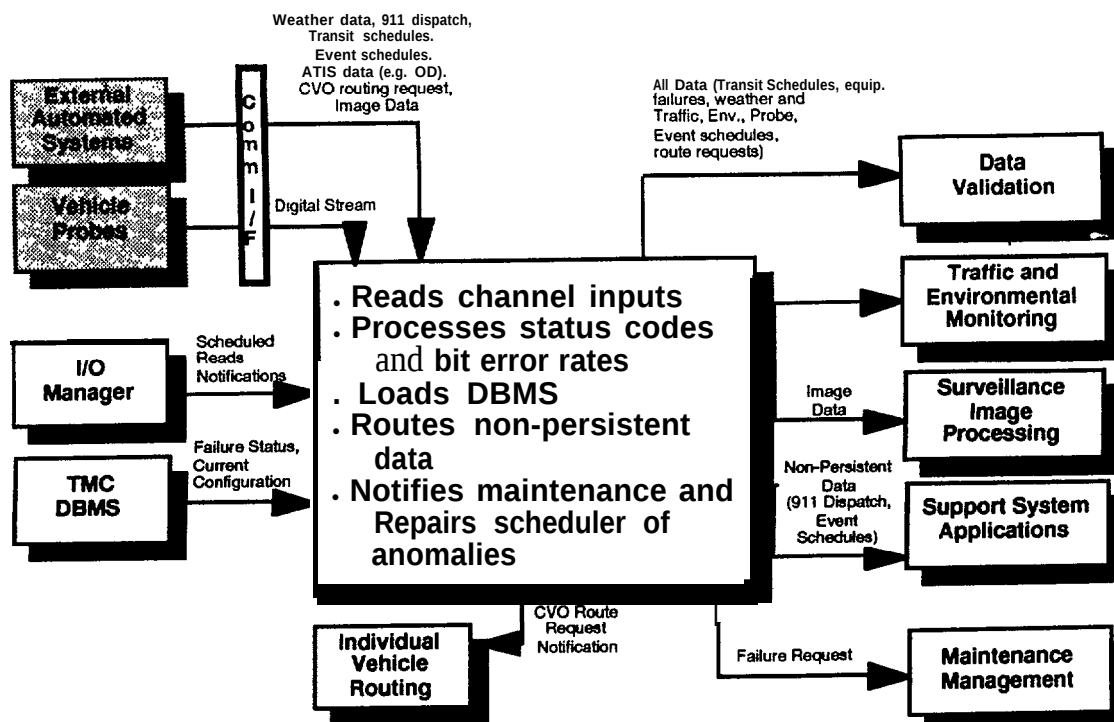
Figure 2-4. The Input Stream Processing Subsystem
