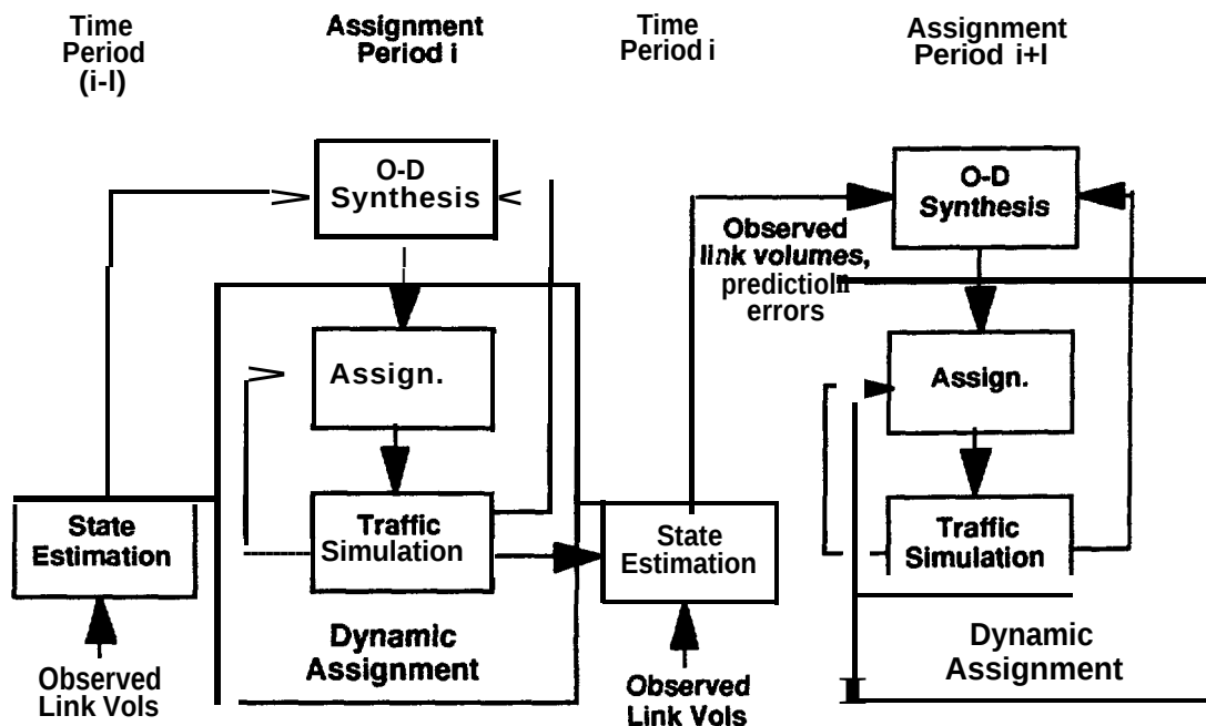
Figure 2-33. The Origin-Destination Processing Subsystem
