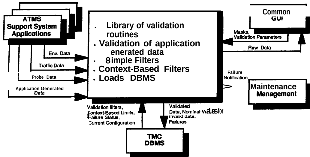
Figure 2-11. The Data Validation Subsystem
