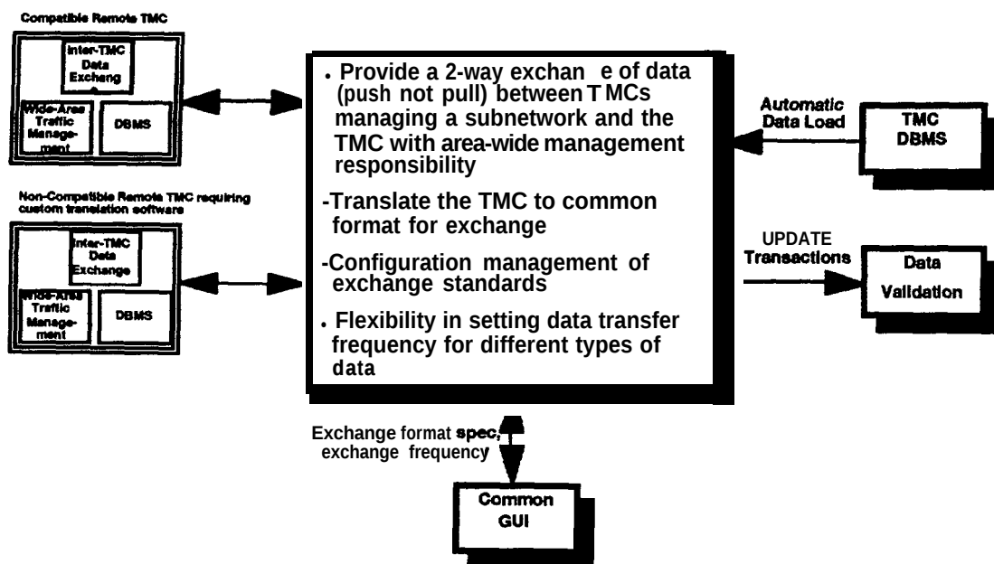
Figure 2-13. The Inter-TMC Data Exchange Subsystem
