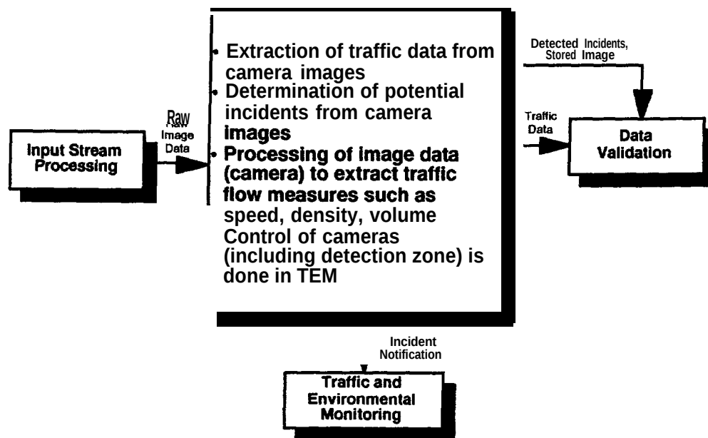
Figure 2-7. The Surveillance Image Processing Subsystem
