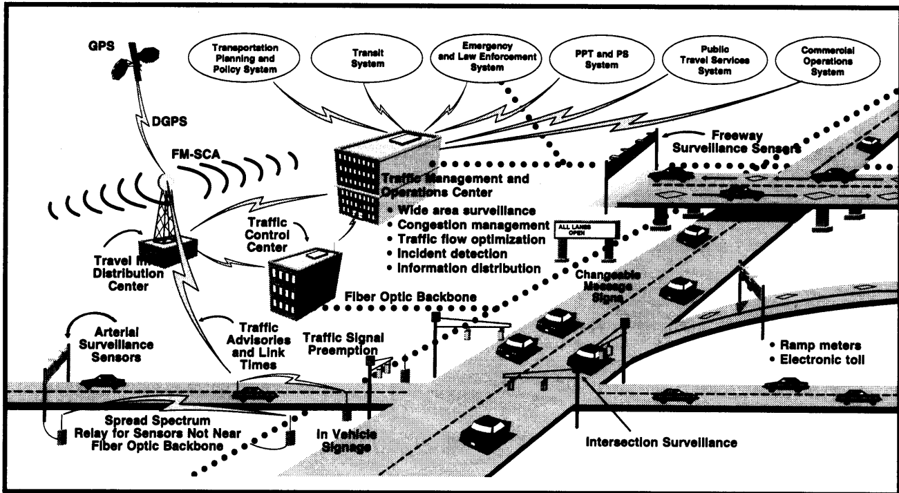
Figure 13. The functions of the Transportation Monitoring and Management System (System #2) are focused on real time adaptive traffic control.
