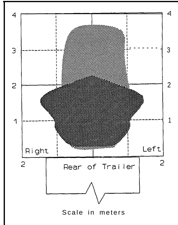
Figure 1 Shortest and Longest Detection Zones to Cardboard Target Covered by Rear Object Detection Systems
