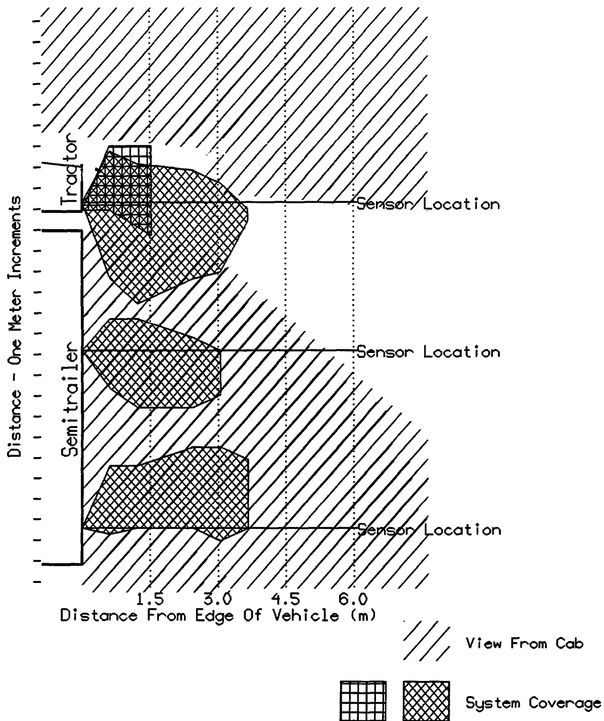
Figure 3 Detection Zones of Two, Right-Side Object Detection Systems and Driver View From the Tractor Cab
