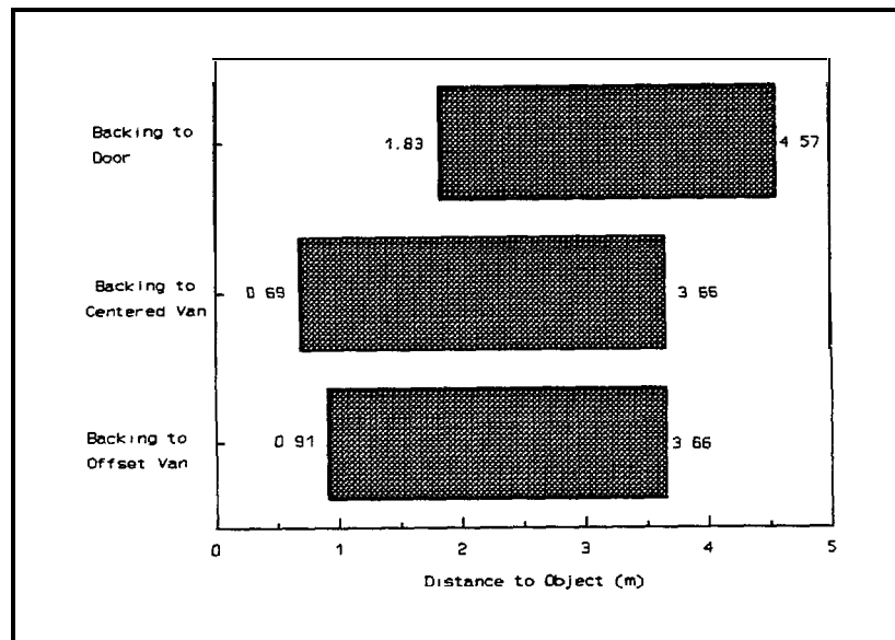
Figure 2 The Range of Maximum Detection Distances to Three Different Objects Provided by Five Rear Object Detection Systems
