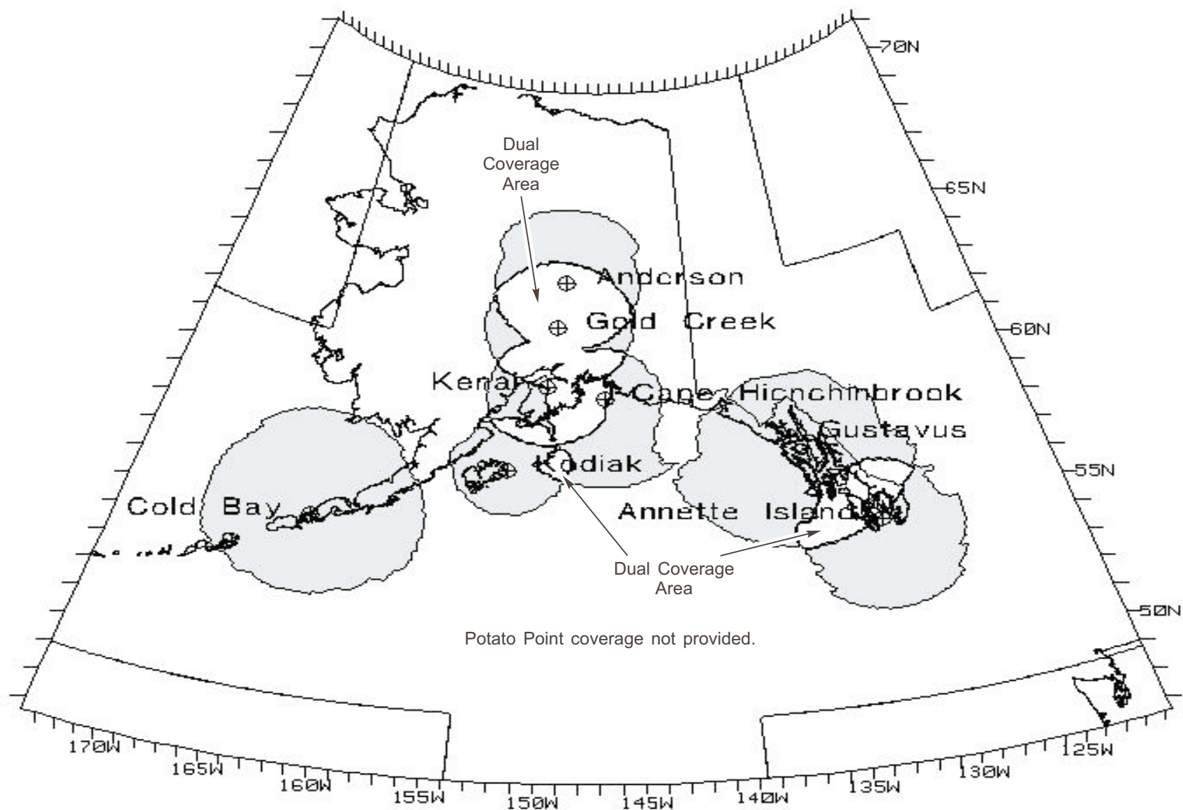
FIGURE 11 ESTIMATED PHASE I NDGPS COVERAGE (ALASKA)
