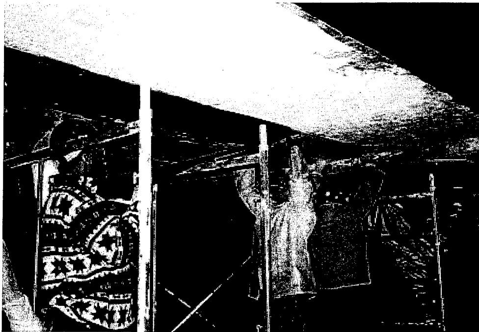
Figure 2.9. Application of CFRP Sheet
