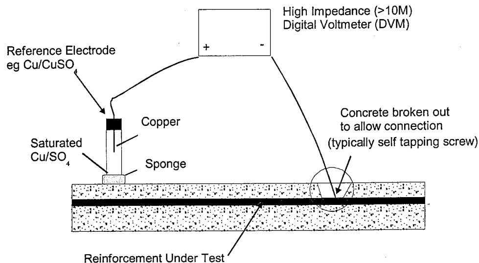
Figure 2.1. Schematic of Half-Cell Potential Measurement Technique
