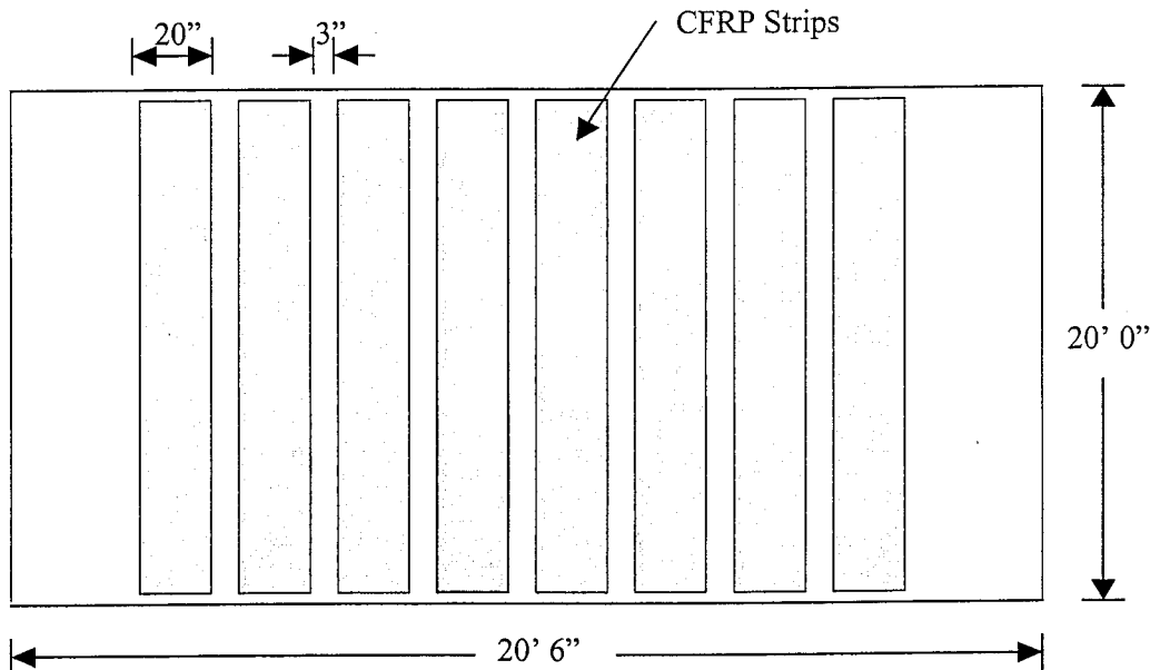
Figure 4.3. CFRP Strengthening Pattern
