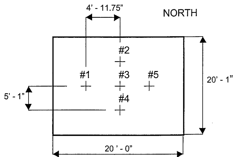
Figure 6.4. LVDT Layout
