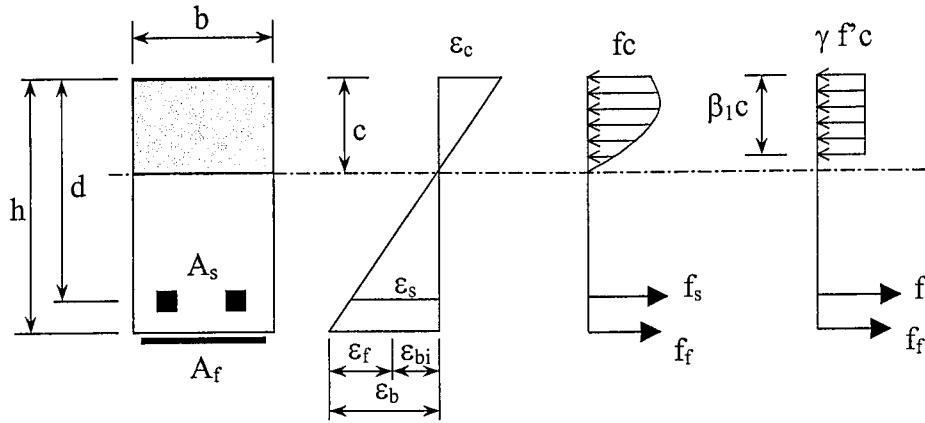
Figure 4.2. Strain and Stress Distribution in a RC Section at Ultimate
