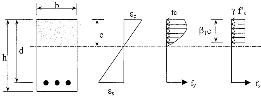
Figure 3.2. Strain and Stress Diagrams for Load Factor
