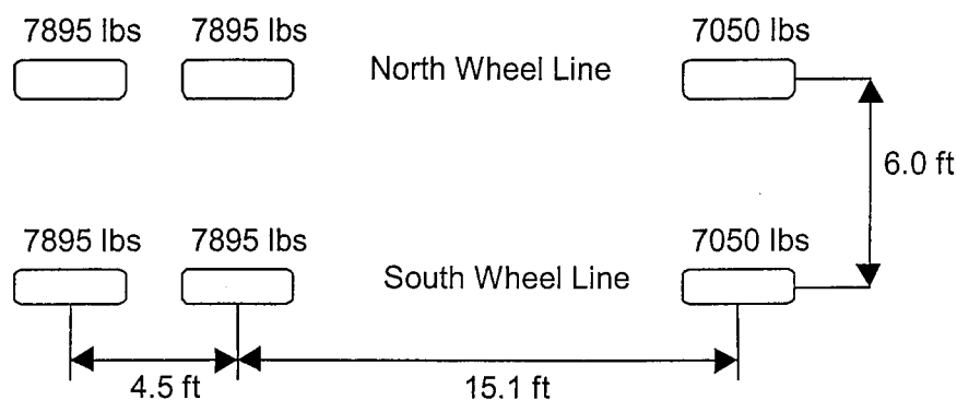
Figure 6.6. UMR Test Truck Wheel Loads
