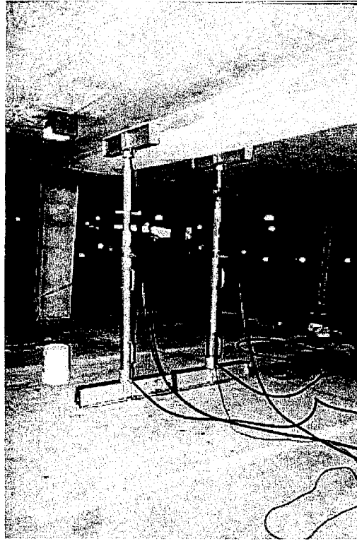
Figure 2.10. Site Load Test of the Repaired Structure
