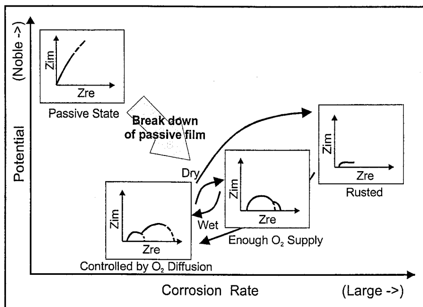
Figure 2.2. Schematic Illustration of Corrosion Data Obtained Using Potential and Impedance Curves
