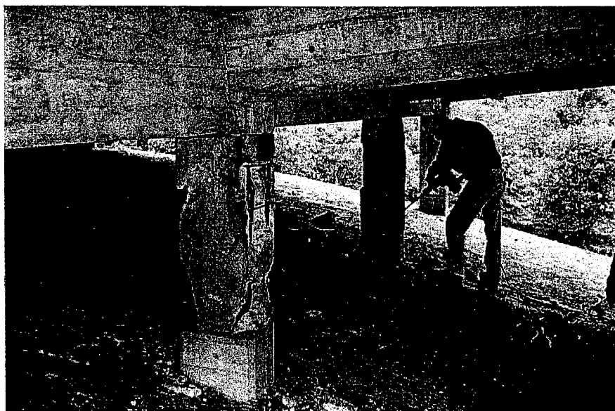
Figure 2.7. Deteriorated Columns
