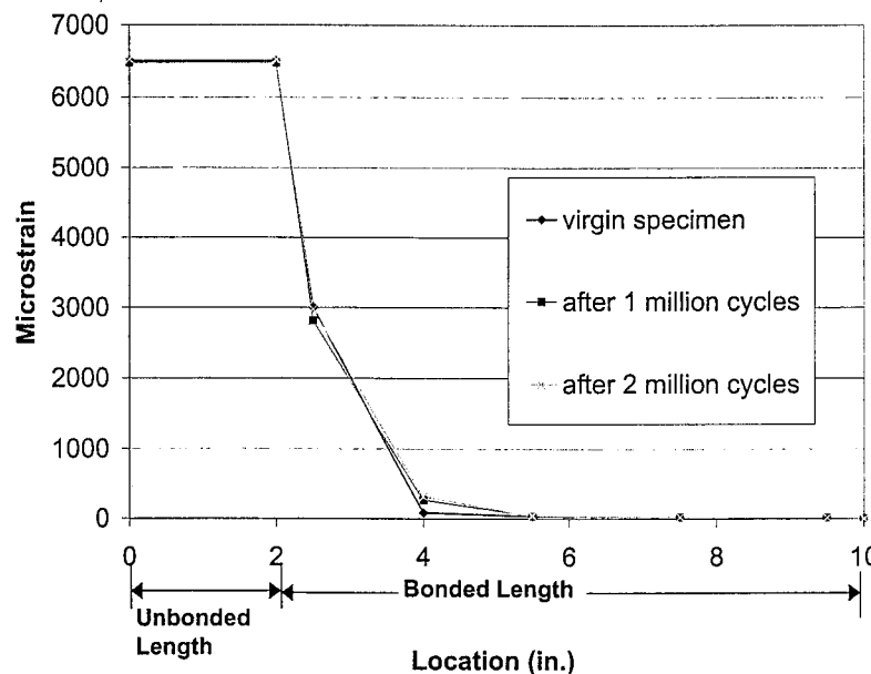
Figure 5.9. Strain Distribution at Different Levels of Fatigue Conditioning (Specimen No. 3)
