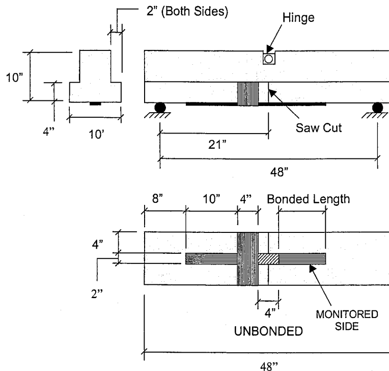
Figure 5.5. Fatigue Test Specimen
