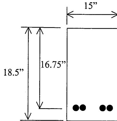
Figure 5.1. Cross-section of the Tested Beams
