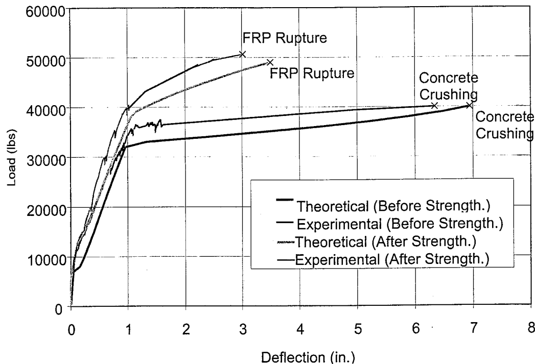
Figure 5.3. Load-Deflection Curves
