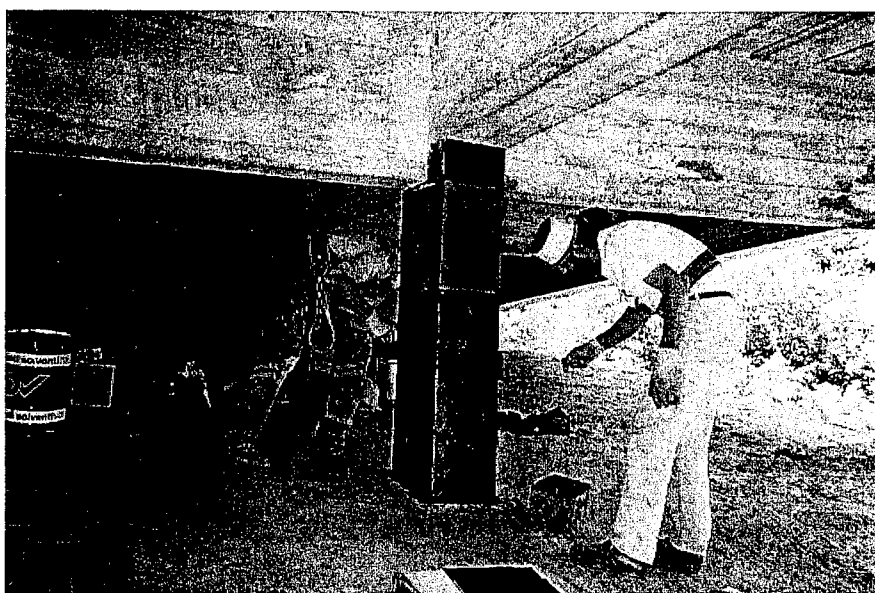
Figure 2.8. Application of the CFRP to Column
