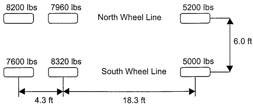
Figure 6.3. UMC Test Truck Wheel Loads
