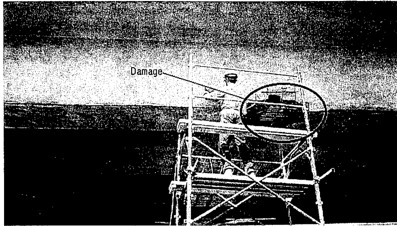
Figure 2.4. Girder Damage Due to Vehicular Impact
