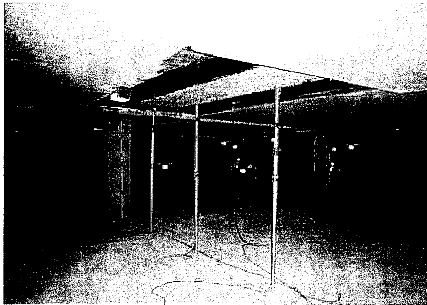
Figure 2.11. Measurement of Deflection During Loading
