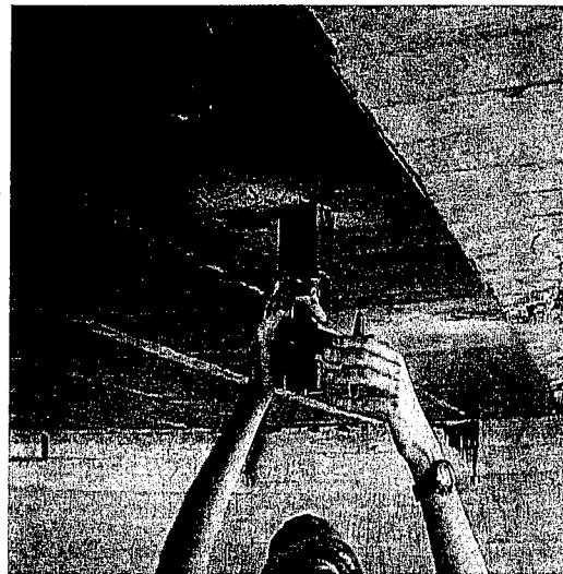
Figure 7.9 Pull-off Test Apparatus
