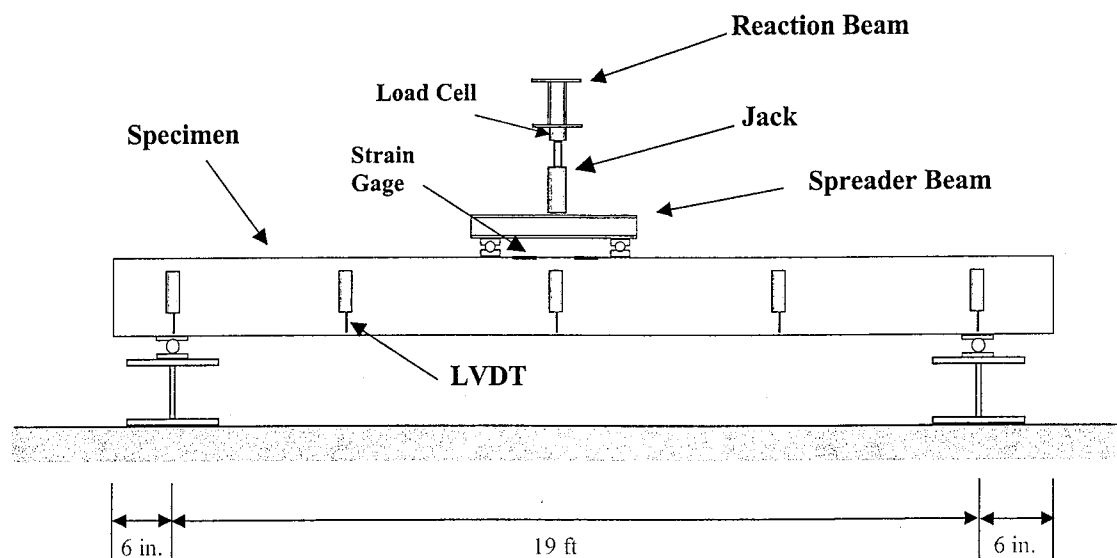
Note: 1 ft = 0.3048 m Figure 5.2. Flexural Test Setup
