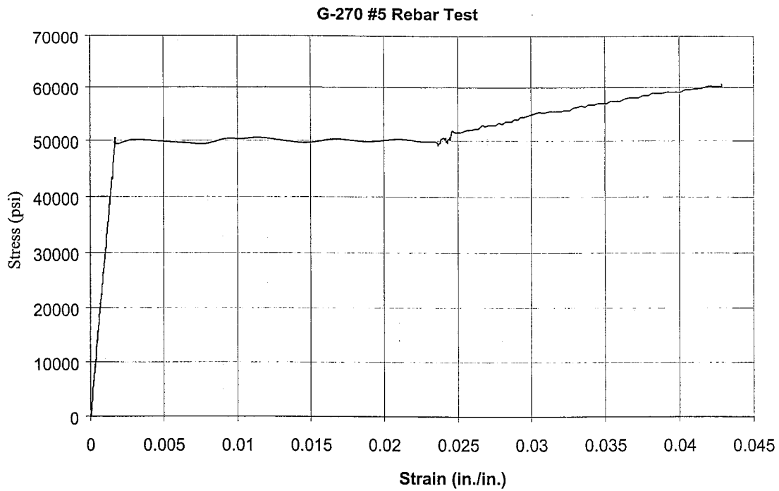
Figure C.1. Stress-strain Curve of Steel Rebar #5 Note: 1000 psi = 6.89 MPa
