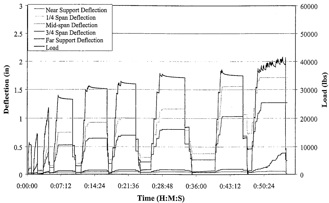
Figure C.3. Deflection-Time History for Beam Test #1 (Unstrengthened) Note: 1 in = 25.4 mm; 1 lb = 4.45 N
