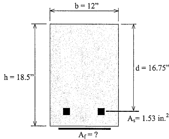
Figure 4.1. Dimensions of the Cross-section
