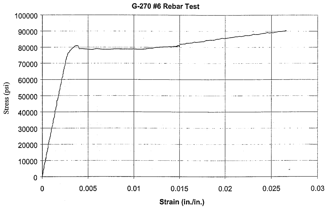
Figure C.2. Stress-strain Curve of Steel Rebar #6 Note: 1000 psi = 6.89 MPa
