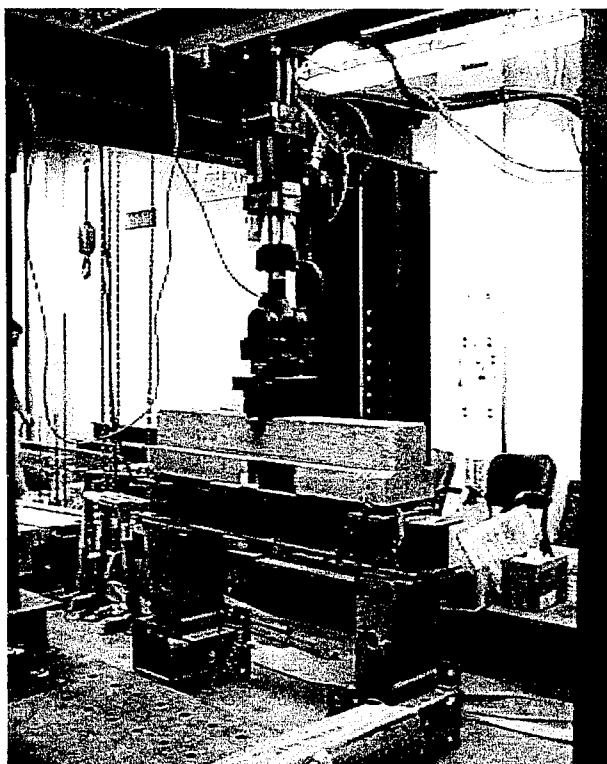
Figure 5.6. Fatigue Test Setup
