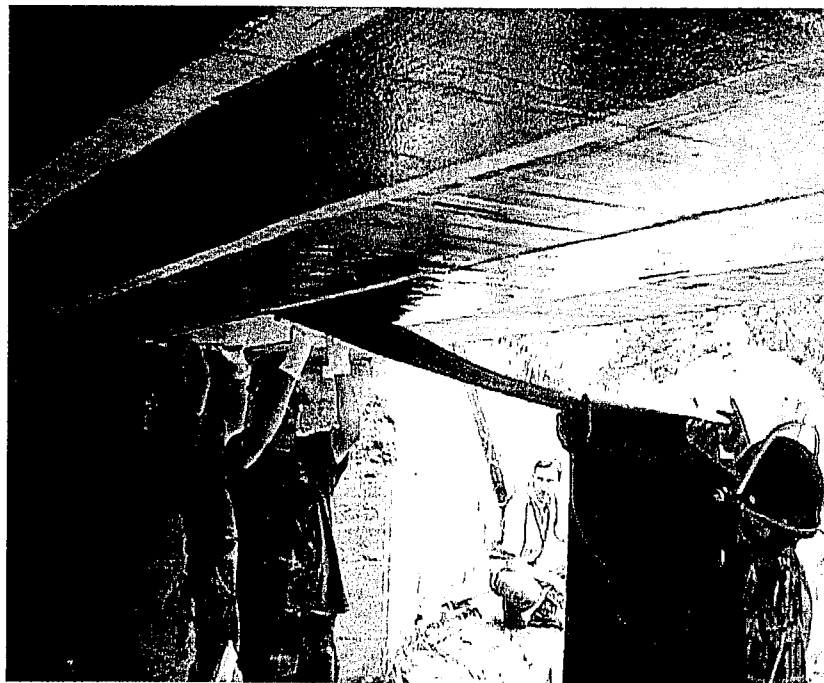
Figure 6.2. Installation of the CFRP Sheets
