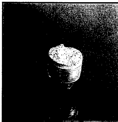
Figure 7.10. Adhesion Fixture Showing Concrete Failure Mode.
