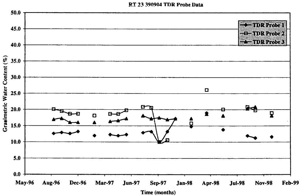
Figure 3.6: TDR Data 390904
