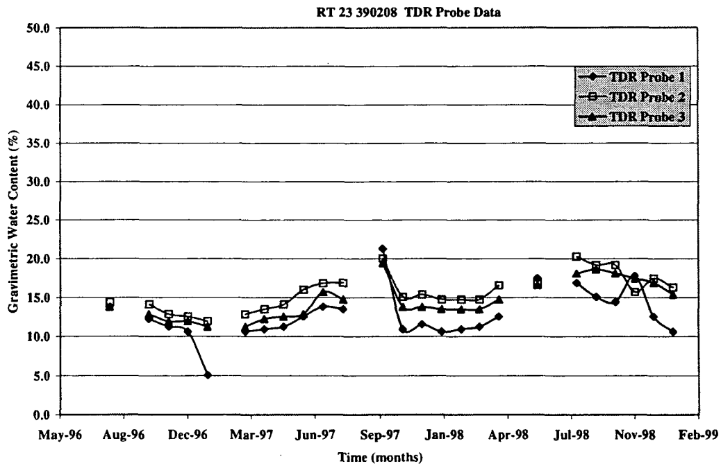
Figure 3.12: TDR Data 390208
