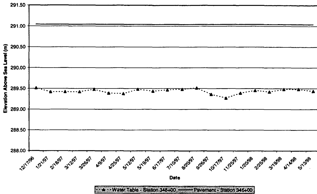
Figure 2.5: Piezometer Readings Station 346+00
