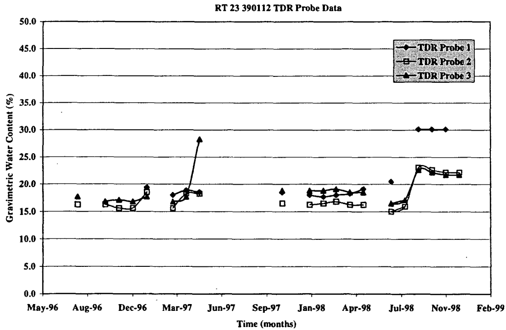
Figure 3.4: TDR Data 390112
