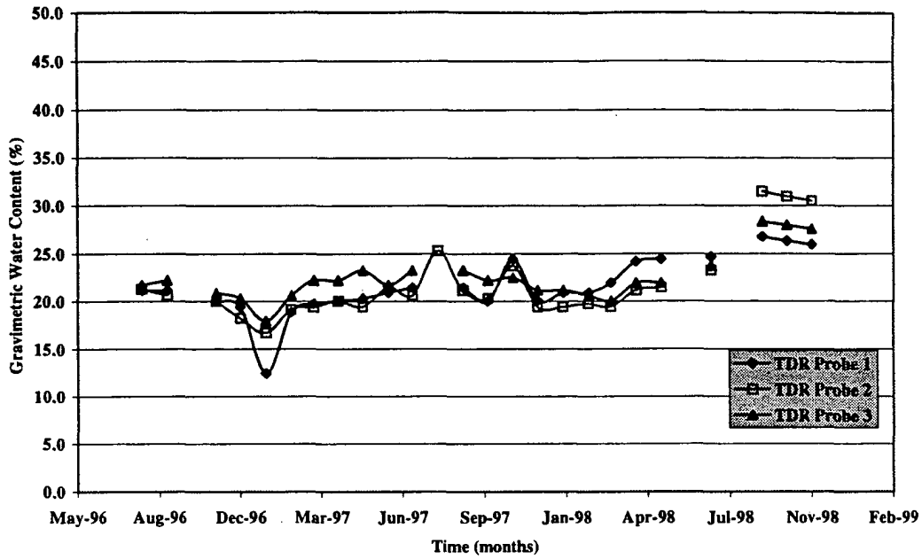
Figure 3.1: TDR Data 390104
