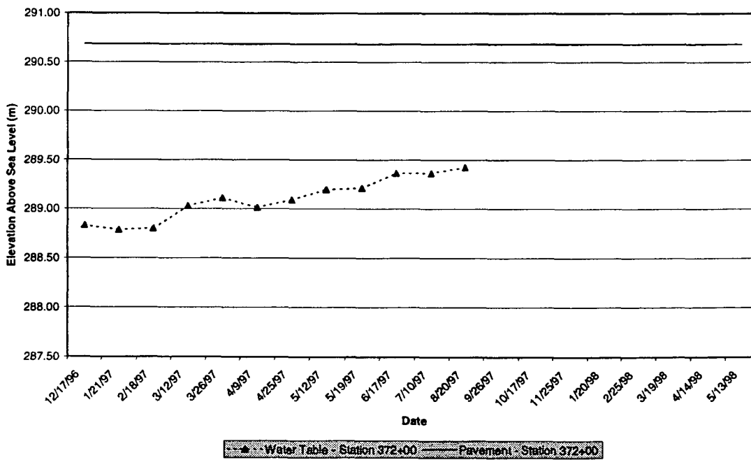
Figure 2.6: Piezometer Readings Station 372+00
