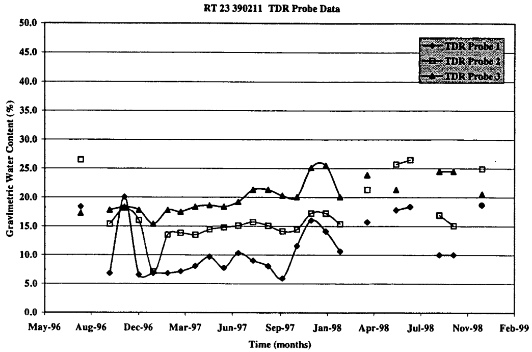
Figure 3.13: TDR Data 390211
