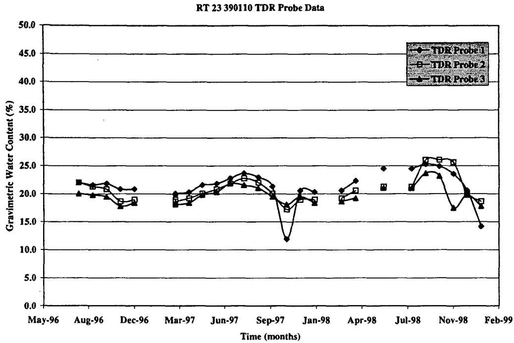
Figure 3.3: TDR Data 390110
