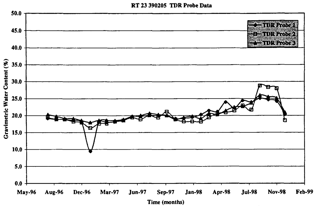
Figure 3.11: TDR Data 390205
