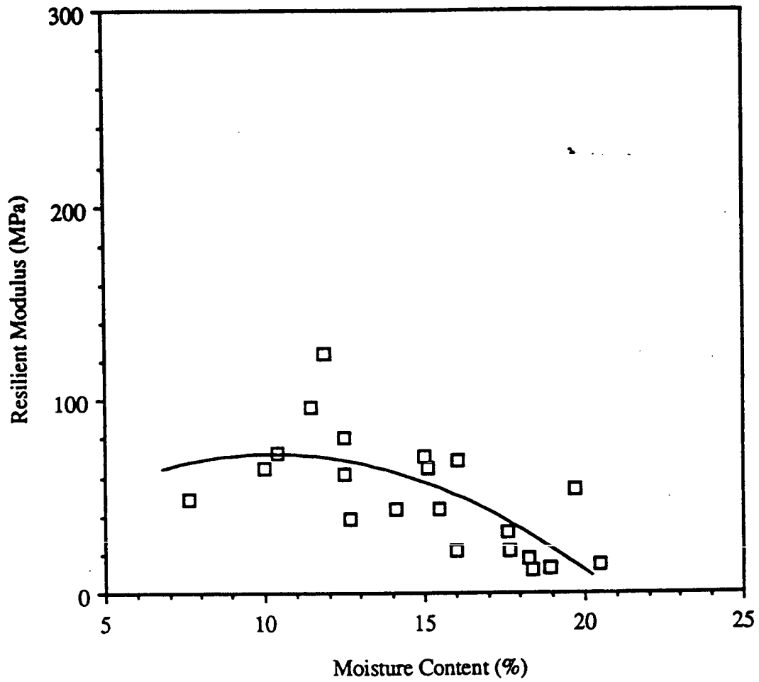
Figure 5.5.(d): Resilient Modulus Vs. Moisture Content Plot for A-6 Soil Specimens (Deviator Stress = 41.4 kPa)
