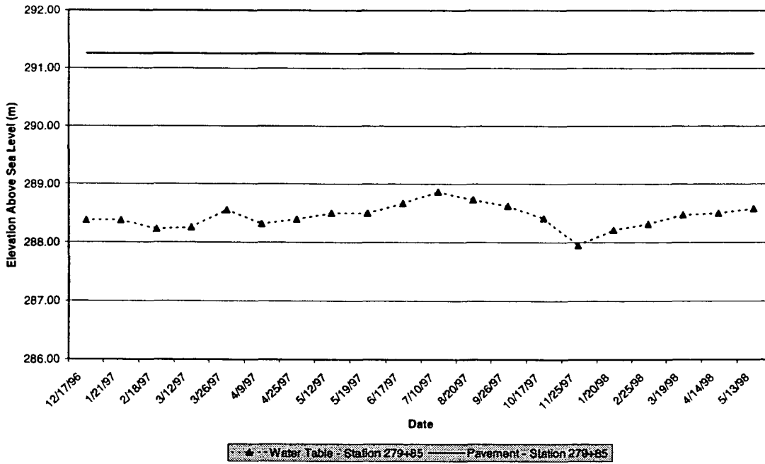
Figure 2.2: Piezometer Readings Station 279+85
