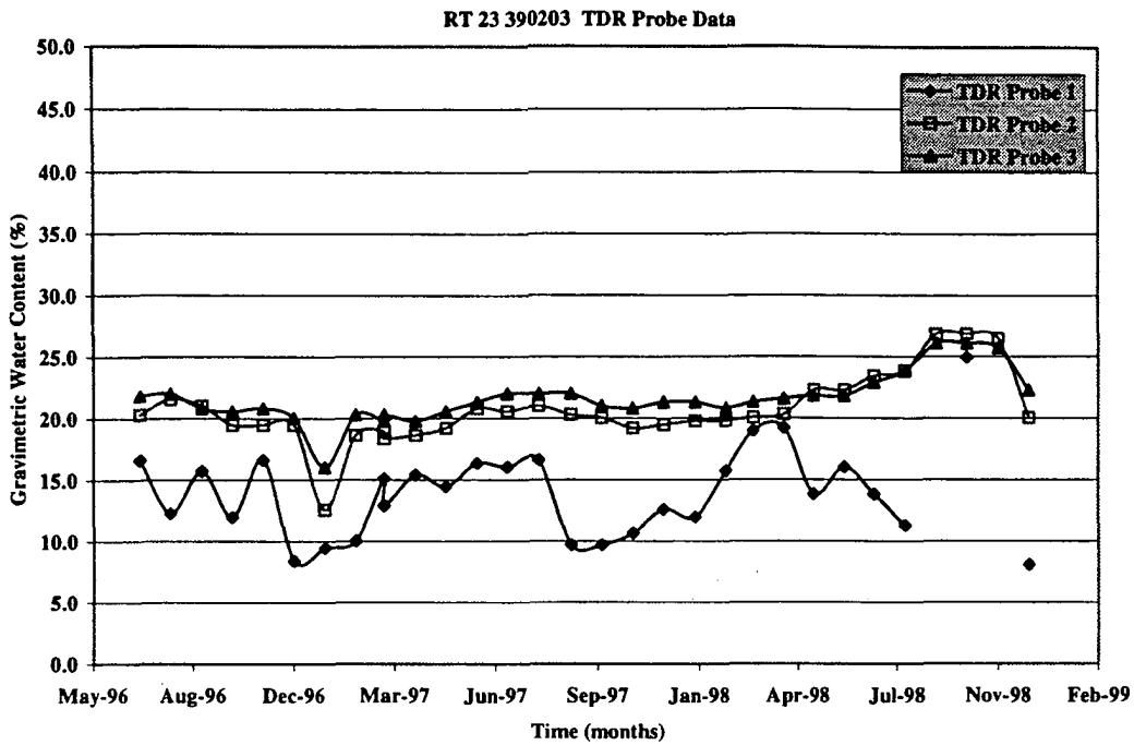
Figure 3.9: TDR Data 390203
