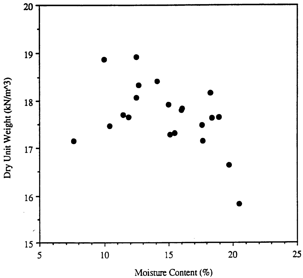
Figure 5.5.(a): Dry Unit Weight Vs. Moisture Content Plot for A-6 Soil Specimens
