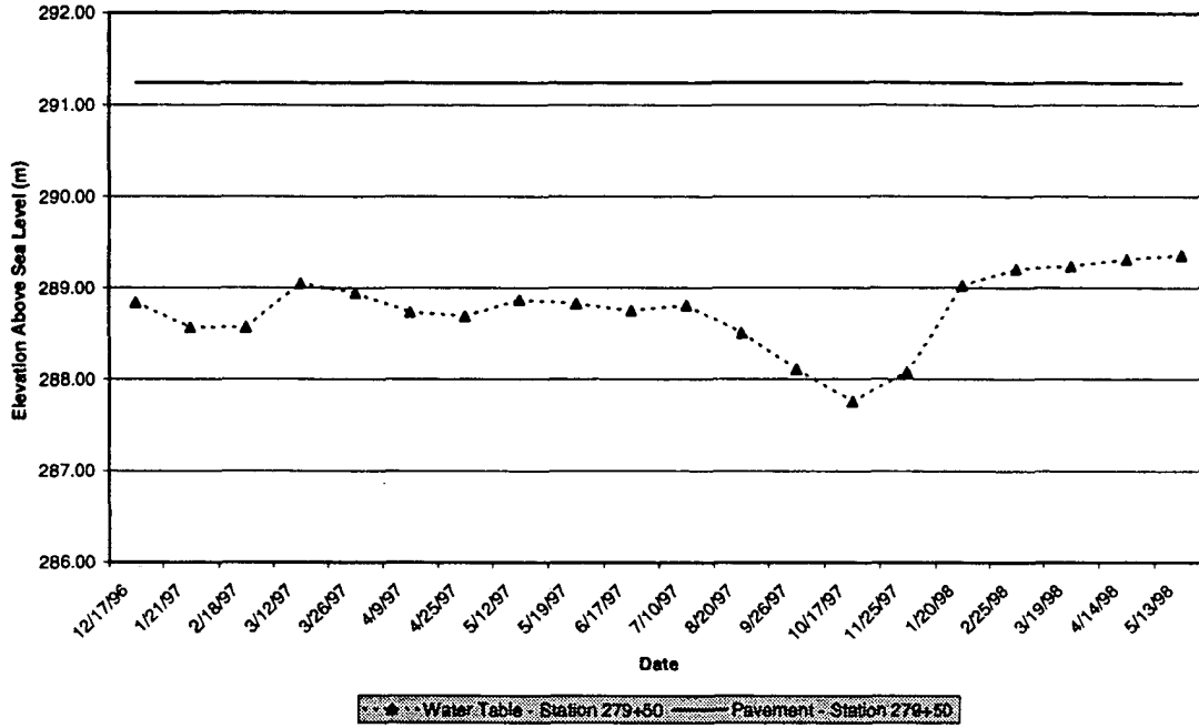
Figure 2.1: Piezometer Readings Station 279+50
