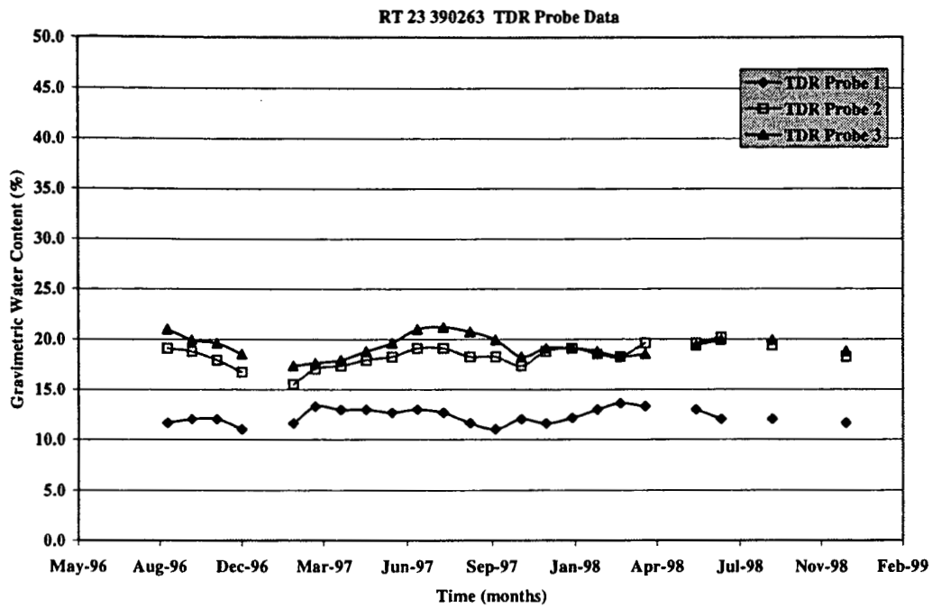
Figure 3.15: TDR Data 390263
