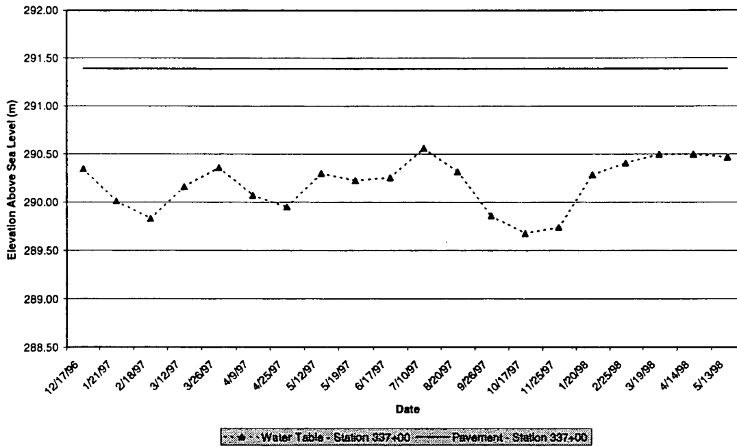
Figure 2.4: Piezometer Readings Station 337+00
