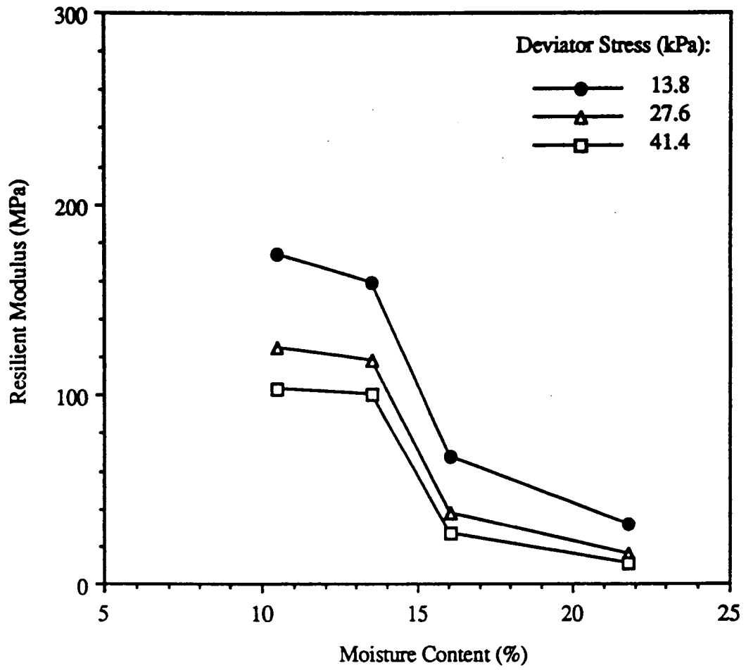
Figure 5.4.(b): Resilient Modulus Vs. Moisture Content Plot for A-7-6 Soil Specimens
