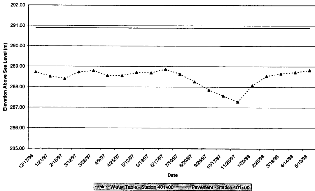
Figure 2.8: Piezometer Readings Station 401+00
