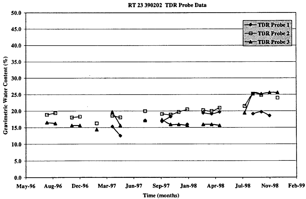
Figure 3.8: TDR Data 390202
