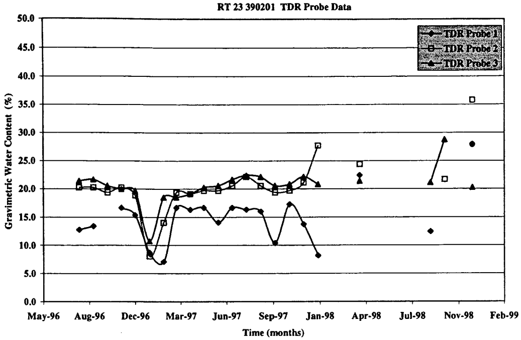
Figure 3.7: TDR Data 390201
