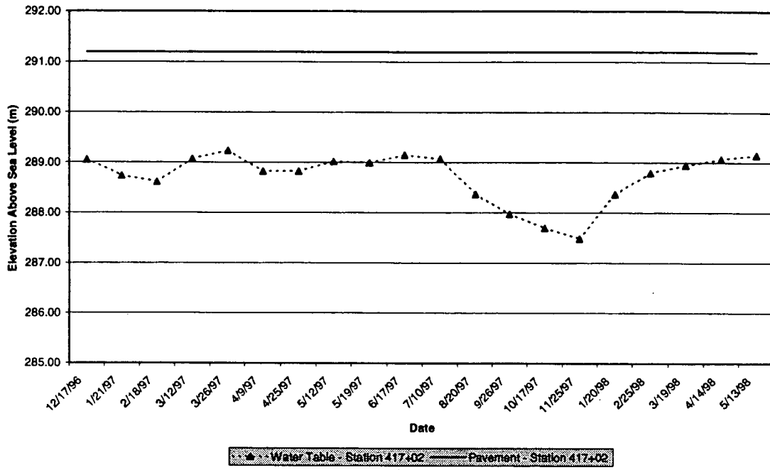
Figure 2.9: Piezometer Readings Station 417+02
