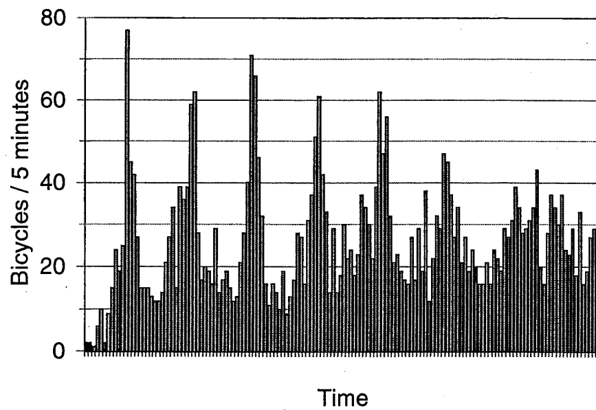
Figure 4: Time Series of 5 minute Bicycle Counts (All Locations)
