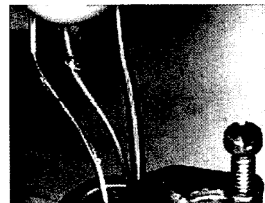
Figure 5. Wire failure mechanisms: mechanical.
