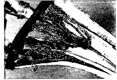
Figure 3. Wire failure mechanisms: thermal.
