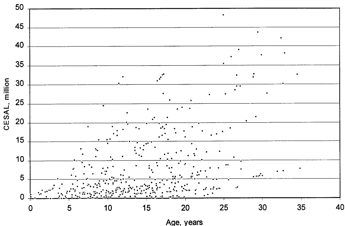
Figure 26. Distribution of CESALs with age.
