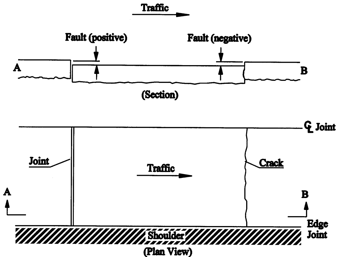
Figure 3. Faulting of transverse joints and cracks.
