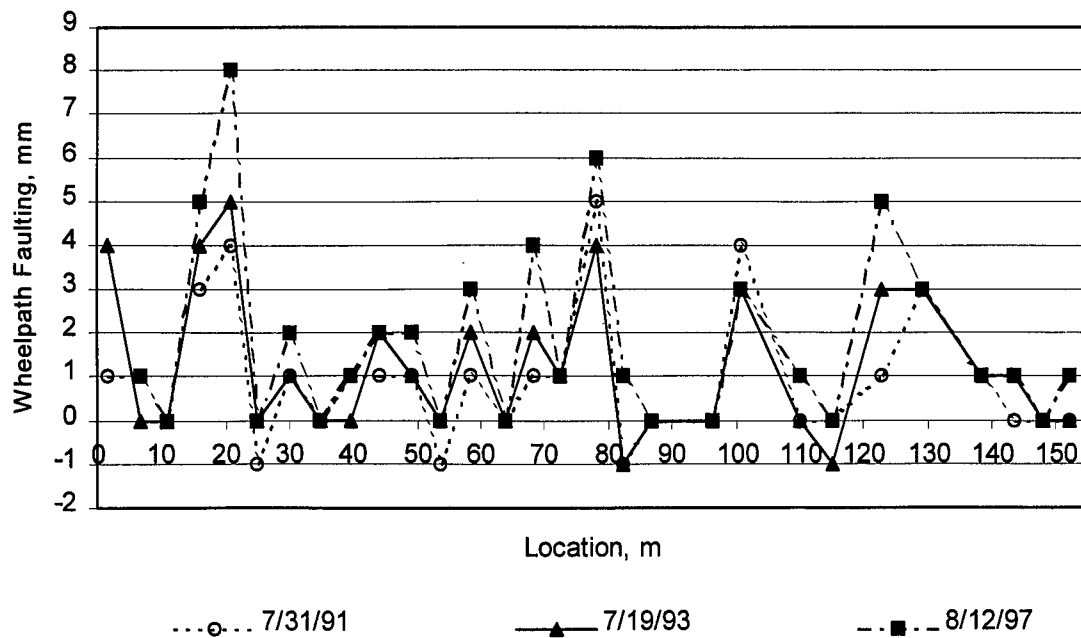
Figure 2. Example of faulting profile for GPS-4 section 314019.
