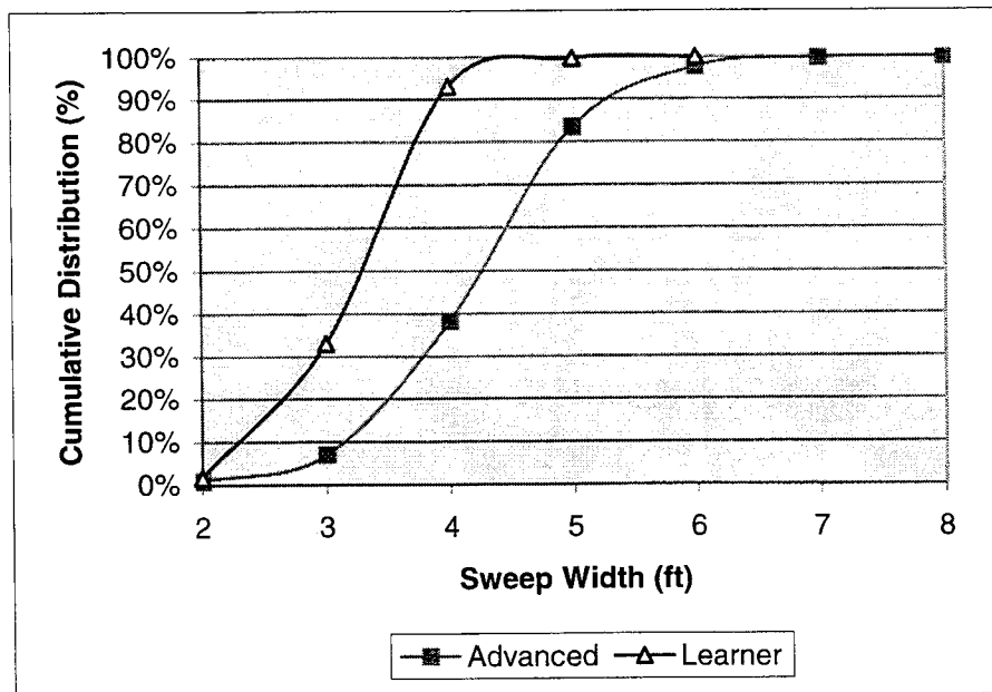
FIGURE 21 Cumulative Distribution Curves for Lower & Upper Sweep Width for Learner and Advanced Skaters
