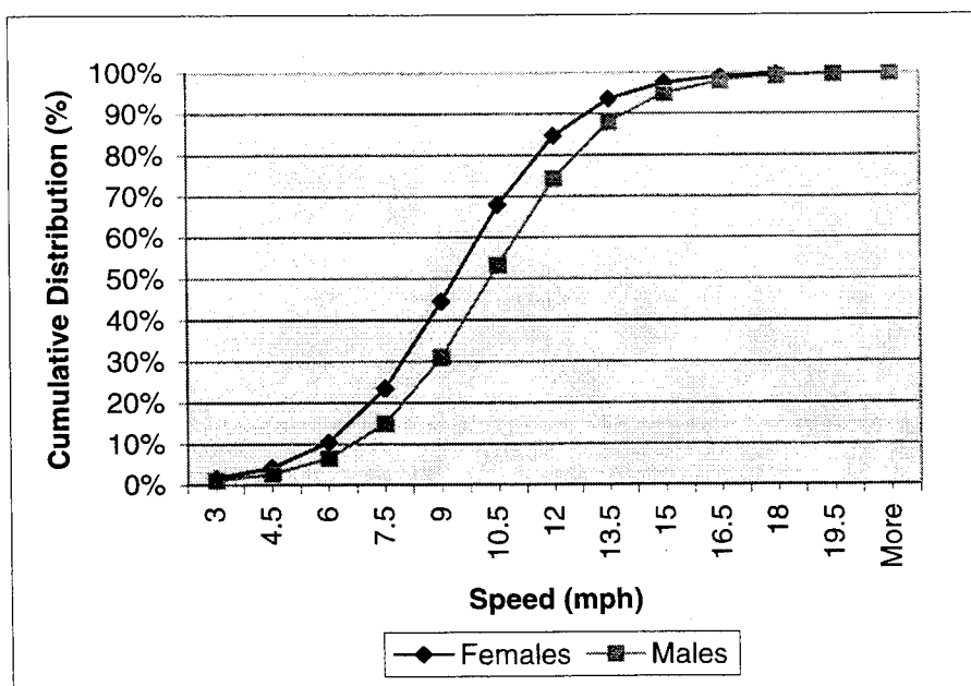
FIGURE 9 Cumulative Distribution Curves for Speed for Male and Female Skaters
