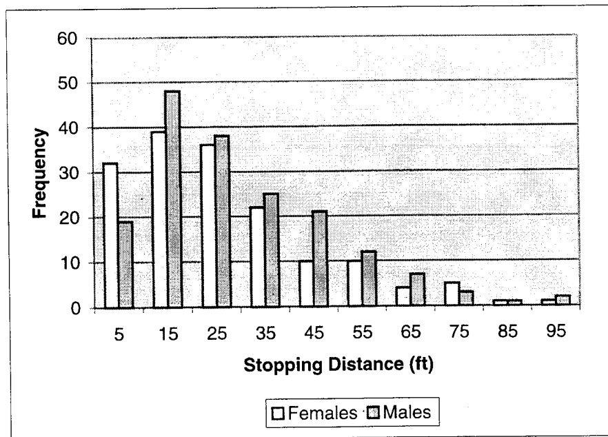
FIGURE 30 Stopping Distance Distributions for Male and Female Skaters.
