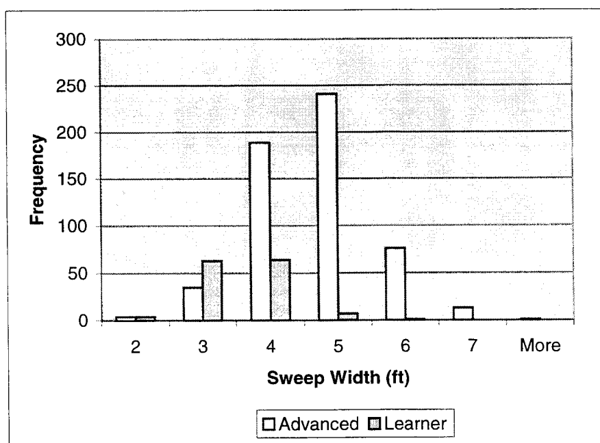
FIGURE 16 Lower Sweep Width Distributions for Learner and Advanced Skaters
