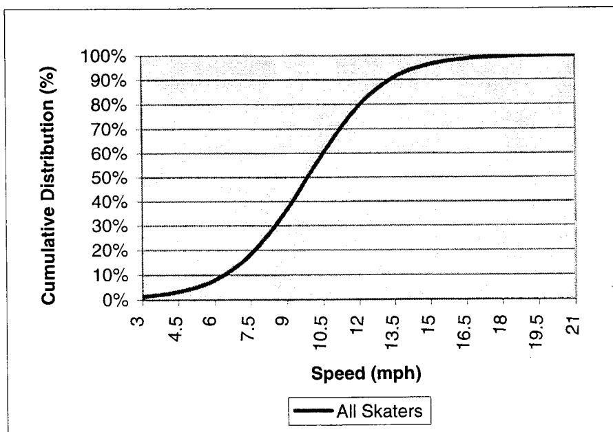
FIGURE 8 Cumulative Distribution Curve for Speed for All Skaters
