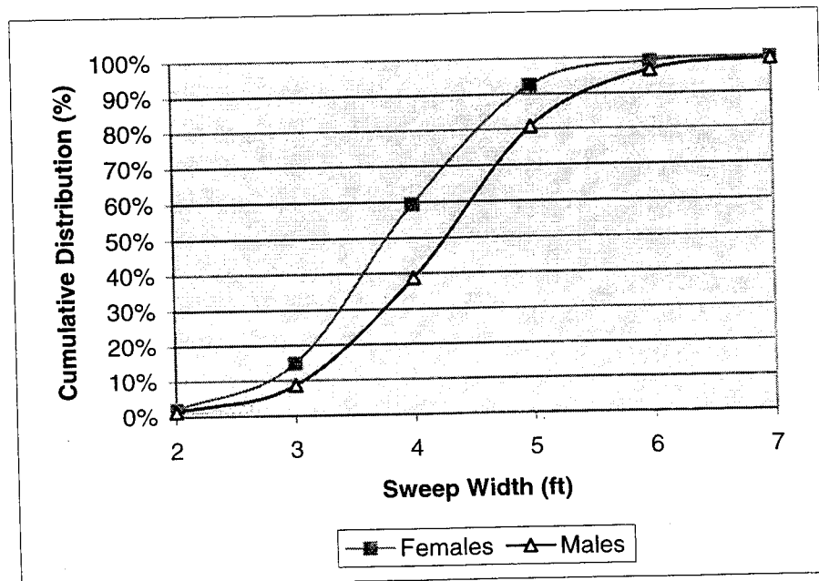
FIGURE 20 Cumulative Distribution Curves for Lower Sweep Width for Male and Female Skaters
