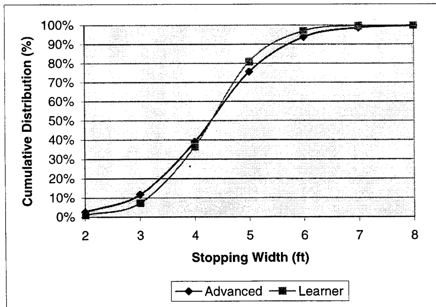
FIGURE 28 Cumulative Distribution Curves for Stopping Width for Learner and Advanced Skaters
