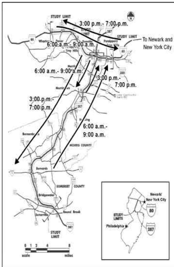
Figure 1. Location and Operation of the HOV Lanes on I-80 and I-287.
