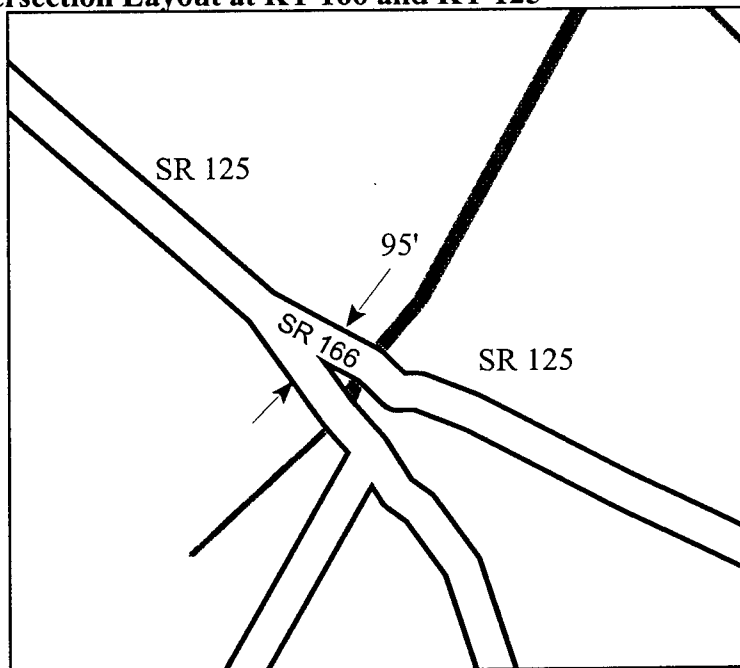
Figure 19: Intersection Layout at KY 166 and KY 125
