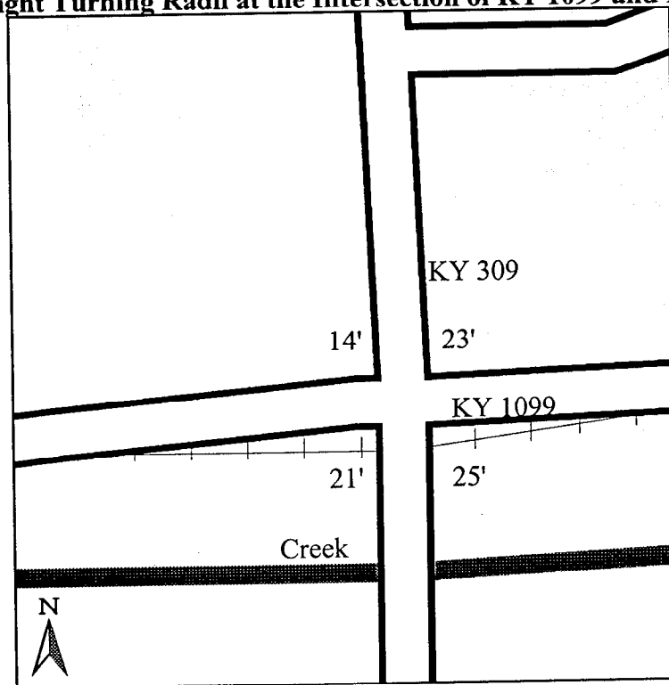
Figure 15: Right Turning Radii at the Intersection of KY 1099 and KY 309
