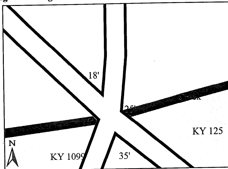
Figure 14: Right Turning Radii at the Intersection of KY 1099 and KY 125.
