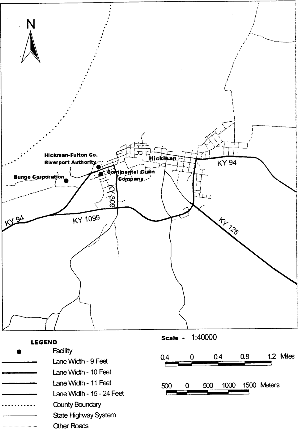
Figure 8: Lane Widths in Town of Hickman
