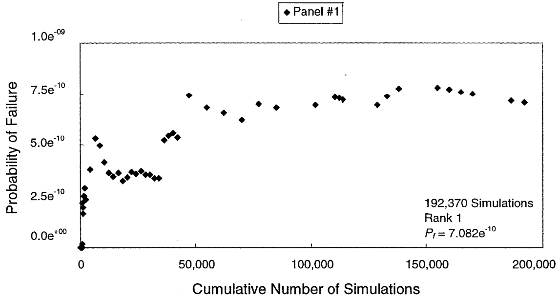
FIGURE 6. AVERAGE PROBABILITY OF FAILURE AT THE MOST CRITICAL LOCATION (panel 1 of figure 2)
