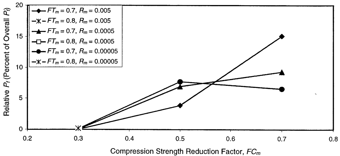
FIGURE 37. RELATIVE P_f SENSITIVITY OF MANUFACTURING DEFECT PARAMETERS AT LOCATION 28 (Critical Tension)
