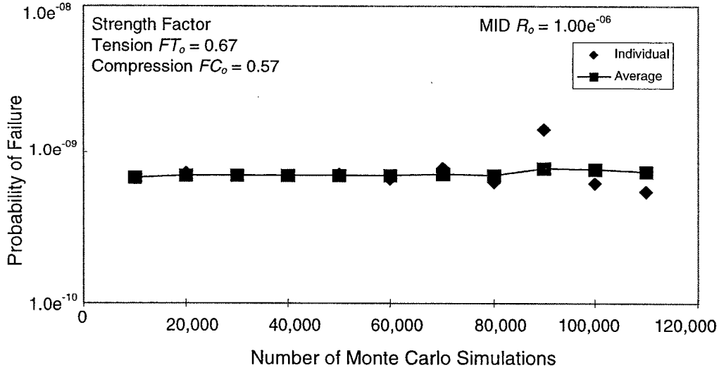
FIGURE 24. OVERALL P_f FOR R_o = 1.00e^{-06}
