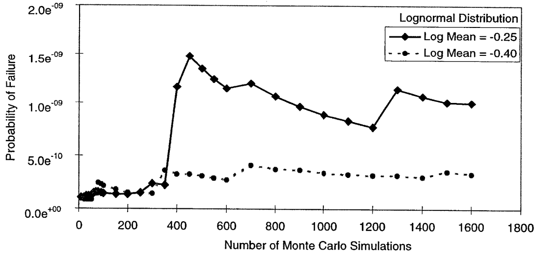
FIGURE 15. EFFECTS OF LOAD FACTOR DISTRIBUTION MEAN ON THE OVERALL PROBABILITY OF FAILURE
