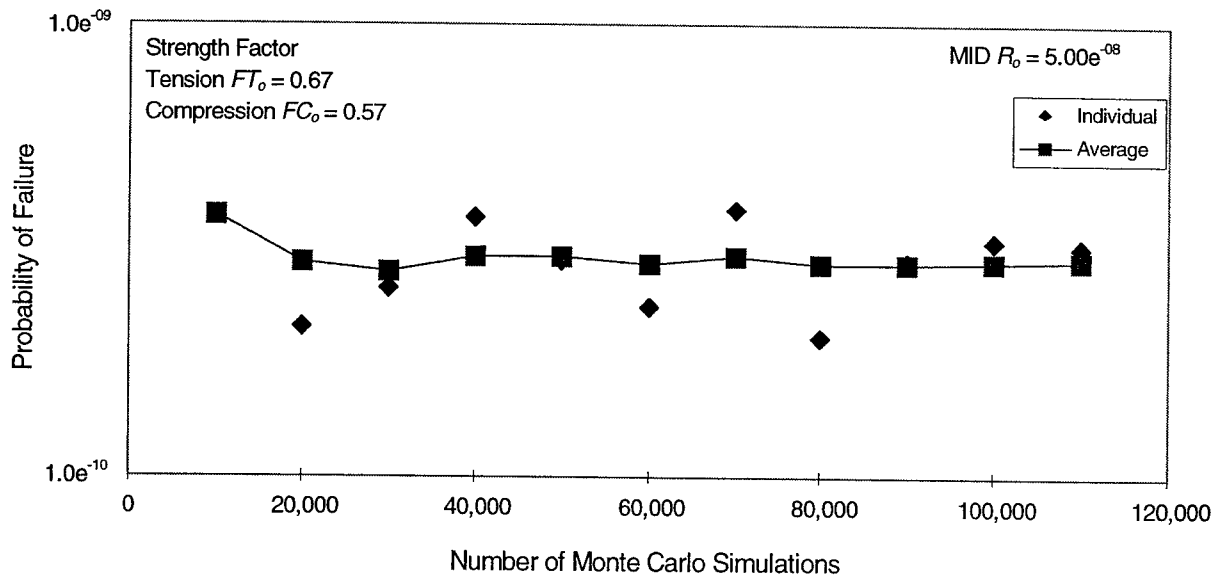
FIGURE 22. OVERALL P_f FOR R_o = 5.00e^{-08}
