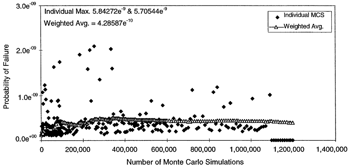
FIGURE 12. AVERAGE PROBABILITY OF FAILURE FOR THE OVERALL LEAR FAN MODEL, COMBINED RESULTS
