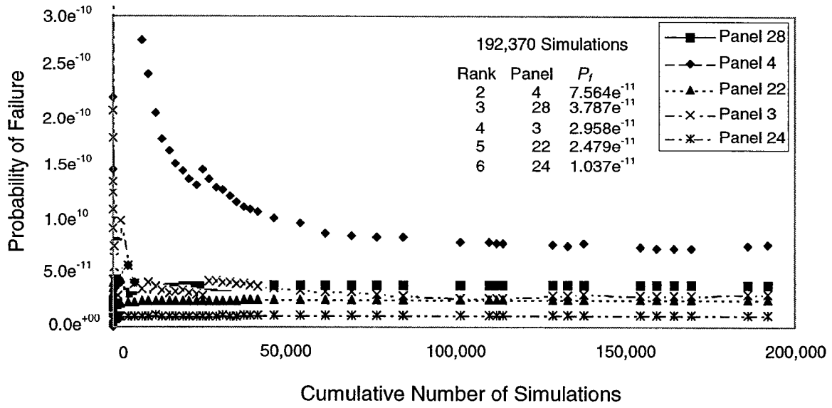
FIGURE 7. AVERAGE PROBABILITY OF FAILURE FOR GROUP 2 PANELS
