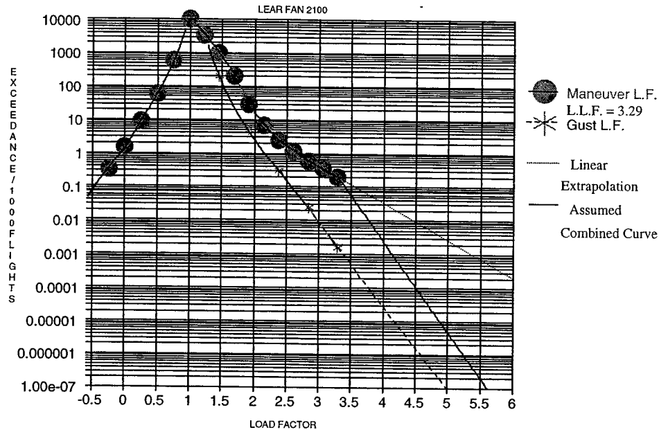
FIGURE 4. EXTRAPOLATED EXCEEDANCE CURVE FOR THE LEAR FAN ANALYSIS
