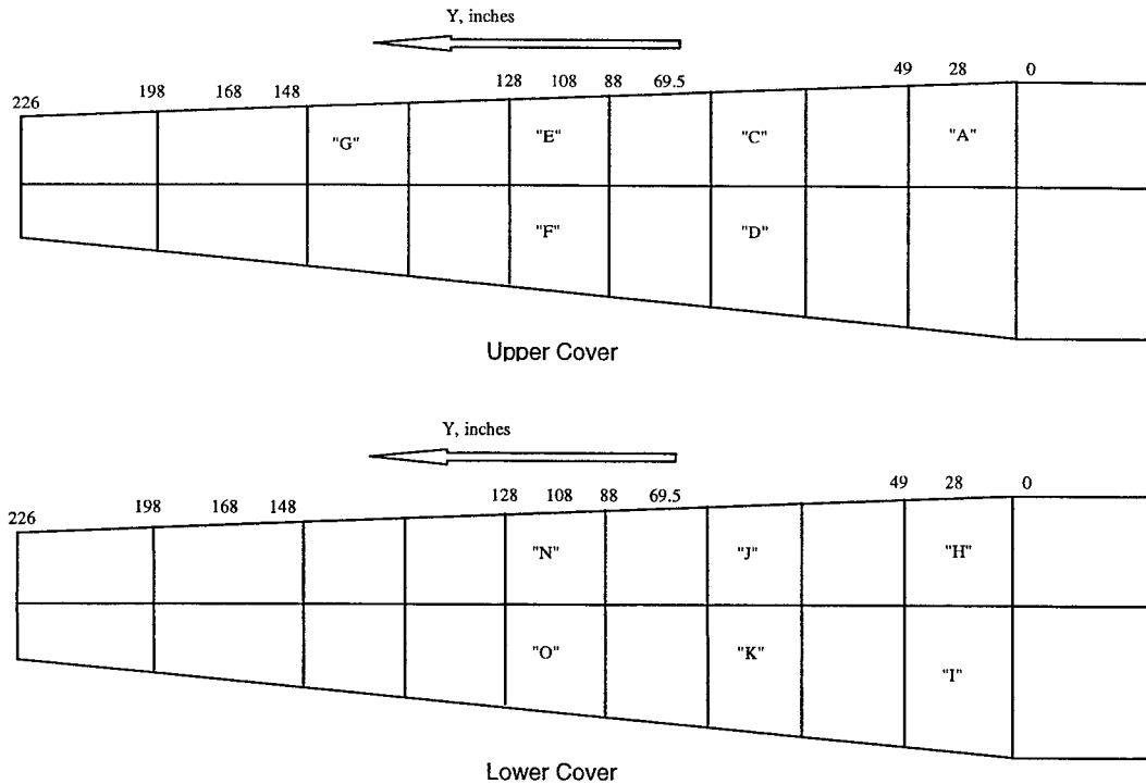
FIGURE 3. CENTRAL AEROHYDRODYNAMIC INSTITUTE MODEL OF LEAR FAN 2100 WING [12]
