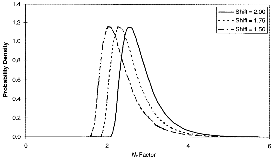
FIGURE 18. SKIN LOAD FACTOR DISTRIBUTIONS WITH VARIABLE SHIFT FACTOR IN THE LOGNORMAL DISTRIBUTION
