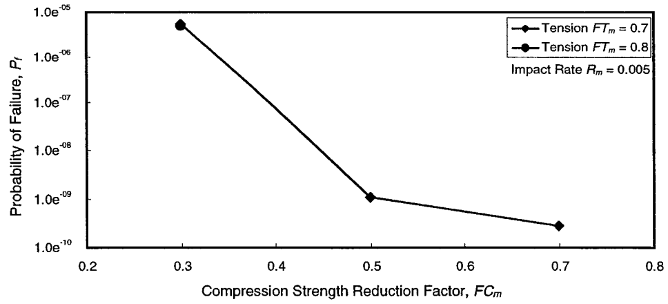
FIGURE 33. INFLUENCE OF THE MANUFACTURING DEFECT PARAMETERS ON P_f , R_m = 0.005
