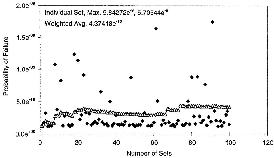
FIGURE 10. AVERAGE PROBABILITY OF FAILURE FOR THE OVERALL LEAR FAN MODEL, BASED ON 1000 SIMULATIONS IN EACH SET
