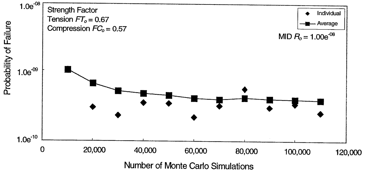
FIGURE 20. OVERALL P_f FOR R_o = 1.00e^{-08}
