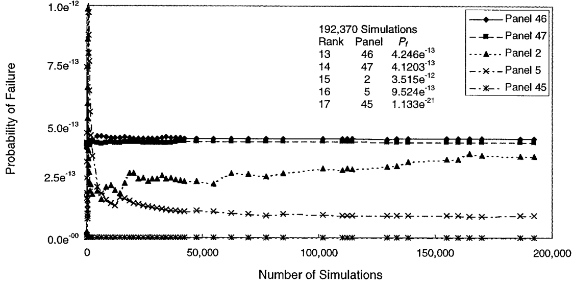
FIGURE 9. AVERAGE PROBABILITY OF FAILURE FOR GROUP 4 PANELS
