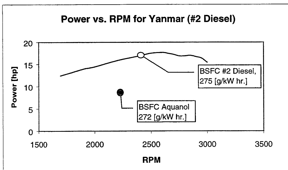
Figure 12. Lugging curve with BSFC data points.
