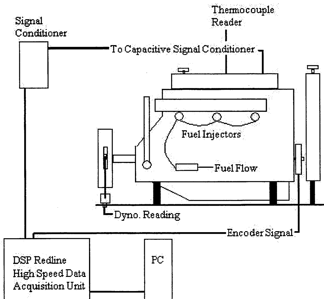
Figure 7. Experimental apparatus.
