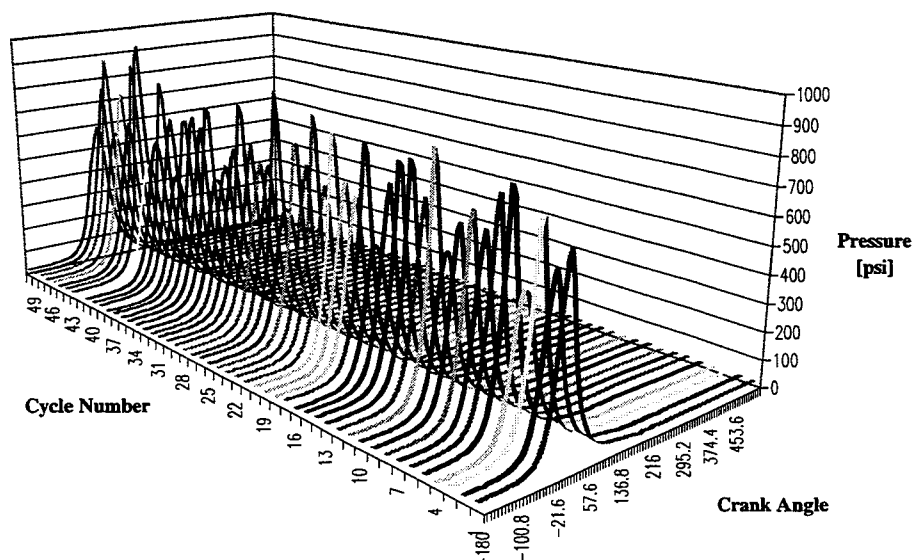
Cycle to Cycle Pressure Variation
