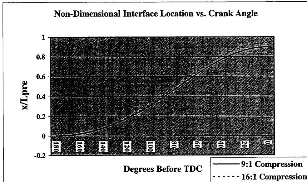
Figure 3. Interface location as a function of crank angle.
