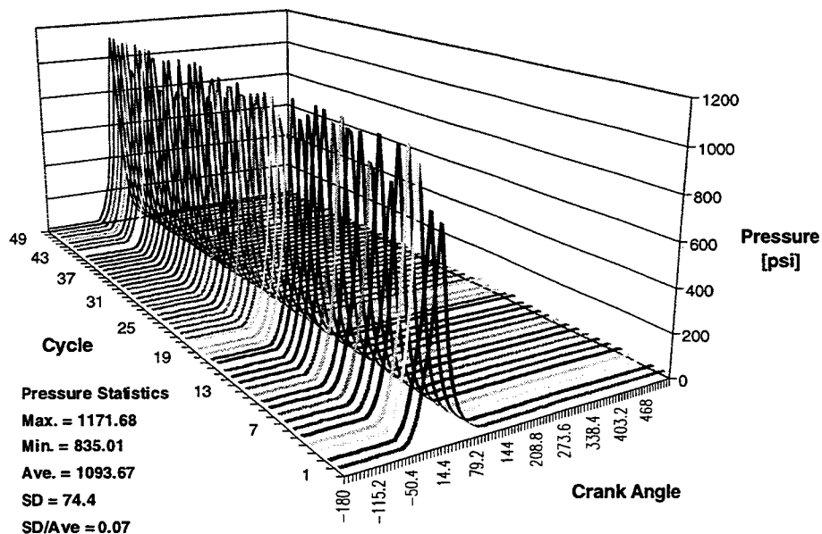
Figure 11. 50-Cycle pressure vs. crank angle traces for shorter igniters, x/L_{pre}=0.63 , 30 percent H_2O , 2000 rpm, 10-hp.
