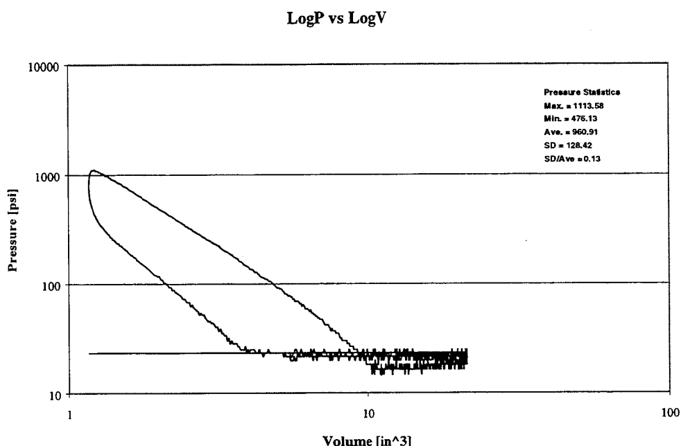
Figure 9. LogP vs. LogV, x/L_{pre}=0.63 , 30 percent H_2O , 2000 rpm, 10-hp
