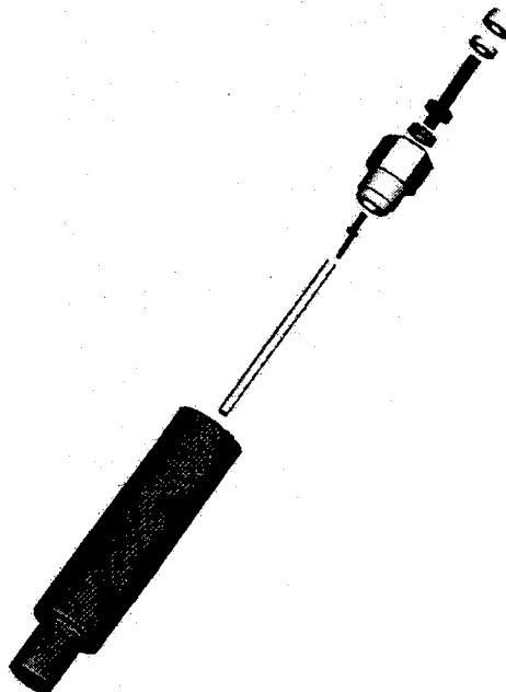
Figure 5. Improved CPT design.
