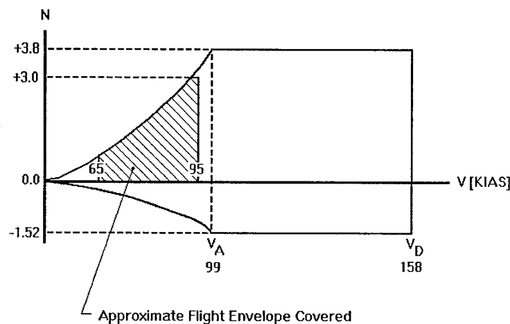
FIGURE 7. APPROXIMATE FLIGHT ENVELOPE COVERED
