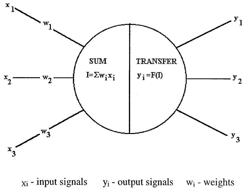
FIGURE 1. PROCESSING ELEMENT
