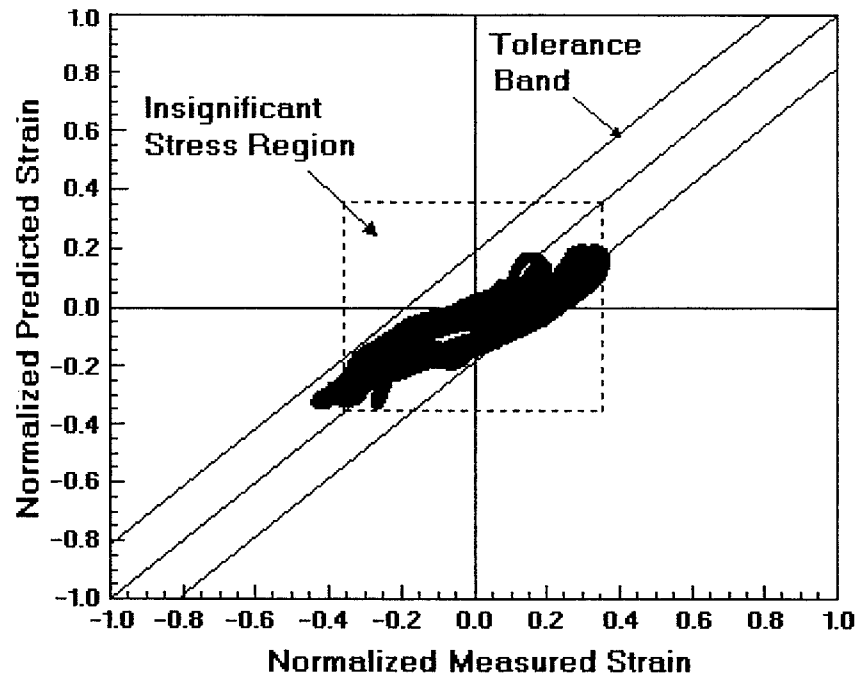
FIGURE 12. DUTCH ROLL, 95 KIAS, HORIZTONTAL TAIL, TRAINING SET— STRAIN PREDICTION RESULTS
