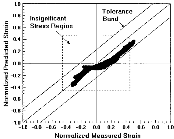
FIGURE 20. DUTCH ROLL, 65 KIAS, VERTICAL TAIL, TRAINING SET—STRAIN PREDICTION RESULTS
