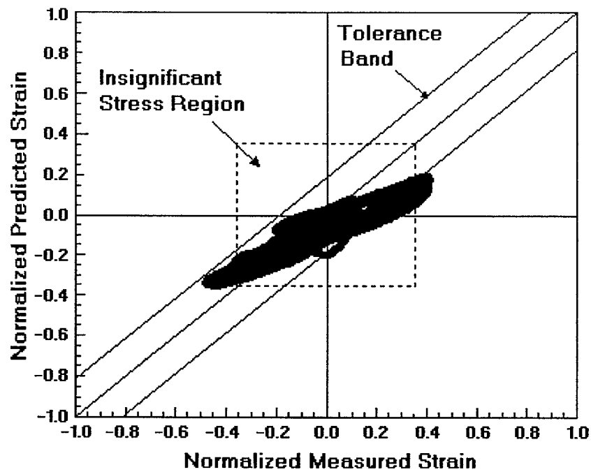
FIGURE 13. DUCTH ROLL, 95 KIAS, HORIZTONTAL TAIL, TESTING SET— STRAIN PREDICTION RESULTS
