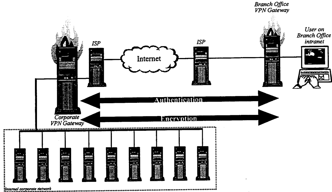
Figure 2-3 Branch Office VPN
