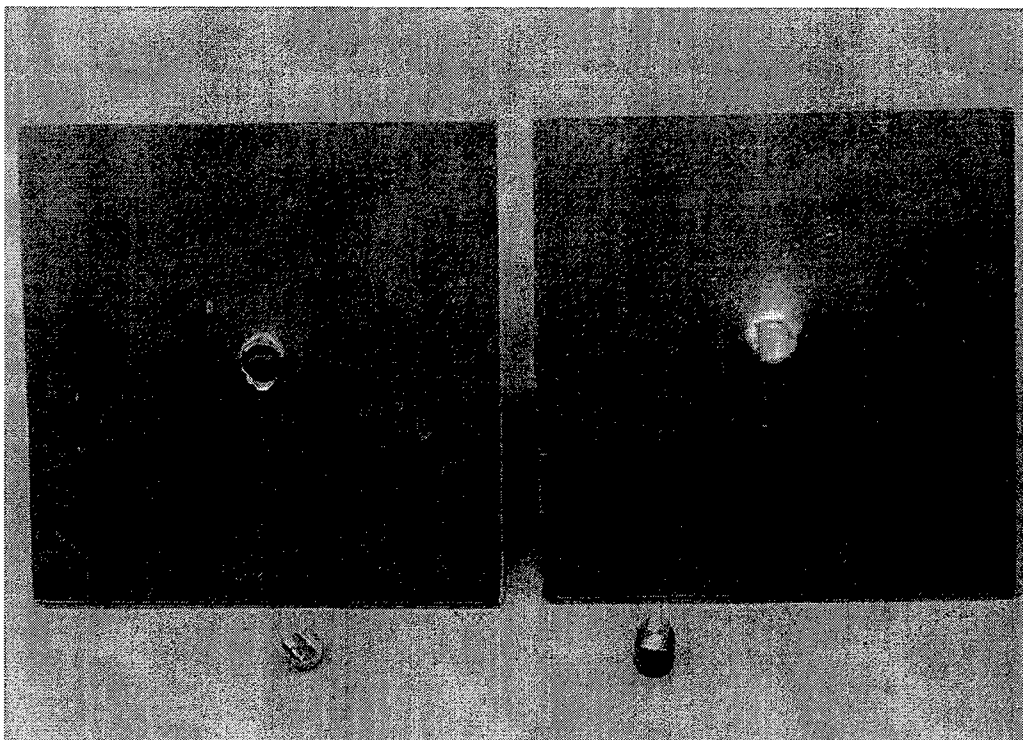
FIGURE 6. TYPICAL (0.150-inch-THICK) ALUMINUM PLATES —REAR FACE (FAA-14 plug failure on left)
