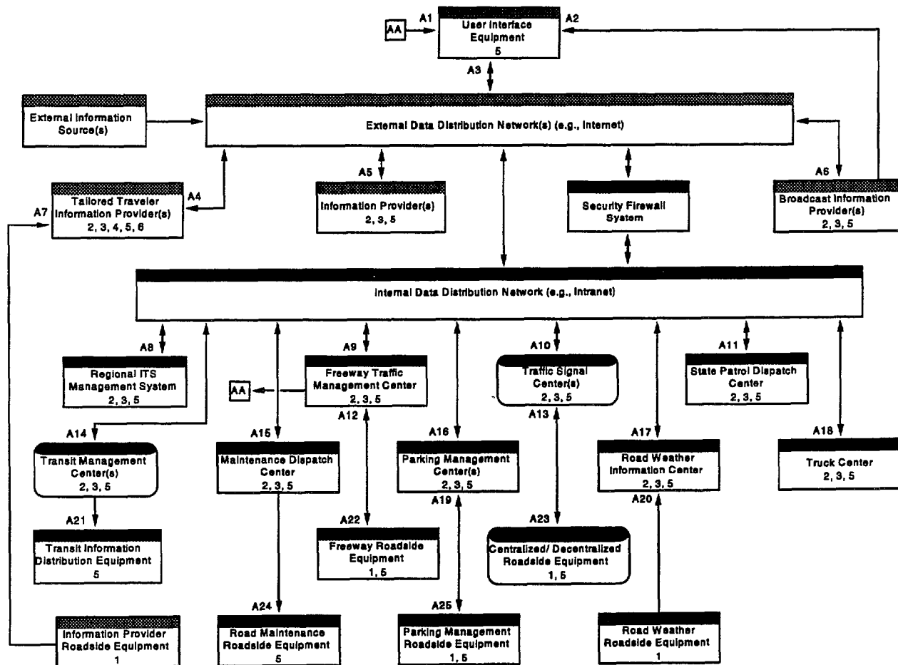
Figure 90. Travel Conditions Information - Physical Architecture
