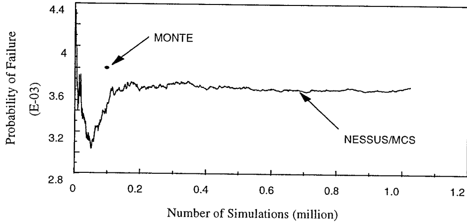
FIGURE 9. PROBABILITY OF FAILURE FOR CASE 4-1
