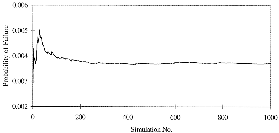
FIGURE 15. AVERAGE FAILURE PROBABILITY FOR CASE 5-1
