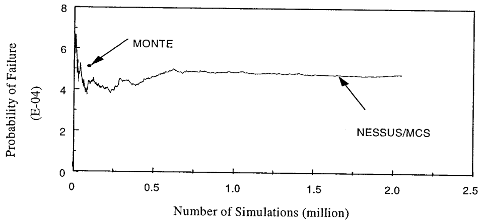
FIGURE 11. PROBABILITY OF FAILURE FOR CASE 4-3
