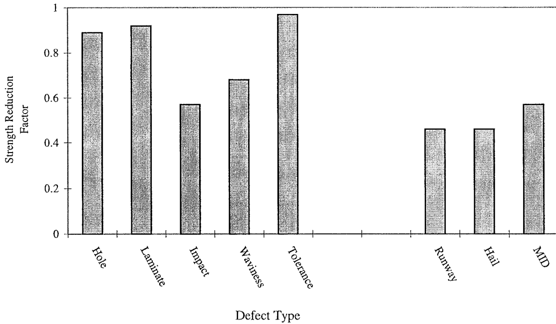
FIGURE 7. STRENGTH REDUCTION DUE TO MANUFACTURING AND OPERATIONAL DEFECTS
