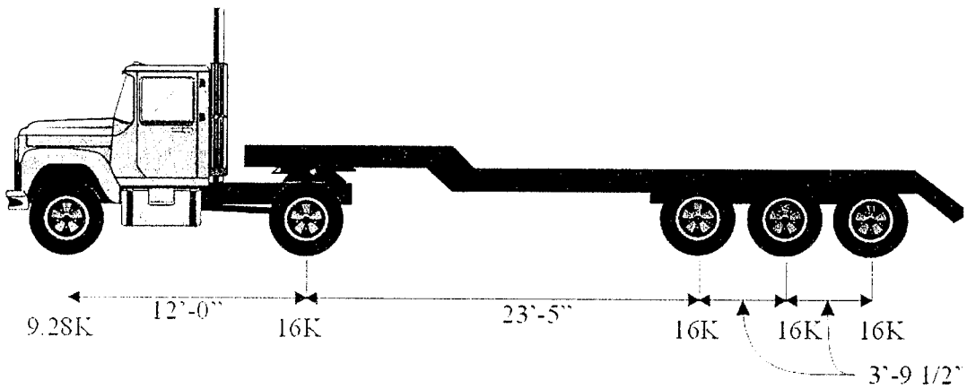
Figure 2.9. Truck MO5
