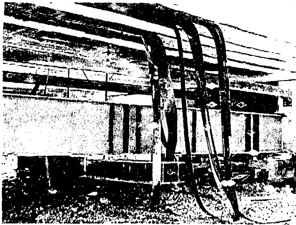
(b) Peeling of CFRP sheets
