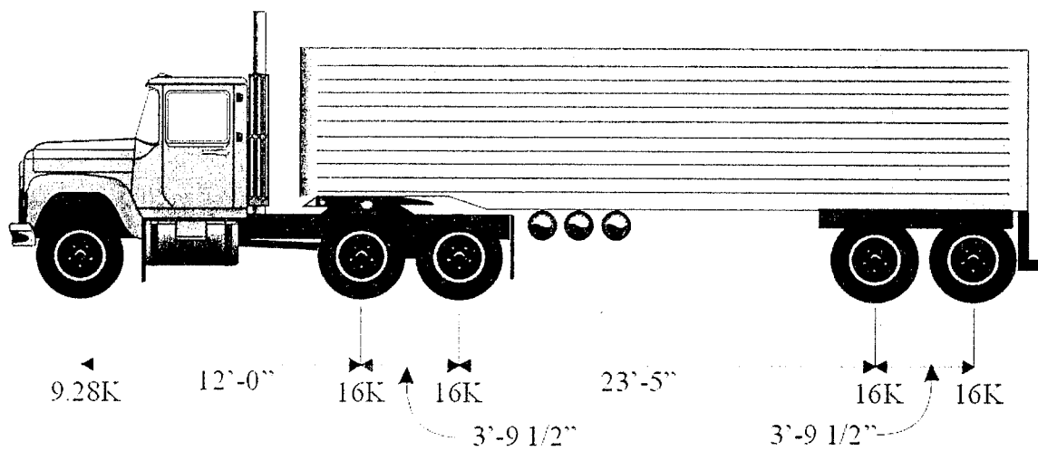
Figure 2.7. Truck 3S2
