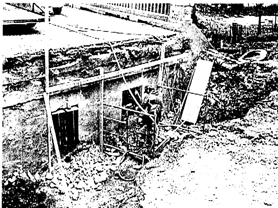
Figure 4.11. Bridge abutment after excavation and cutting.
