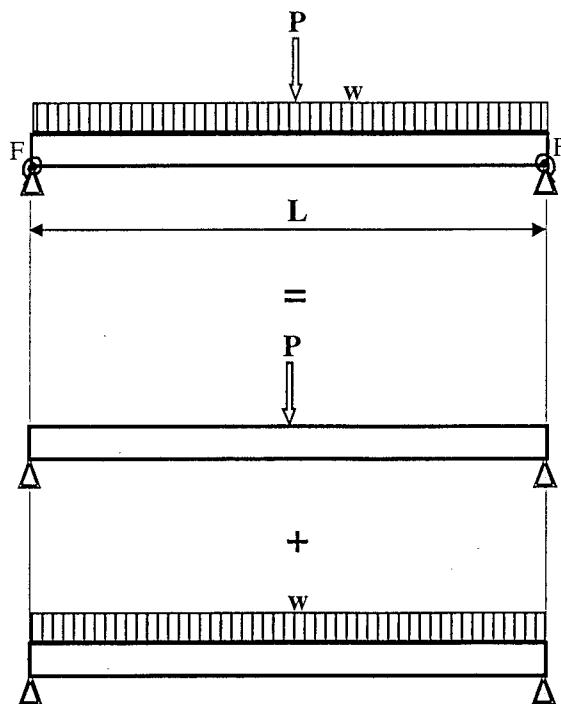
Figure D.1. Superposition of the deck loading.
