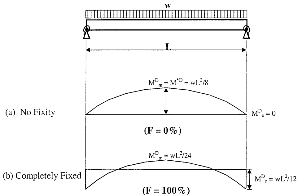
Figure D.3. Moment diagrams for a flexural beam under distributed load with various end conditions.
