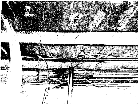
(c) Close up showing peeling of CFRP sheets
