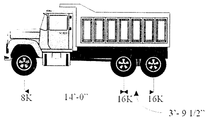
Figure 2.10. Truck H20
