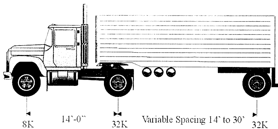
Figure 2.6. Truck HS20
