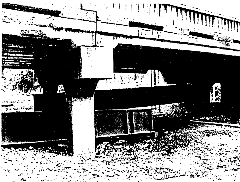
Figure 4.12. Installation of the steel girders.
