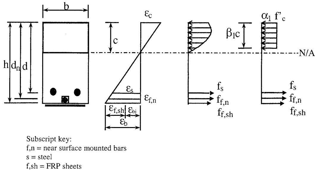
Figure 6.1. Strain and stress conditions of a RC section strengthened with FRP reinforcement.
