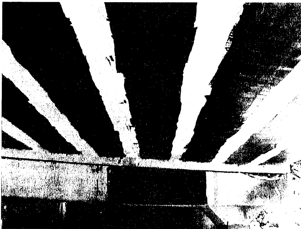
Figure 3.10. Deck 2 after strengthening with CFRP sheets.
