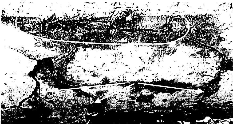
(b) Cross section through the deck showing concrete crushing
