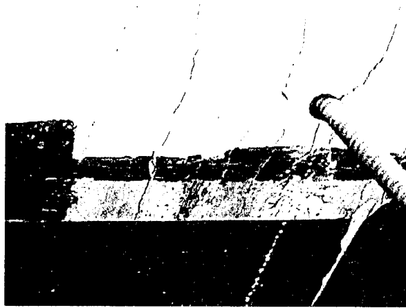
(a) Rupture of CFRP at formlines
