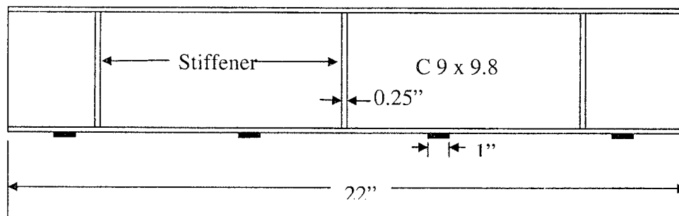
(b) Side view of a distribution beam
