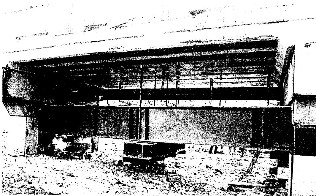
Figure 4.14. Assembled test setup for the middle deck (deck 2).
