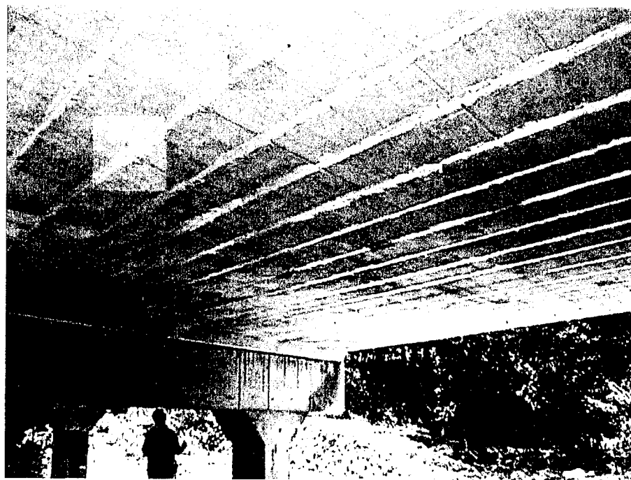
Figure 3.8. Deck 1 after strengthening with NSM rods.
