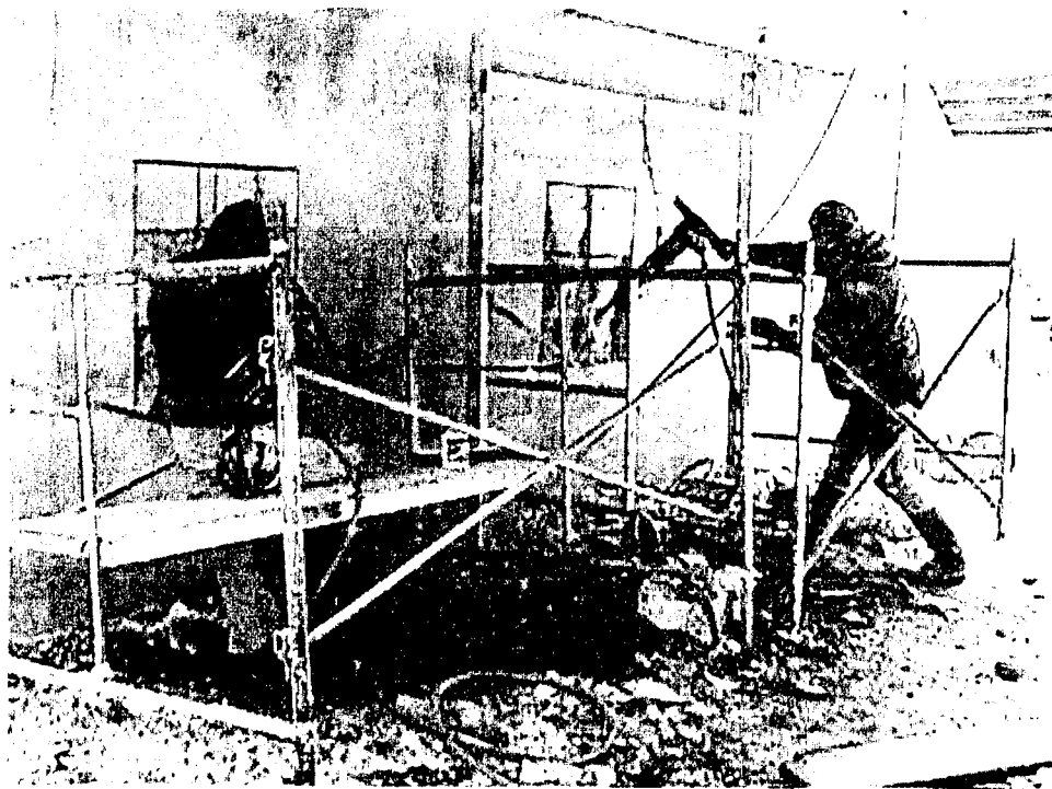
Figure 4.9. Cutting the bridge abutment.
