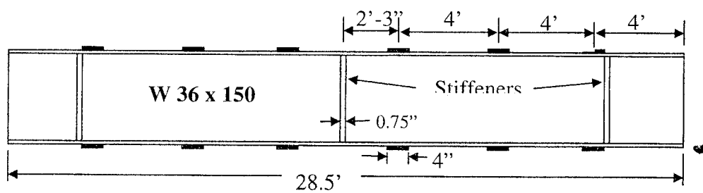
(b) Side view of a girder
