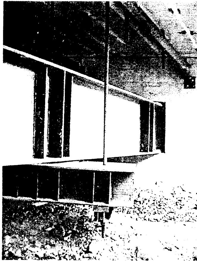
Figure 4.13. Assembled test setup for an end deck.
