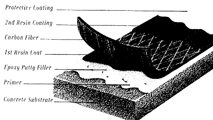
Figure 3.2. Components of the MBrace FRP composite strengthening system.
