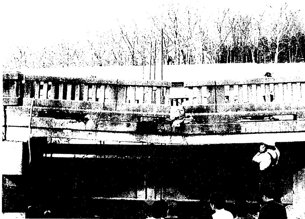
Figure 5.17. Deck 3 at failure.
