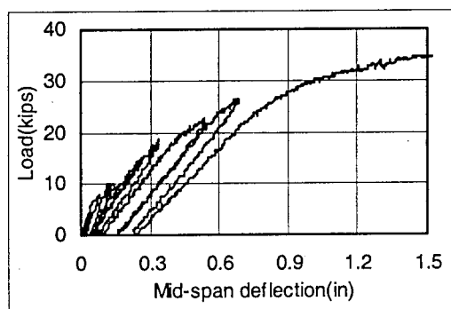
Figure 4.3 Load versus midspan deflection of Beam 3
