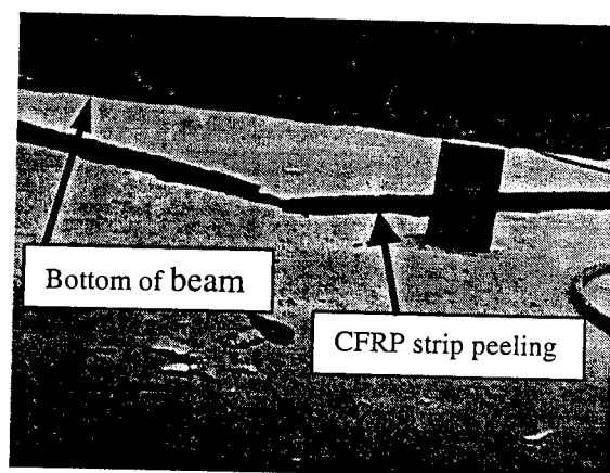
Figure 4.17 Peeling of a CFRP strip
