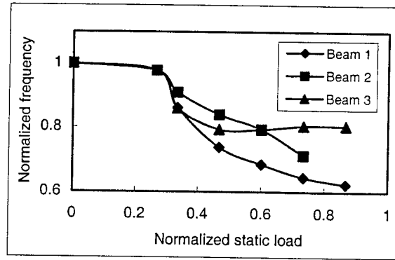
Figure 4.7 Fundamental frequency of beams
