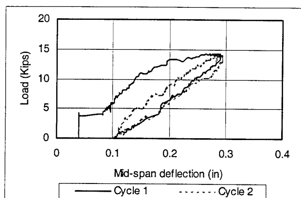
Figure 4.4 Stiffness degradation of Beam 1 ( P_s=14 kips)
