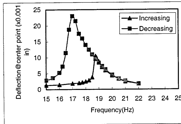
(c) Beam 3 ( P_s=22 kips)
