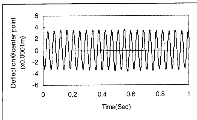
Figure 4.10 Time history response of beam
