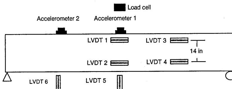
Figure 3.5 Location of transducers
