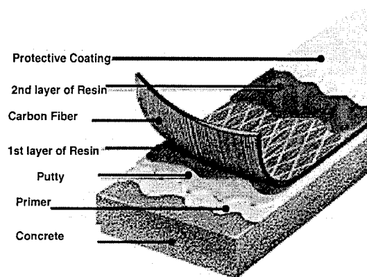
Figure 3.6 CFRP strengthening system
