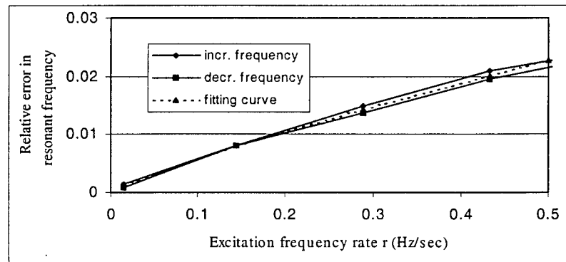
Figure 6.5 Effect of excitation frequency rate on resonant frequency
