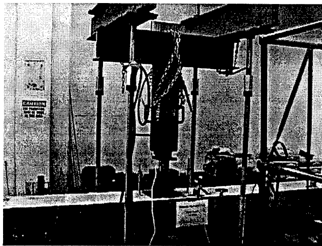
Figure 3.3 Static test setup
