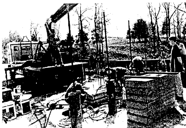
Figure 5.4 Preloading before dynamic tests
