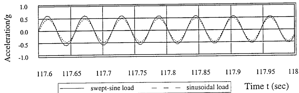
Figure 6.3 Response comparison under swept-sine and sinusoidal loads
