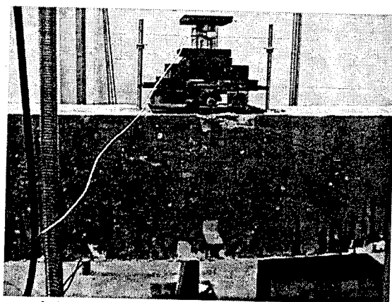
Figure 4.16 Failure of a CFRP strengthened beam
