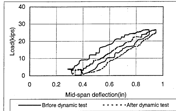
Figure 4.5 Dynamic effect on beam responses ( P_s=26 kips)
