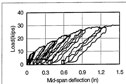
Figure 4.1 Load versus midspan deflection of Beam 1
