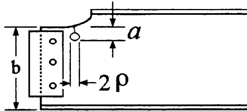
Figure 17. Dimensions for Computing Required Hole Diameter, 2\rho
