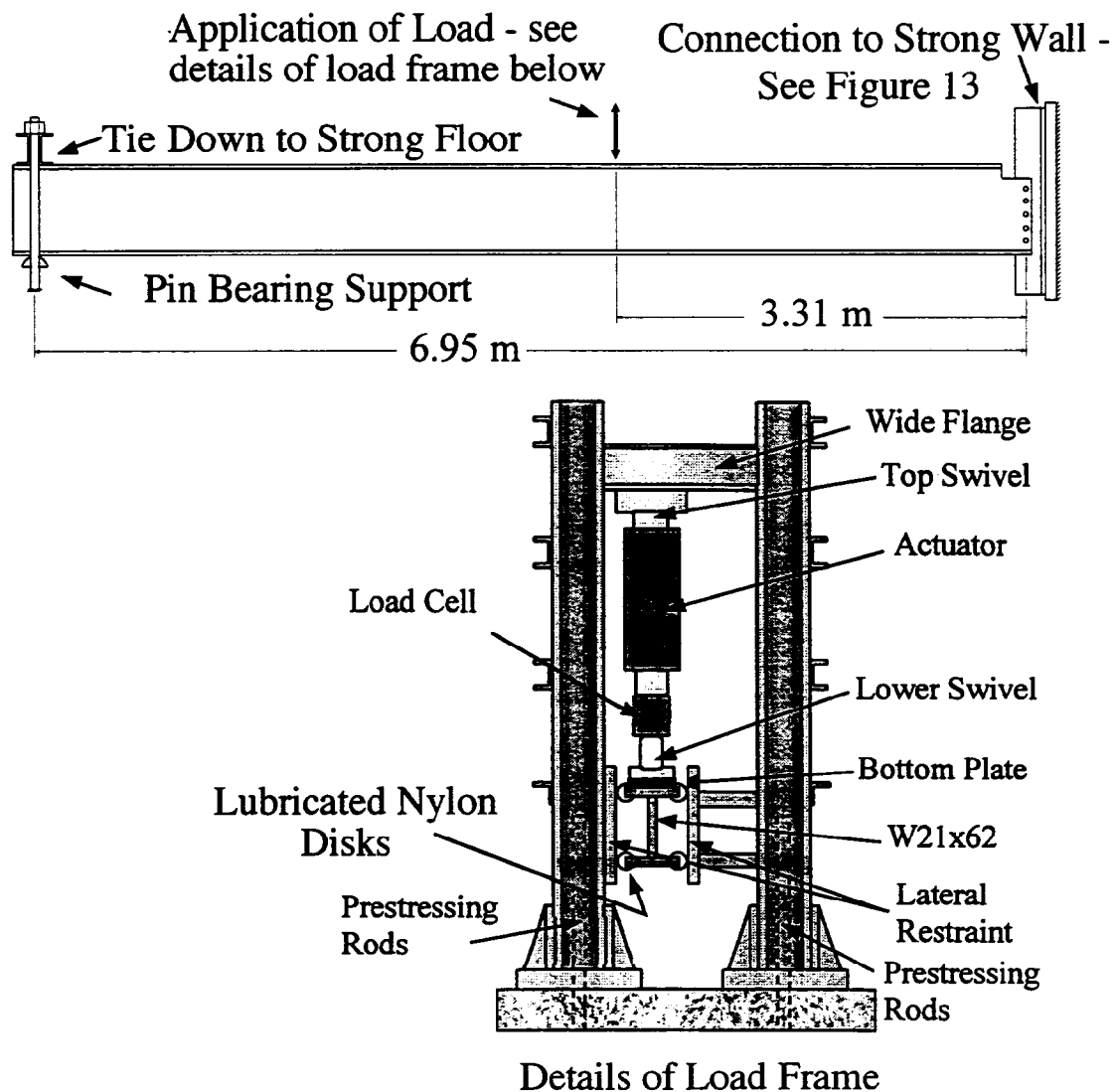
Figure 12. Test Set-Up
