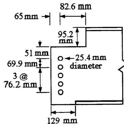
Figure 36. Lewis River Bridge Stringer Detail
