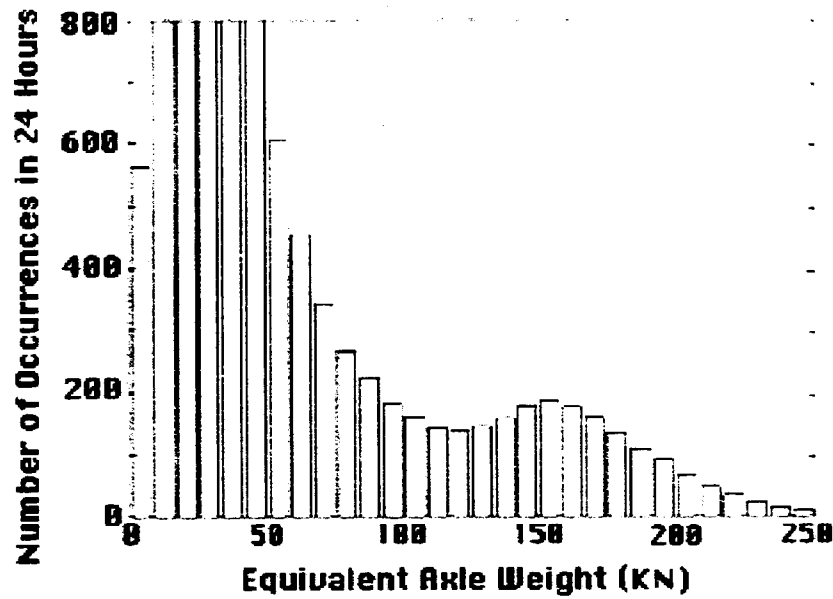
Figure 31. Histogram of Axle Load Variation Measured on the Lewis River Bridge
