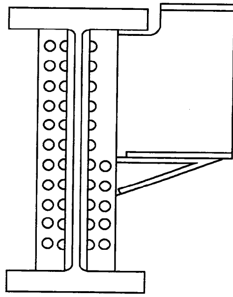
b) Stiffened Seat Connection
