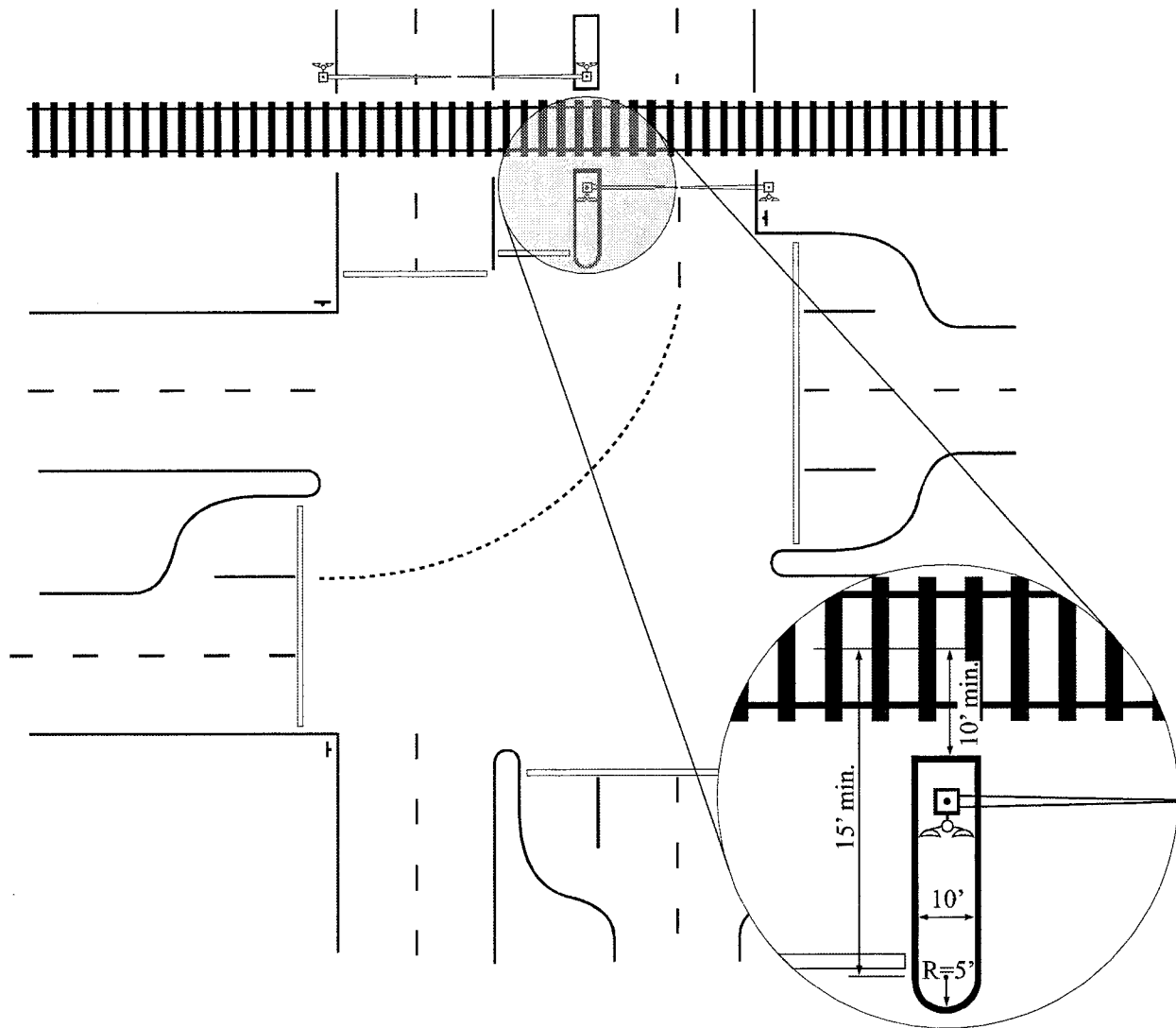
Figure 5. Channelization Design with Clearance to Turning Vehicle.
