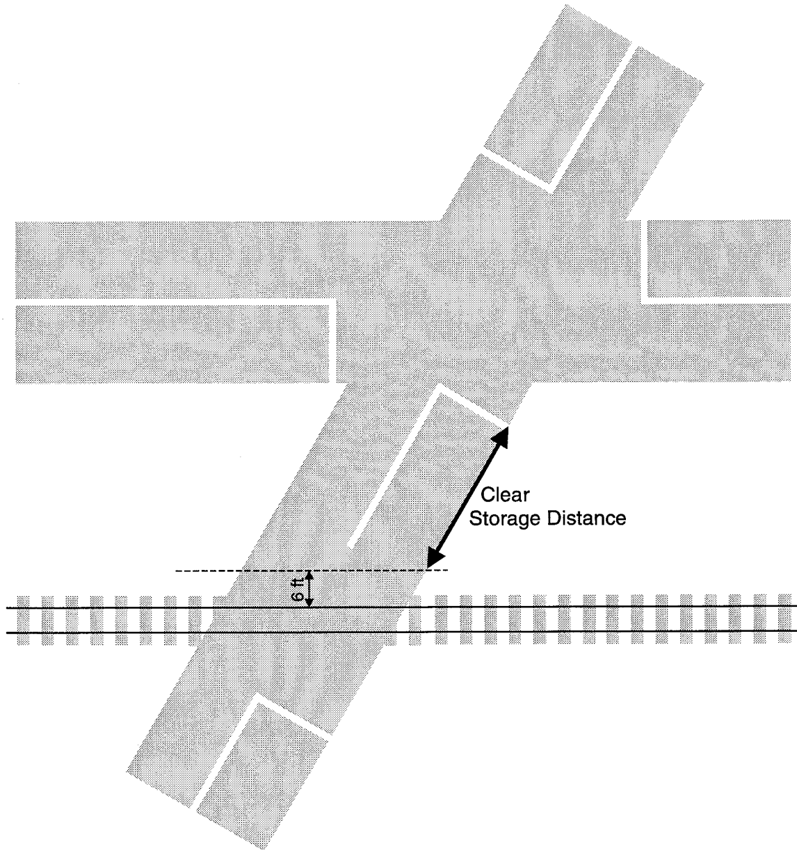
Figure 3. Clear Storage Distance at Skewed Crossings.
