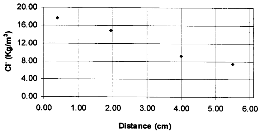
Chloride content vs distance from inside surface
