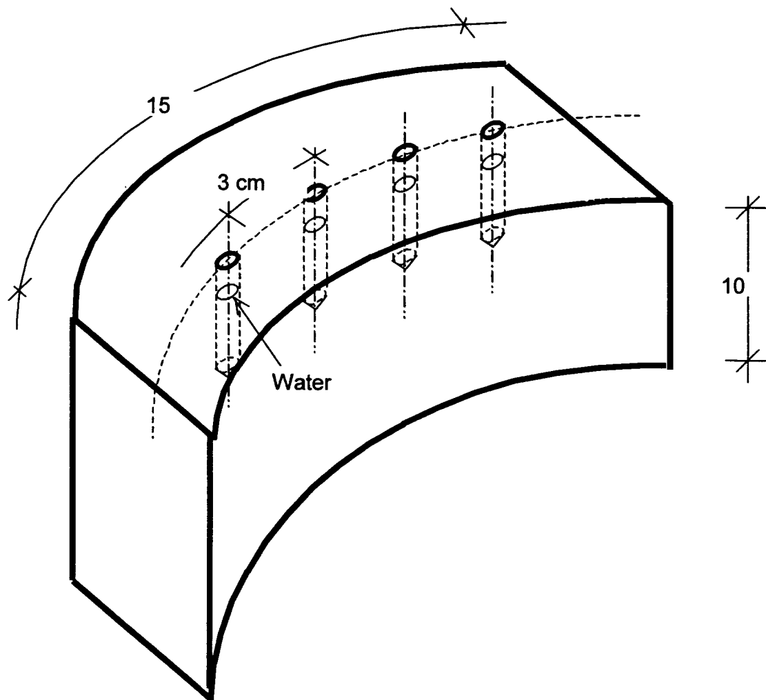
Figure 2. Concrete Culvert Segment for Pore Water pH Measurements. Note: Plastic toppers are not represented in this
