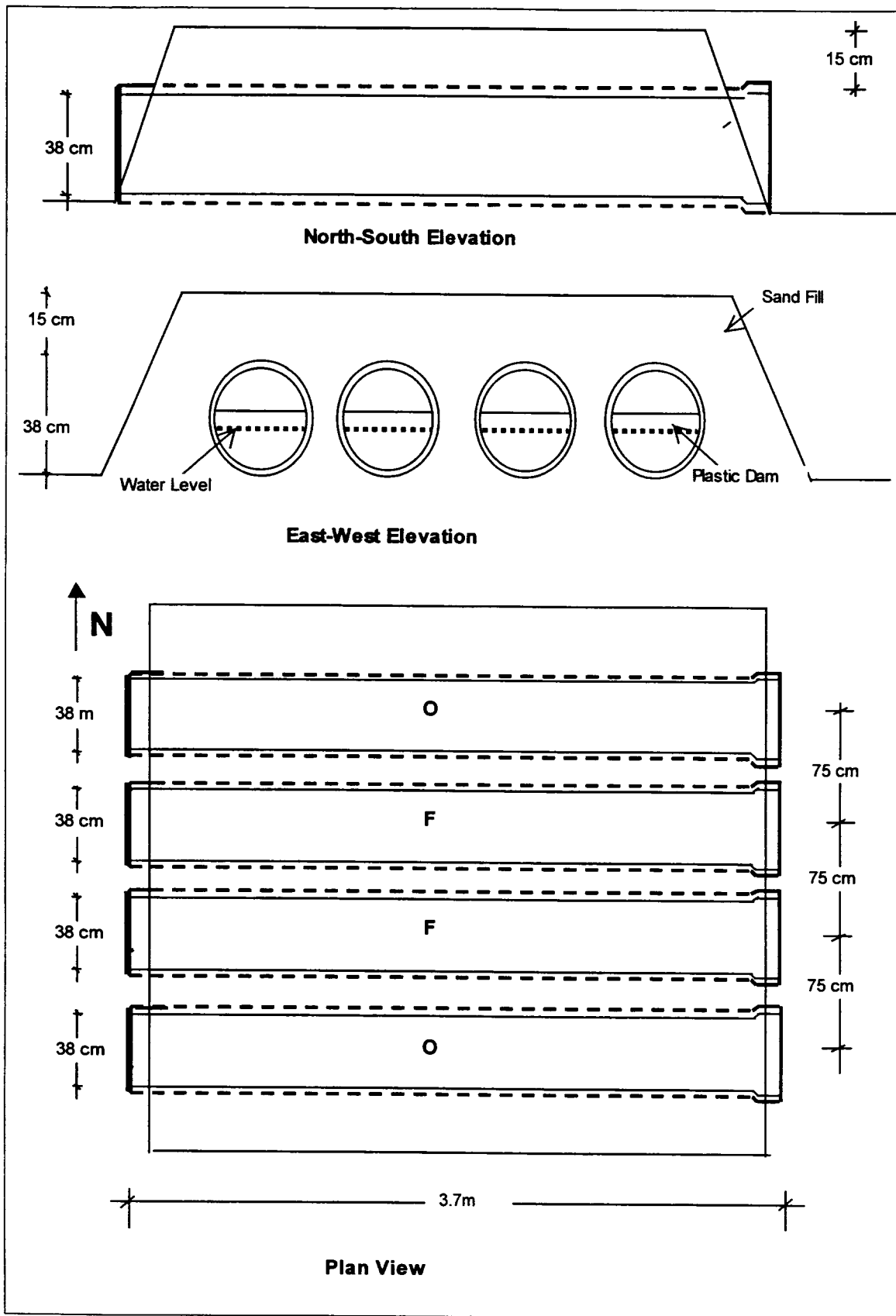
Figure 12. Culvert Yard Test Set up.
