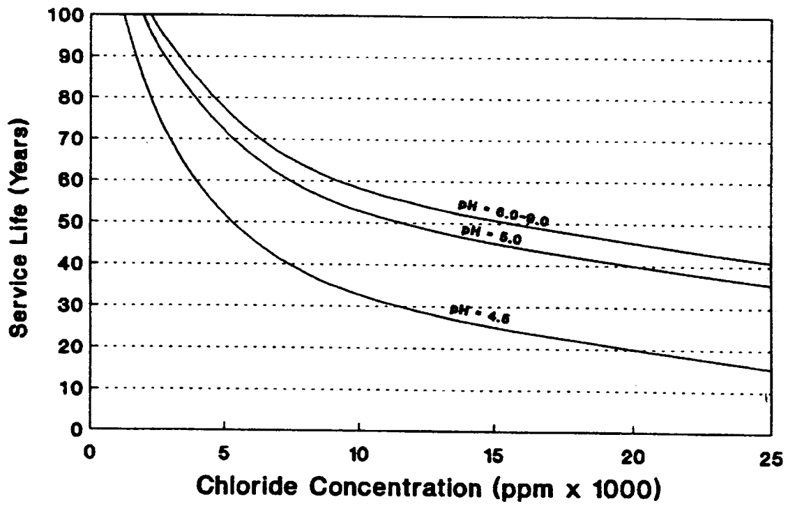
Figure 32. Estimated Service Life vs. pH and Chlorides for 36" DIA Concrete Culverts, S=1500 ppm
