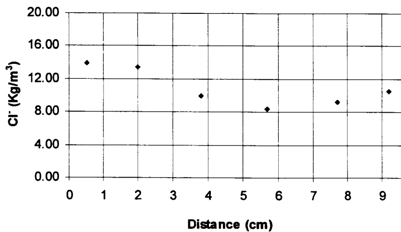
Chloride content vs distance from inside surface
