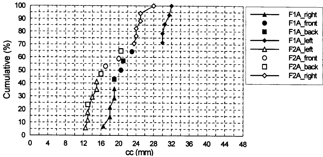
Figure 4. Distribution of concrete cover with cc values for cross sections of longitudinal and transversal wires plotted separately. Data for all six specimens of a) set A and b) set B.
