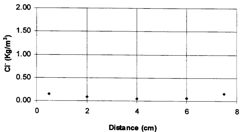
Chloride content vs distance from inside surface
