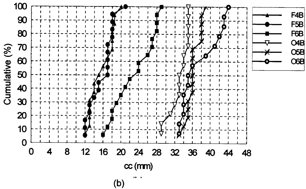
Figure 3. Cumulative percentage of steel wire cross sections examined in the cut edges vs concrete cover thickness (cc) for specimens corresponding to : a) set A and b) set B.
